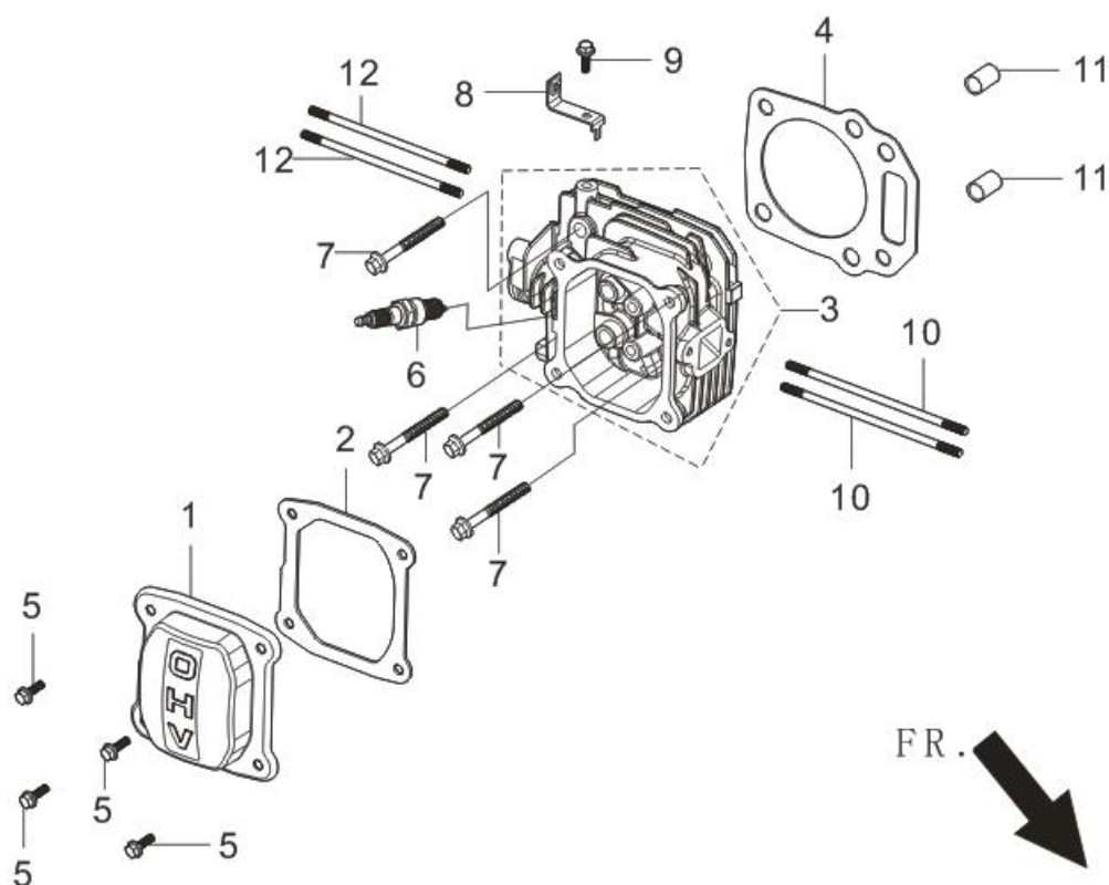
FIG.1 HEAD SUBASSEMBLY, CYLINDER / PLUG,SPARK (E01)
