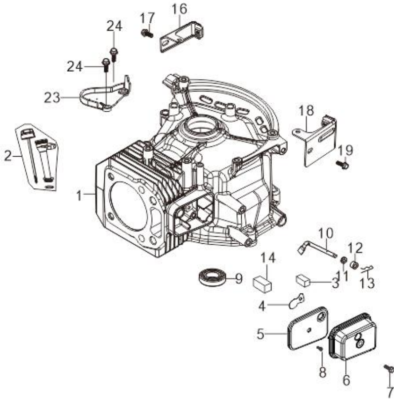
FIG.2 CRANKCASE.(E02)
