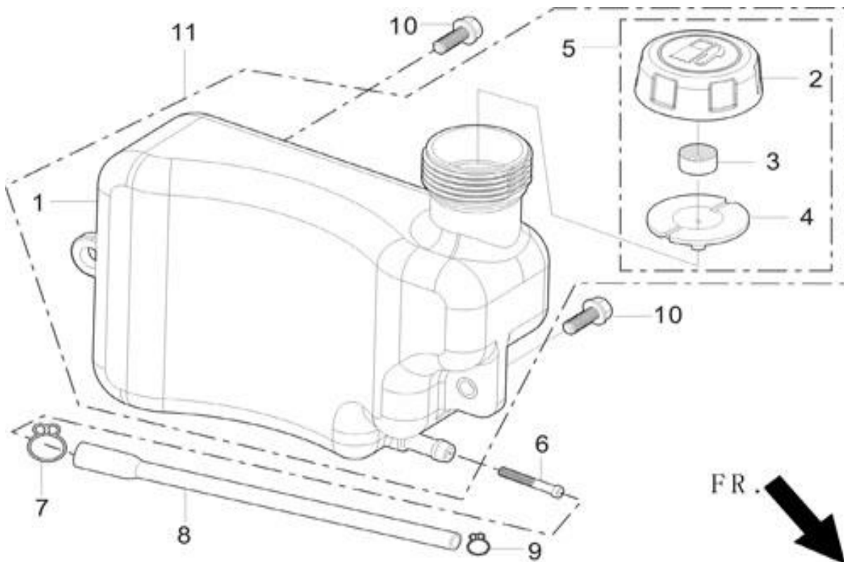
FIG.11 TANK, FUEL (E11)
