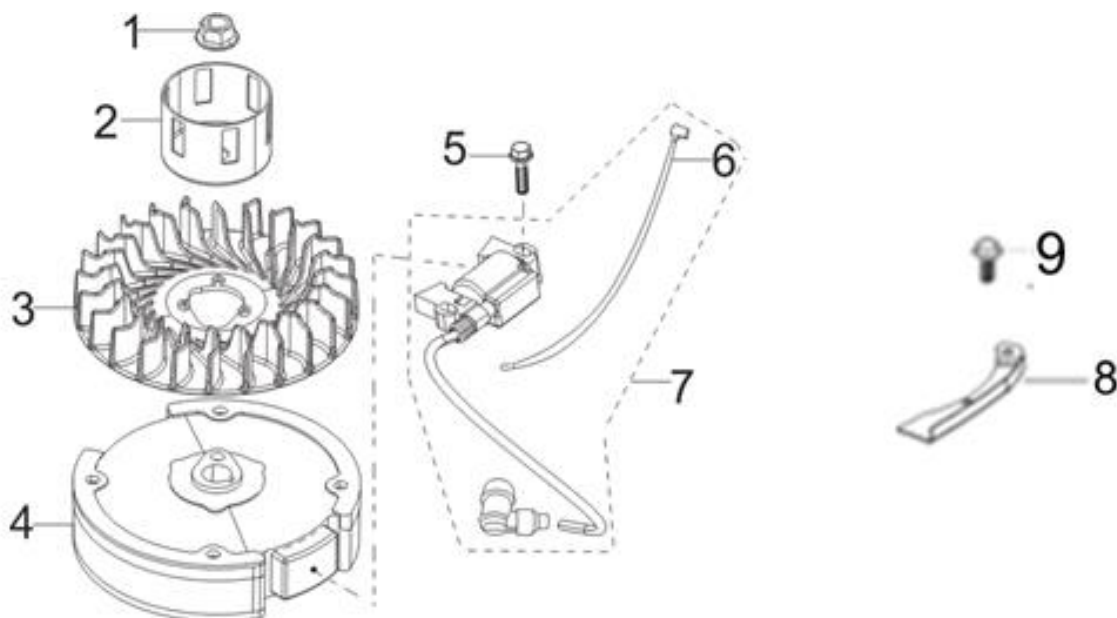
FIG.12 FLYWHEEL / IMPELLER / STARTER PULLEY / IGNITION COIL (E12)
