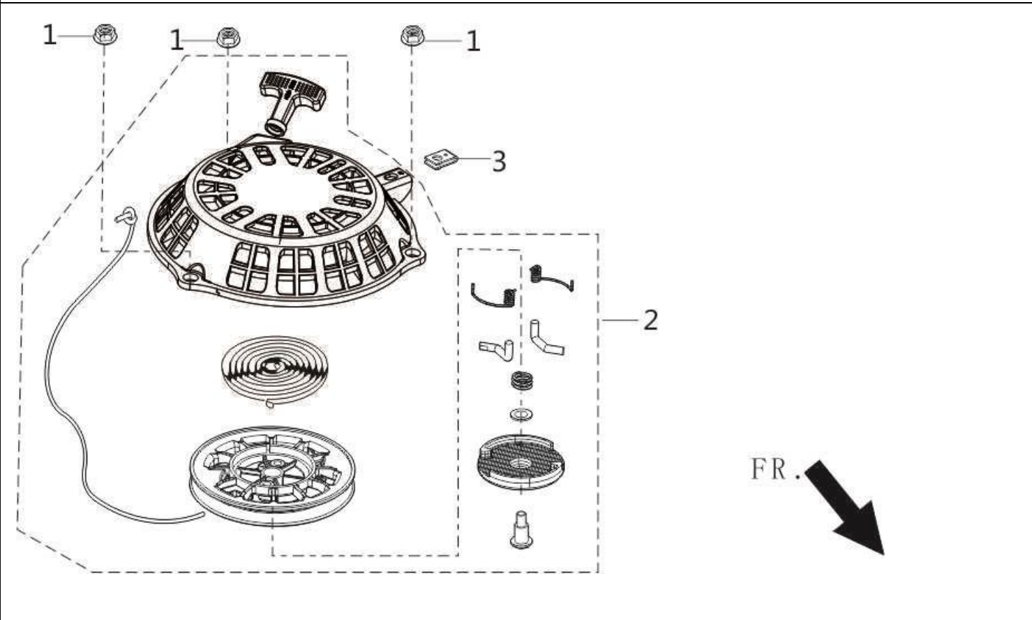
FIG.6 STARTER,RECOIL (E06)
