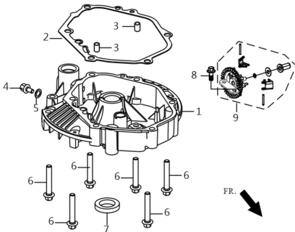
FIG.3 COVER SUBASSEMBLY, CRANKCASE / GEAR ASSY, GOVERNOR(E03)
