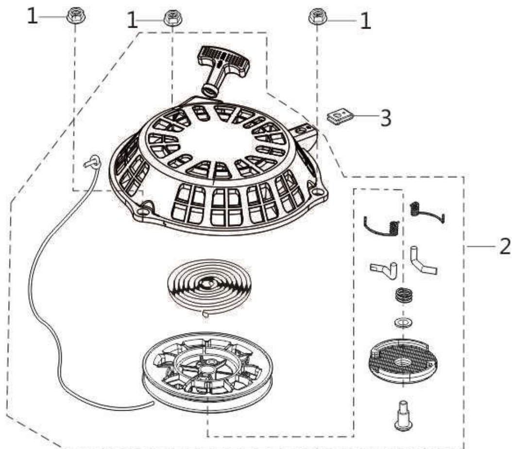
FIG.6 STARTER,RECOIL (E06)
