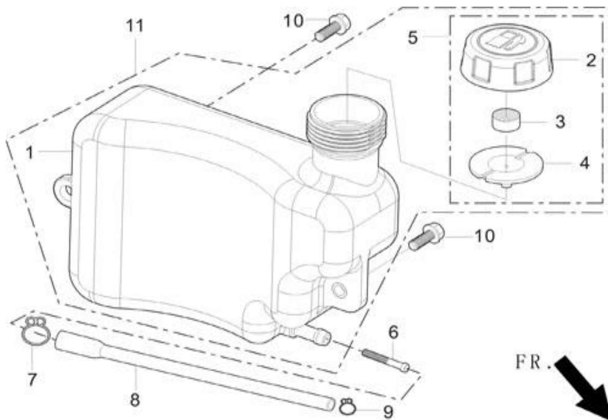
FIG.11 TANK, FUEL (E11)
