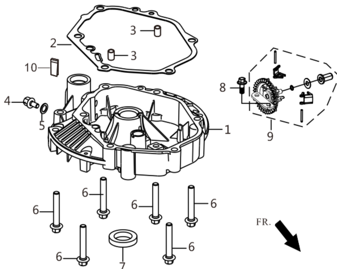
FIG.3 COVER SUBASSEMBLY, CRANKCASE / GEAR ASSY, GOVERNOR (E03)
