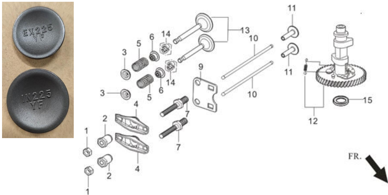
FIG.5 TRAIN,VALVE / CAMSHAFT SUBASSEMBLY (E05)
