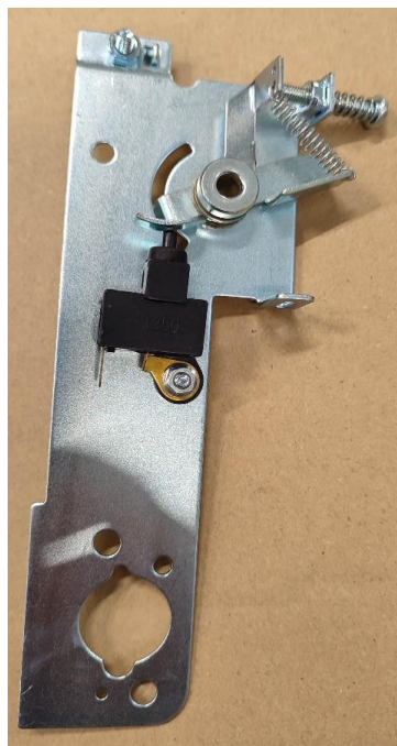
FIG.13 CONTROL ASSY, THROTTLE (E13)
