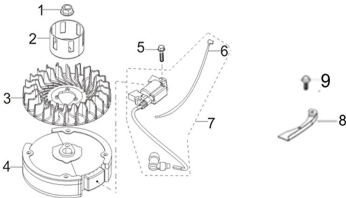
FIG.12 FLYWHEEL / IMPELLER / STARTER PULLEY / IGNITION COIL (E12)
