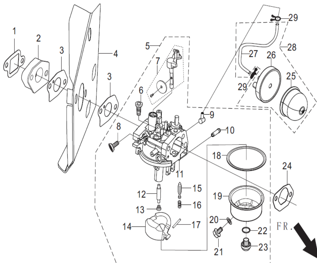
FIG.8 CARBURETOR ASSY. (E08)
