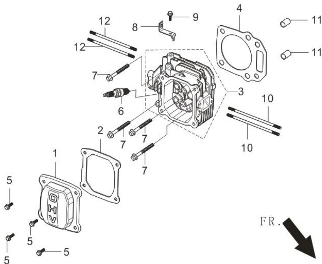
FIG.1 HEAD SUBASSEMBLY, CYLINDER / PLUG,SPARK (E01)
