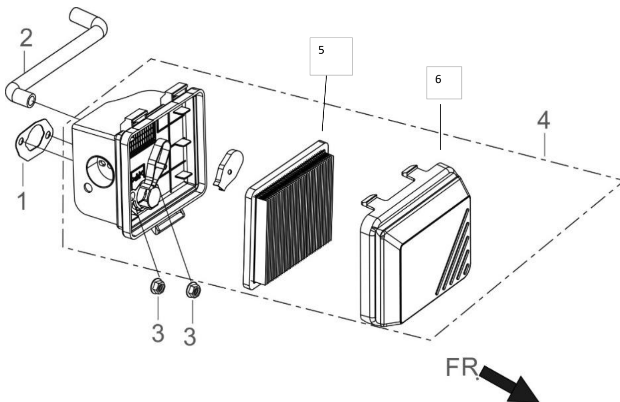
FIG.9 CLEANER, AIR (E09)
