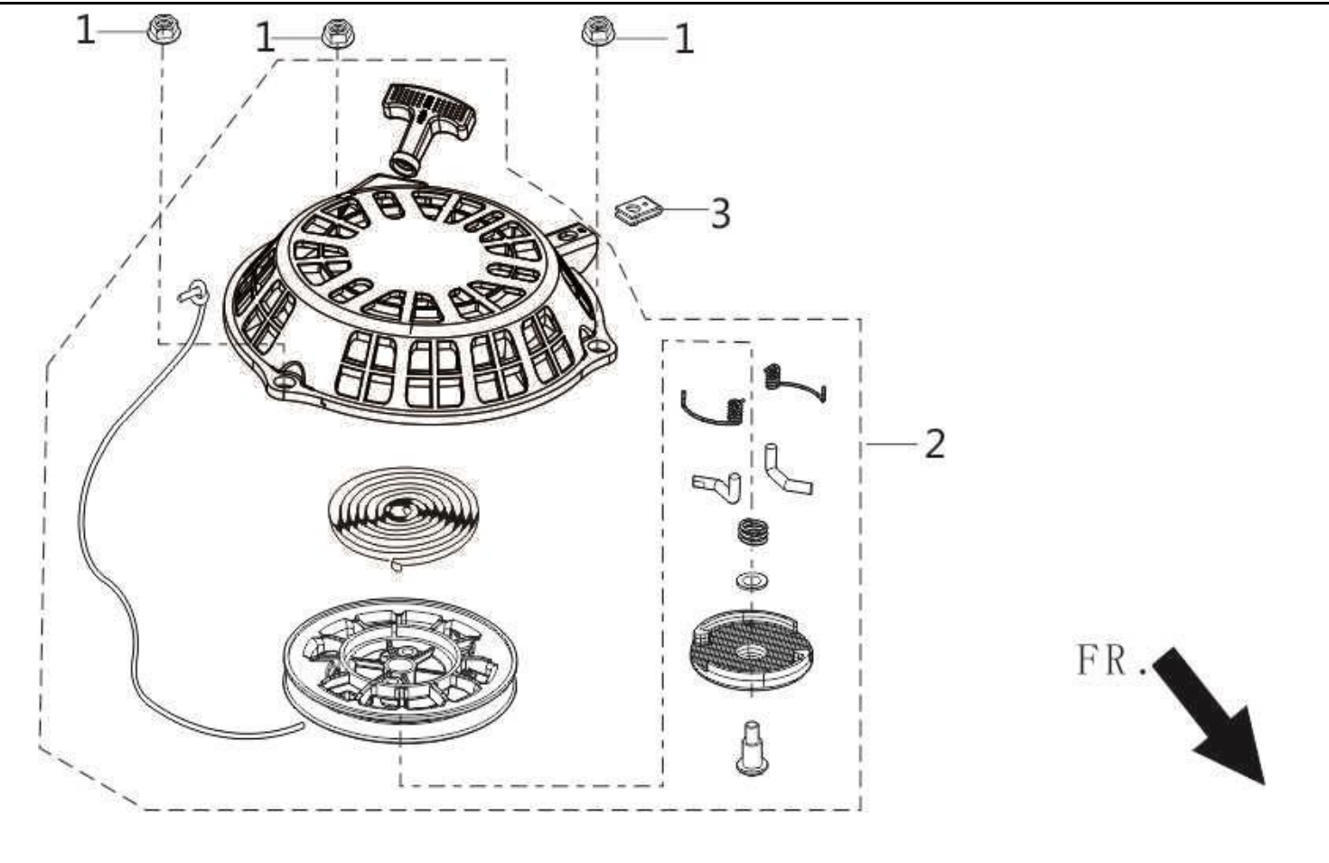
FIG.6 STARTER,RECOIL (E06)
