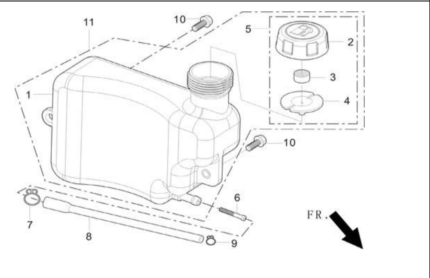
FIG.11 TANK, FUEL (E11)
