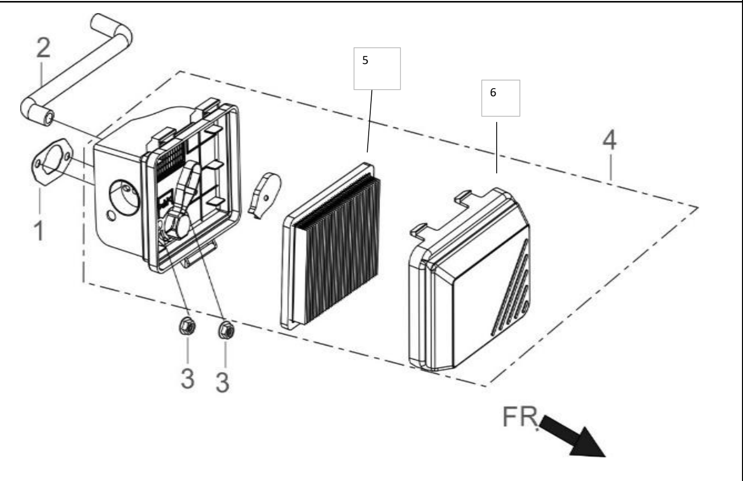
FIG.9 CLEANER, AIR (E09)
