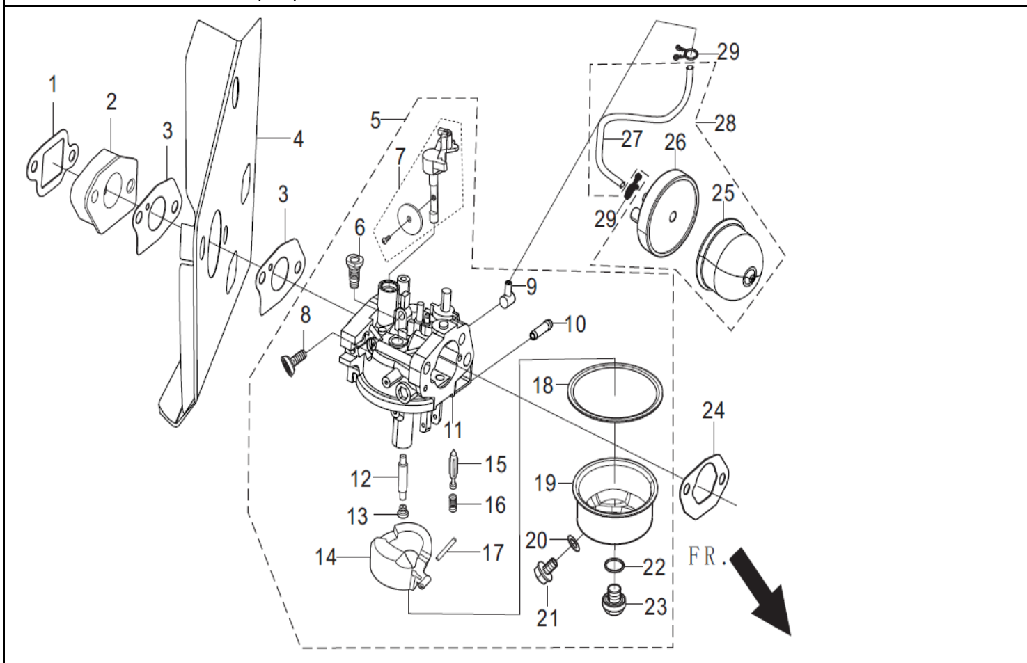
FIG.8 CARBURETOR ASSY. (E08)
