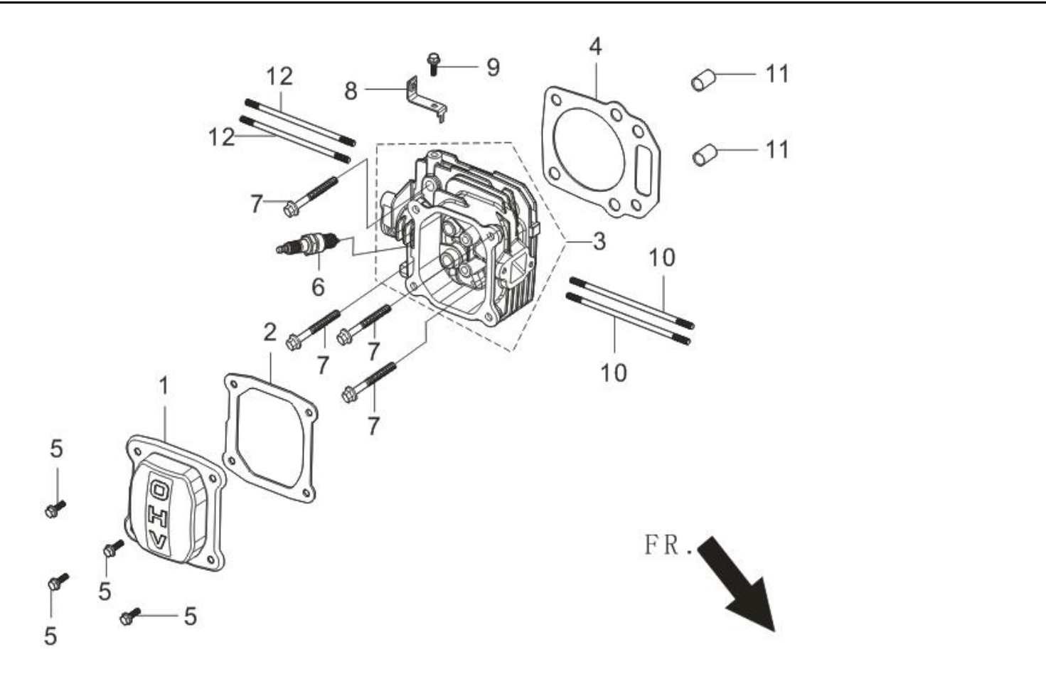
FIG.1 HEAD SUBASSEMBLY, CYLINDER / PLUG,SPARK (E01)
