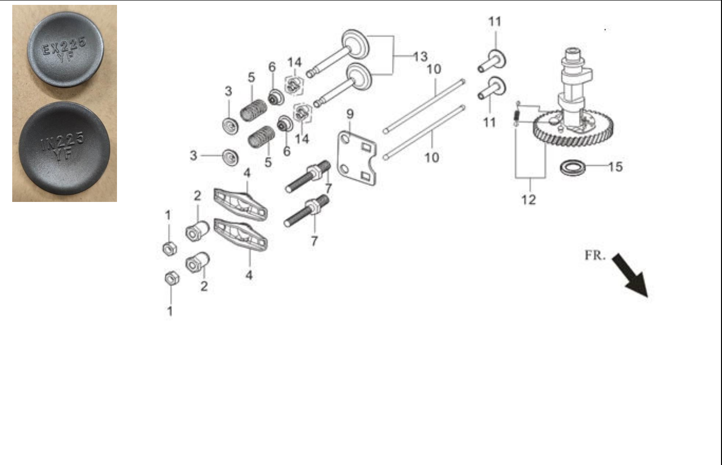
FIG.5 TRAIN,VALVE / CAMSHAFT SUBASSEMBLY (E05)
