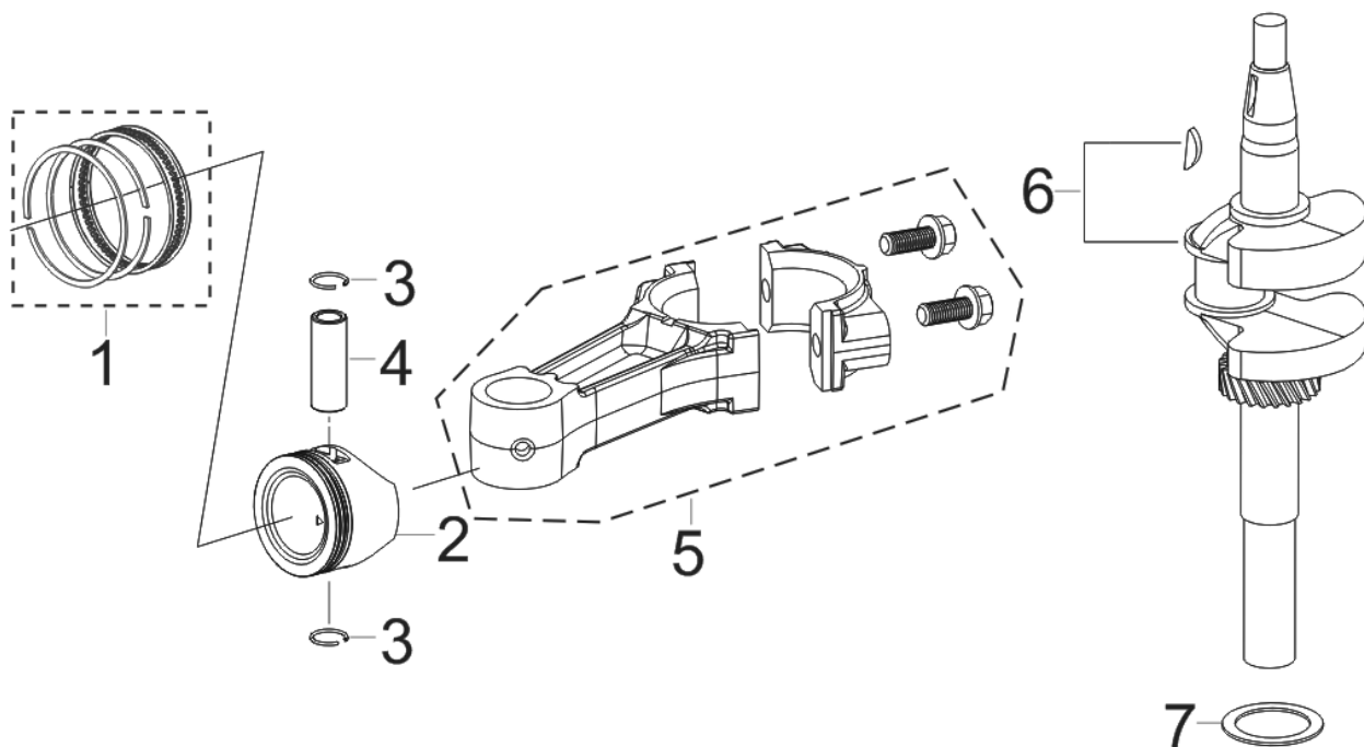
FIG.4 ROD,CRANKSHAFT CONNETING (E04)
