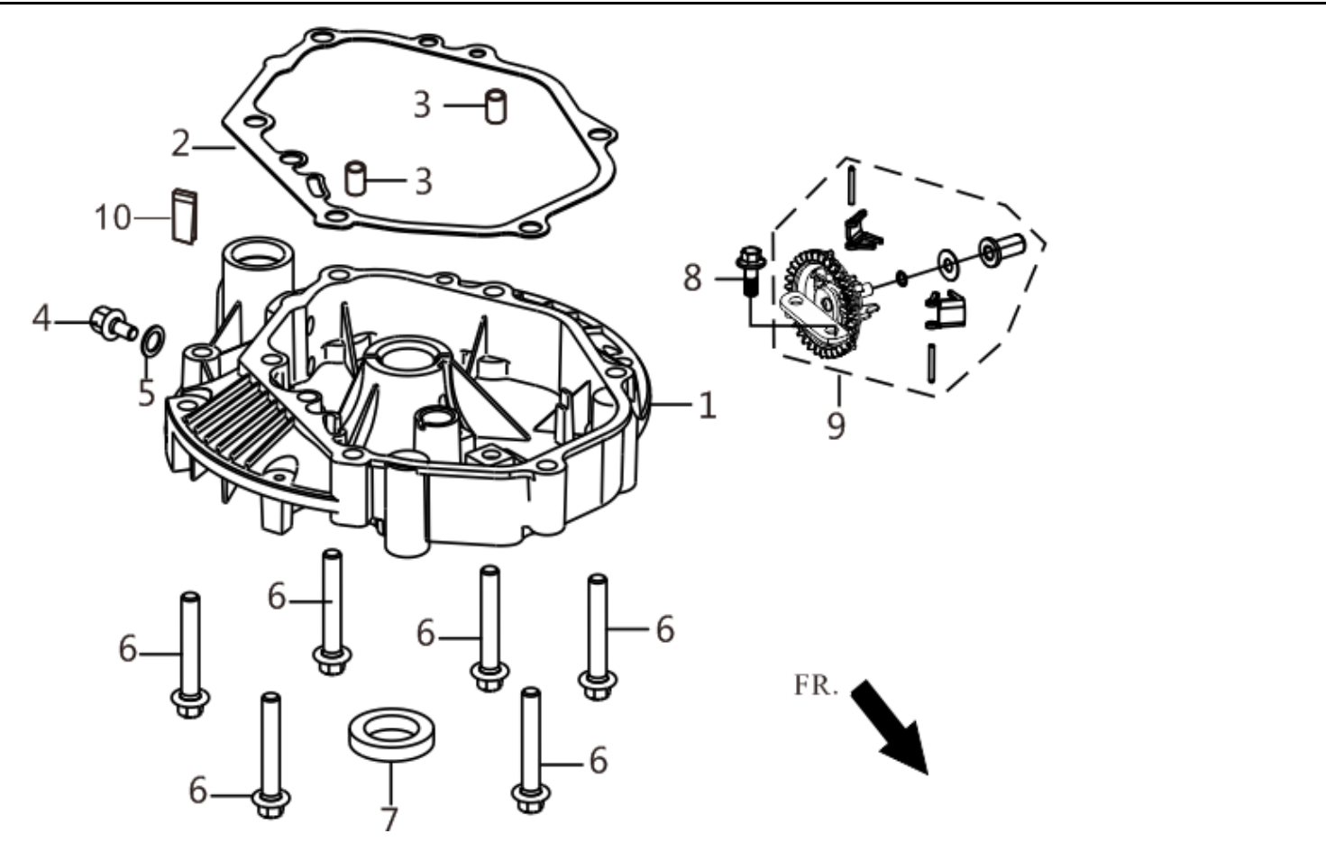
FIG.3 COVER SUBASSEMBLY, CRANKCASE / GEAR ASSY, GOVERNOR (E03)
