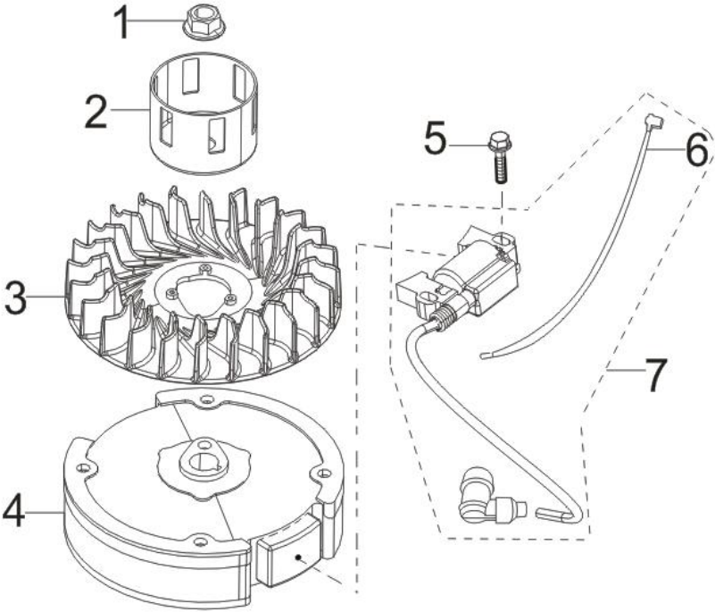
FIG.12 FLYWHEEL / IMPELLER / STARTER PULLEY / IGNITION COIL (E12)
