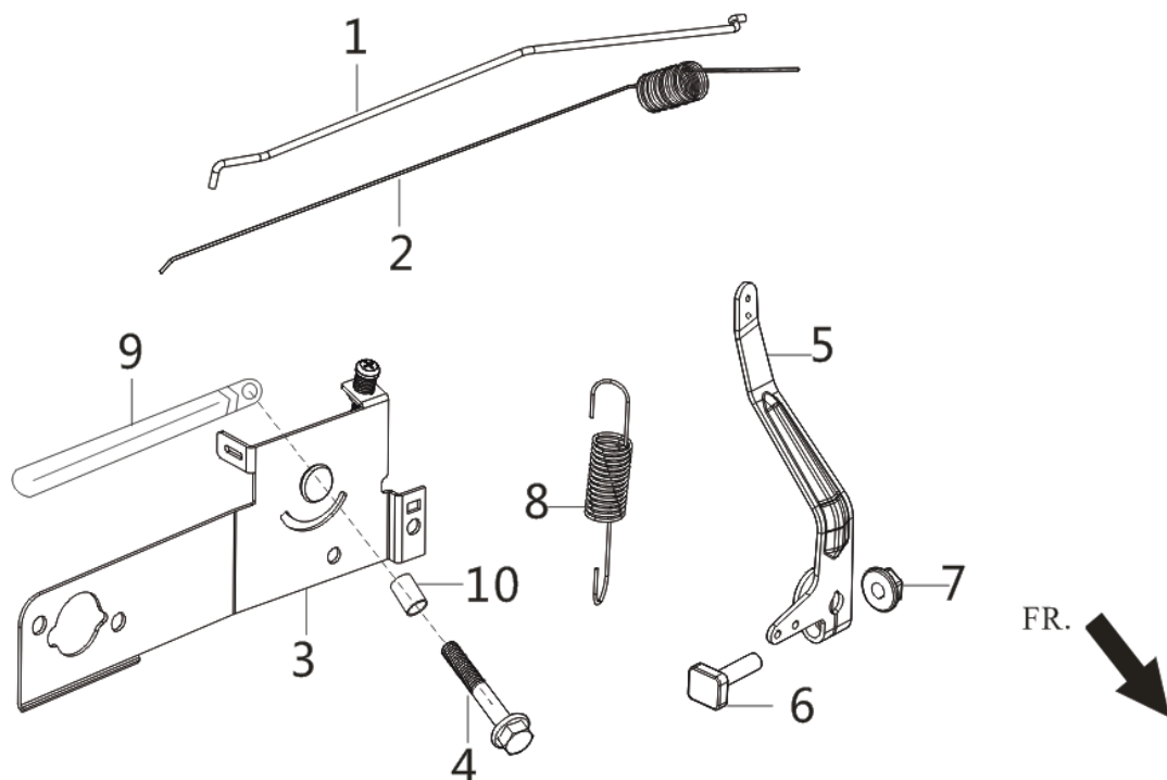
FIG.13 CONTROL ASSY, THROTTLE (E13)
