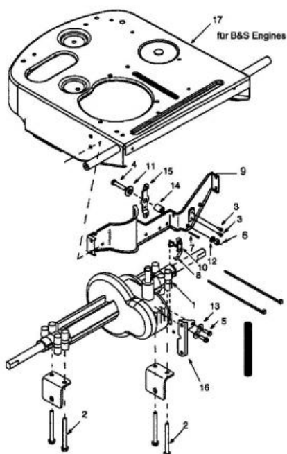
Hinterachse Transaxle Assembly
