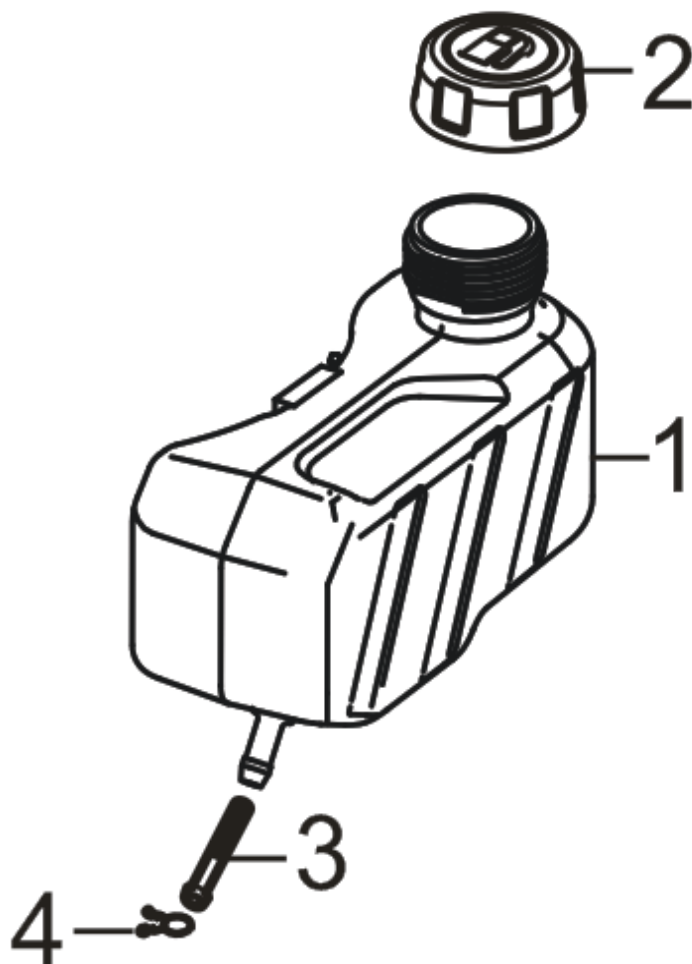
FIG.10 TANK ASSY, FUEL
