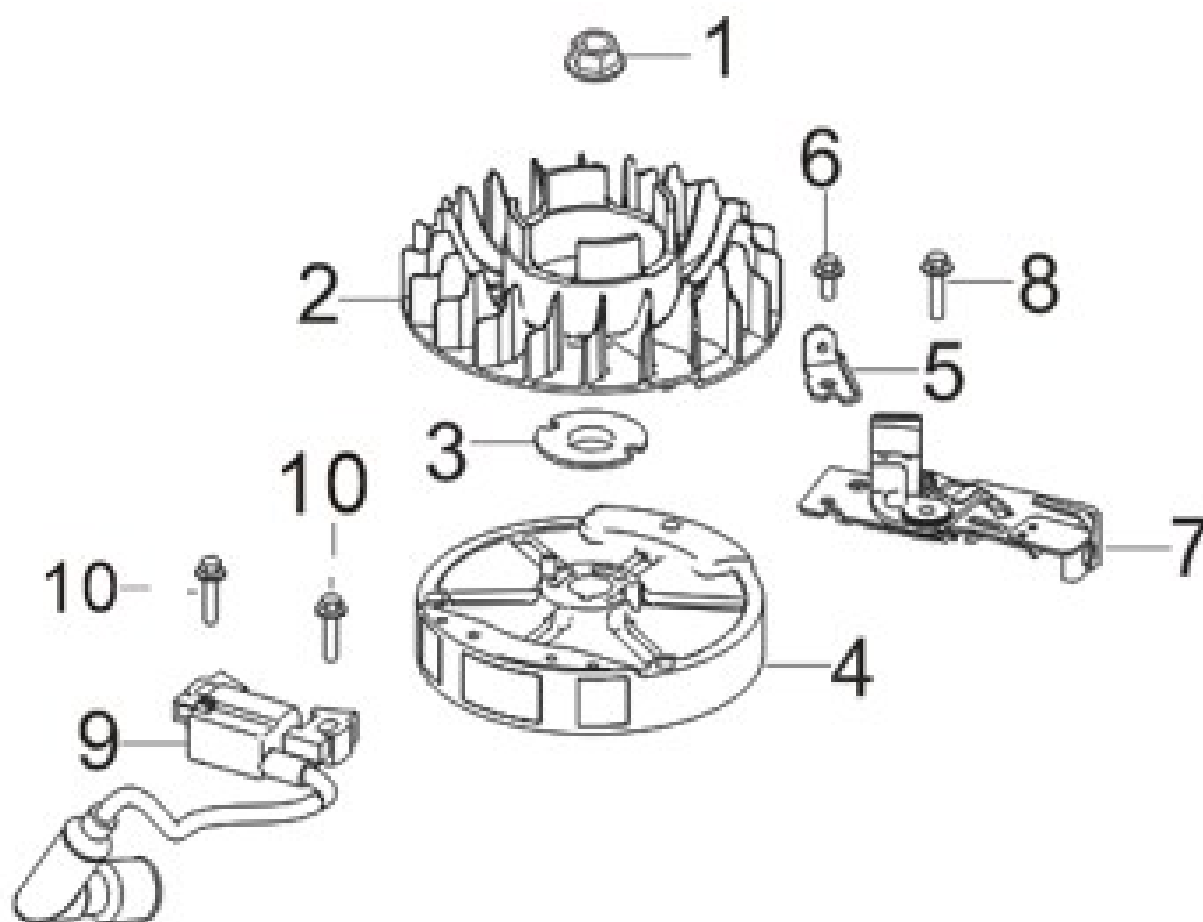
FIG.7 FLYWHEEL / IMPELLER / STARTER PULLEY / IGNITION COIL (E07)
