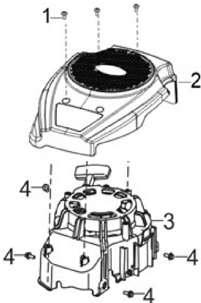
FIG.5 STARTER,RECOIL (E05)
