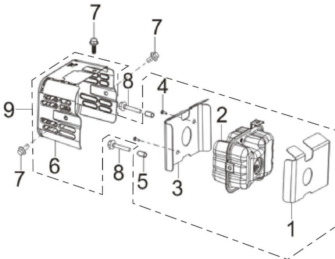
FIG.19 MUFFLER ASSY.
