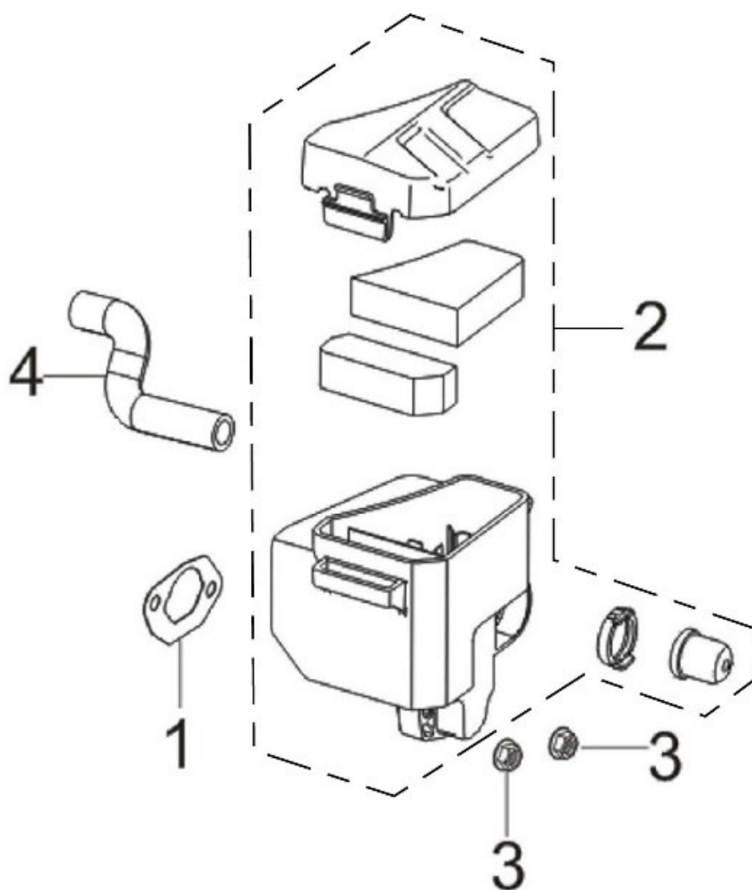
FIG.8 CLEANER, AIR (F01)
