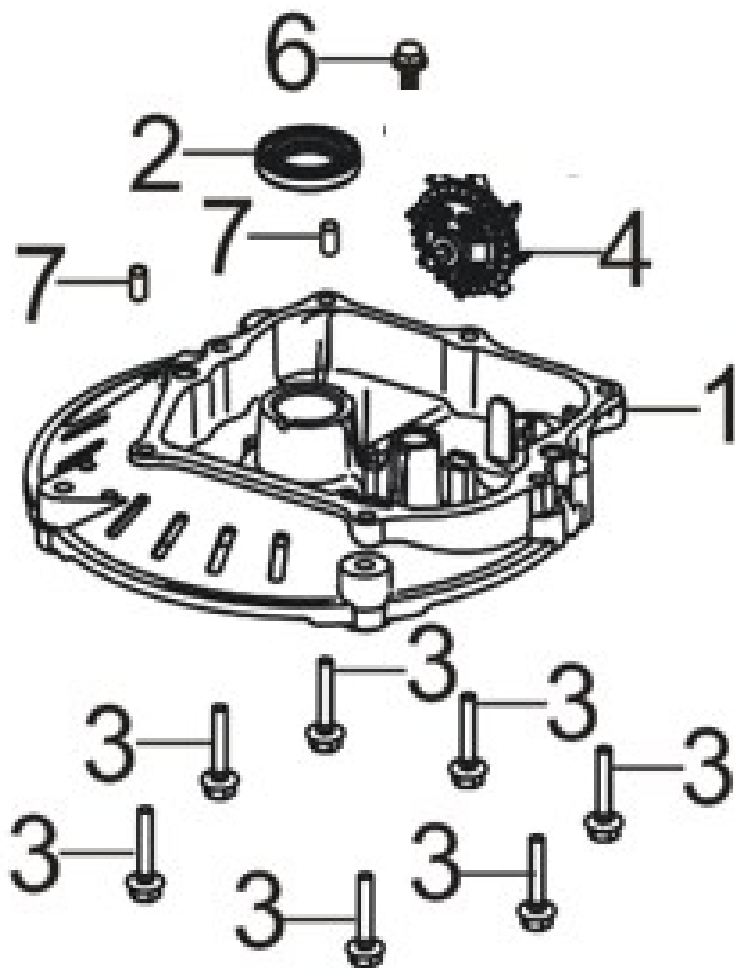
FIG.2 COVER SUBASSEMBLY, CRANKCASE
