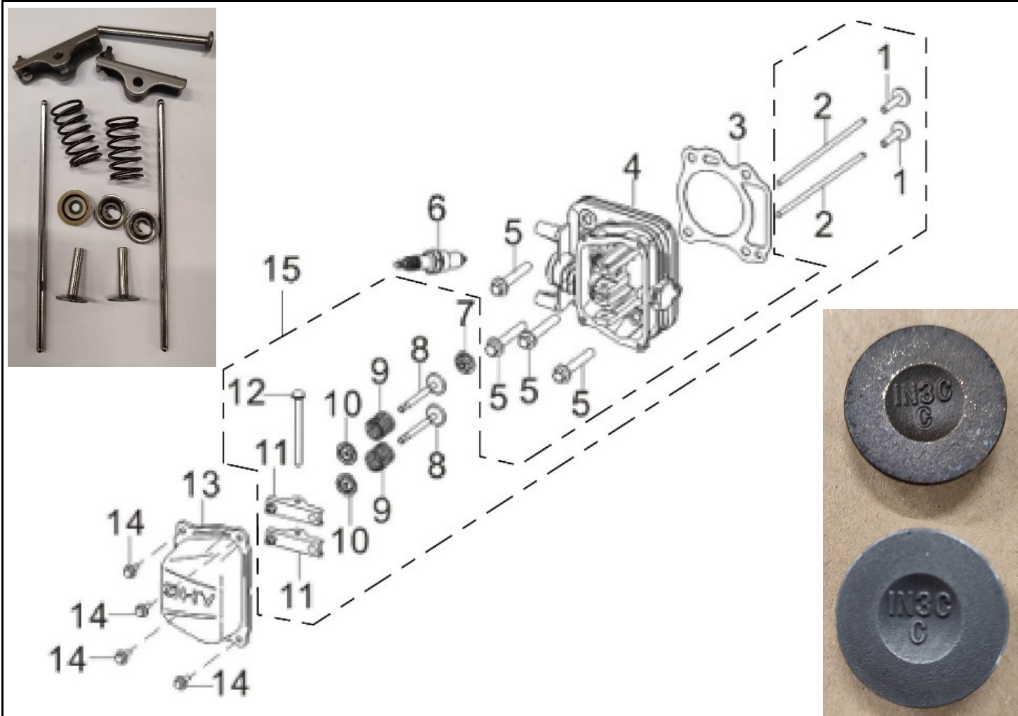
FIG.3 HEAD SUBASSEMBLY, CYLINDER / PLUG,SPARK
