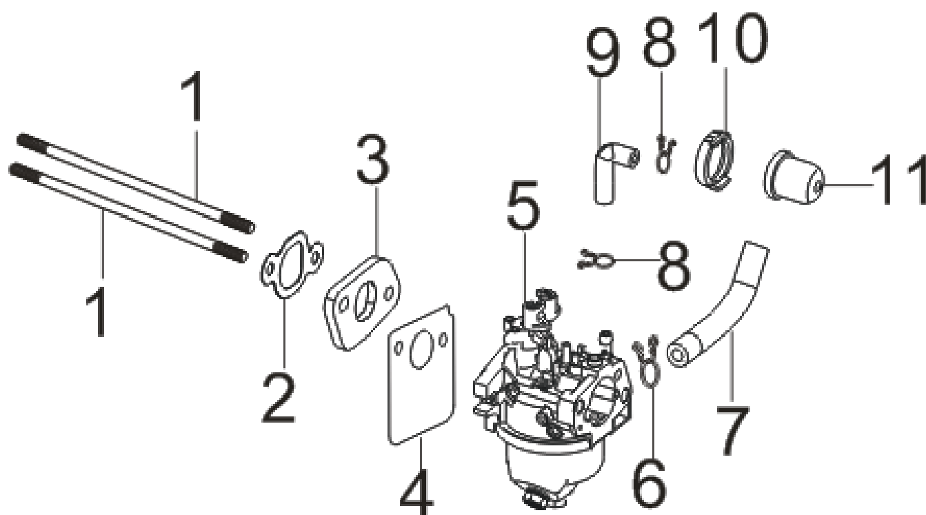
FIG.6 CARBURETOR ASSY. (E06)
