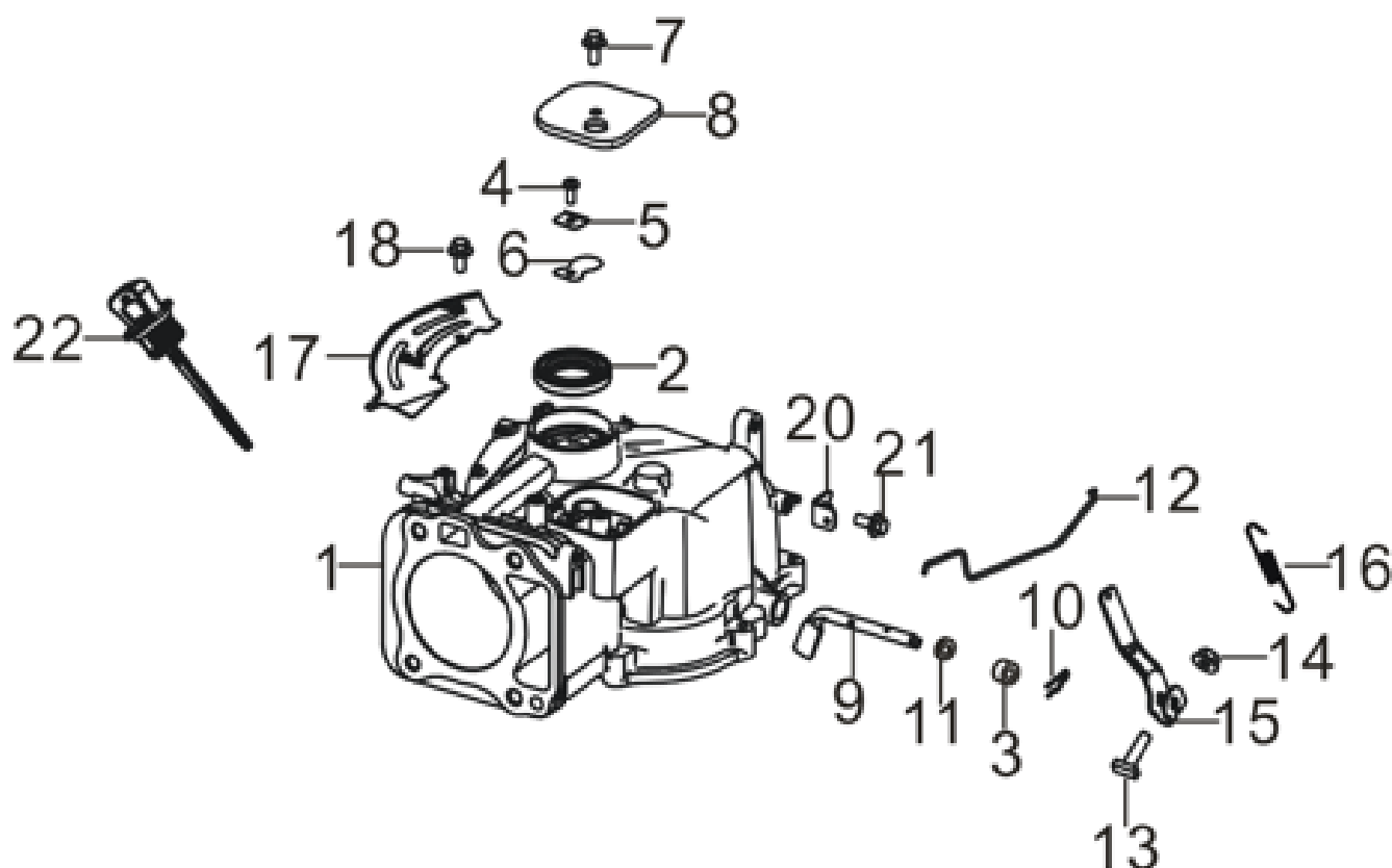
FIG.1 CRANKCASE. / GEAR ASSY, GOVERNOR.
