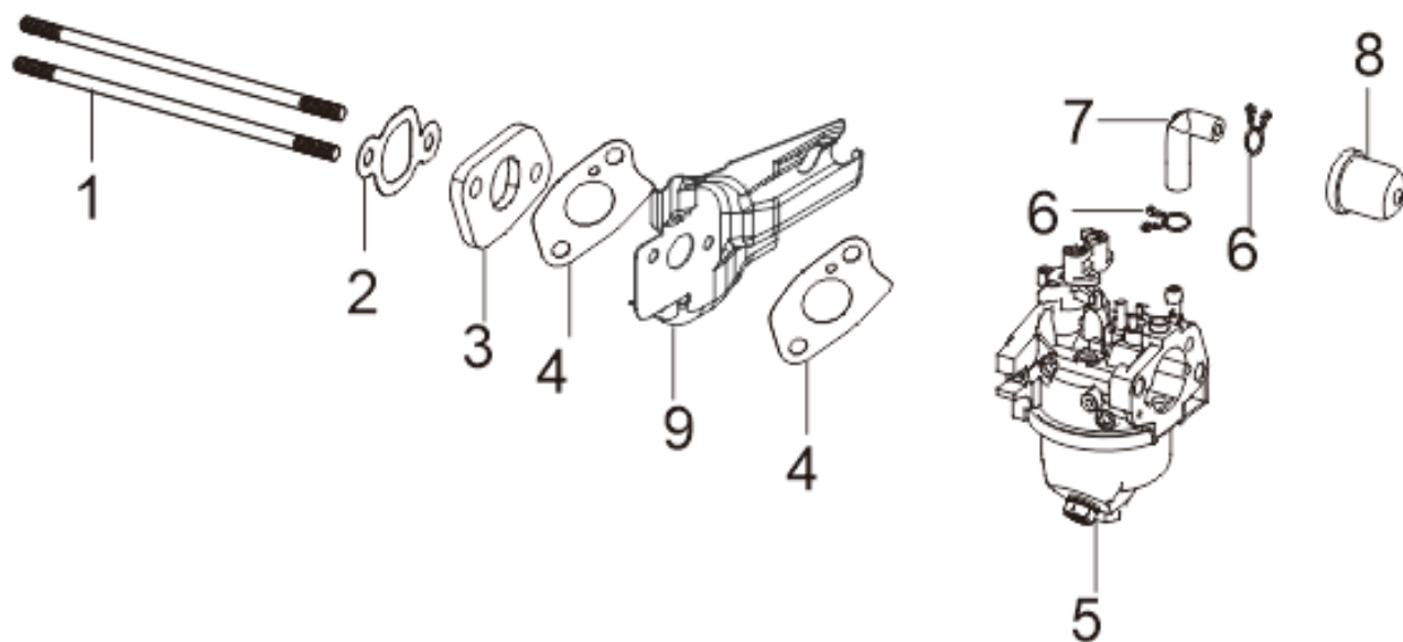
FIG.6 CARBURETOR ASSY. ( E06 )
