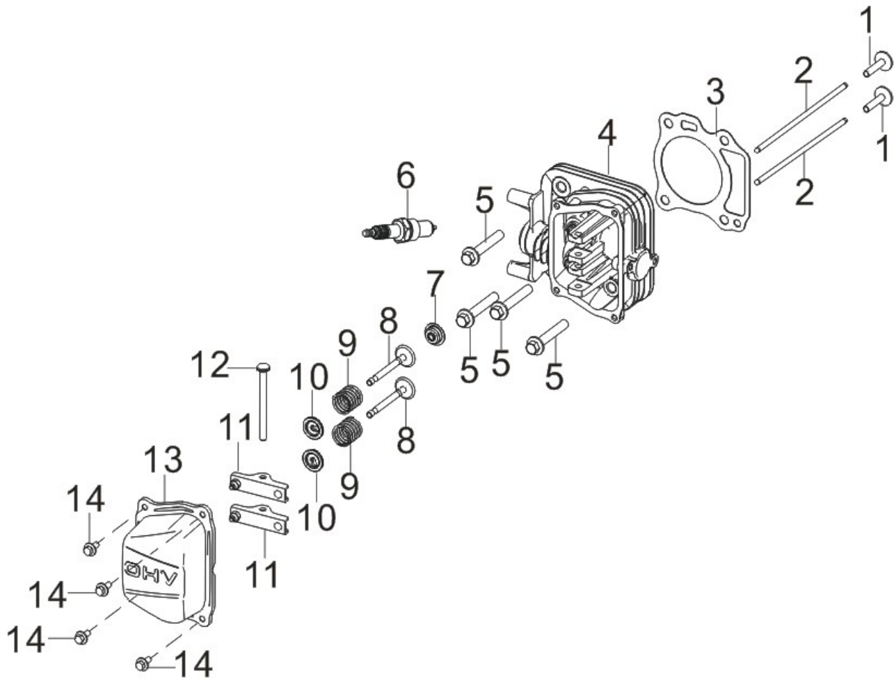
FIG.3 HEAD SUBASSEMBLY, CYLINDER / PLUG,SPARK ( E03 )
