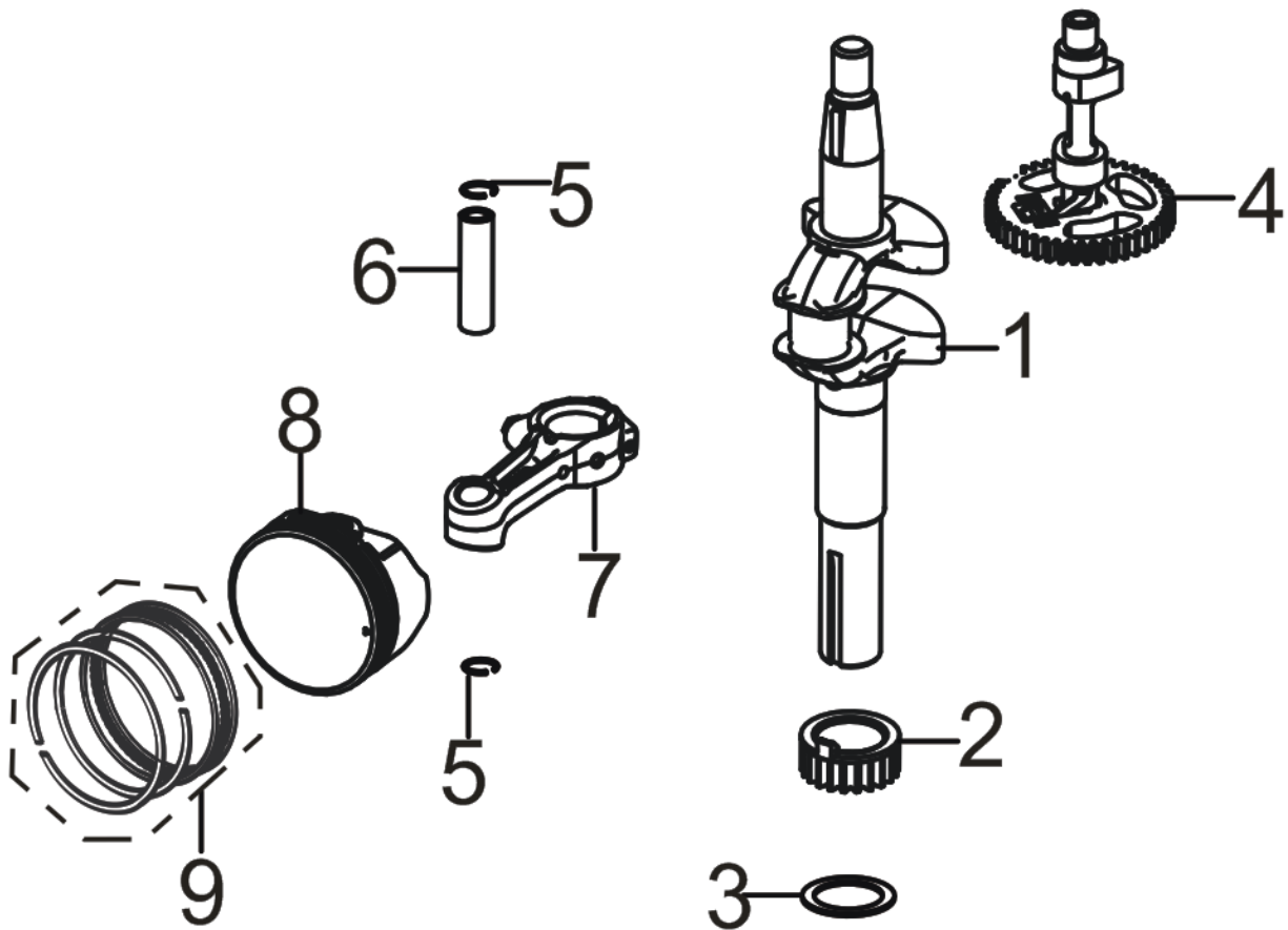
FIG.4 ROD,CRANKSHAFT CONNETING ( E04 )
