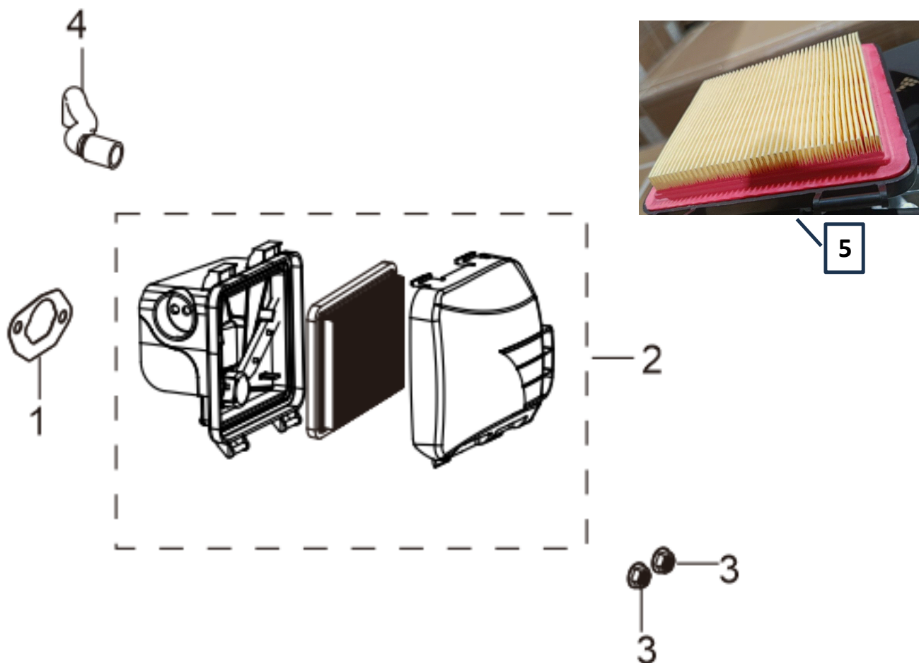
FIG.8 CLEANER, AIR ( F01 )
