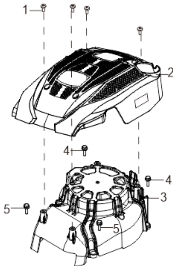
FIG.5 STARTER,RECOIL ( E05 )
