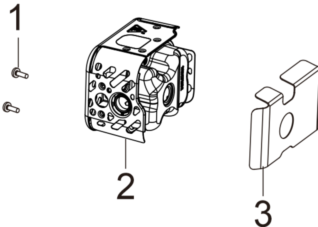
FIG.13 MUFFLER ASSY. ( F02 )
