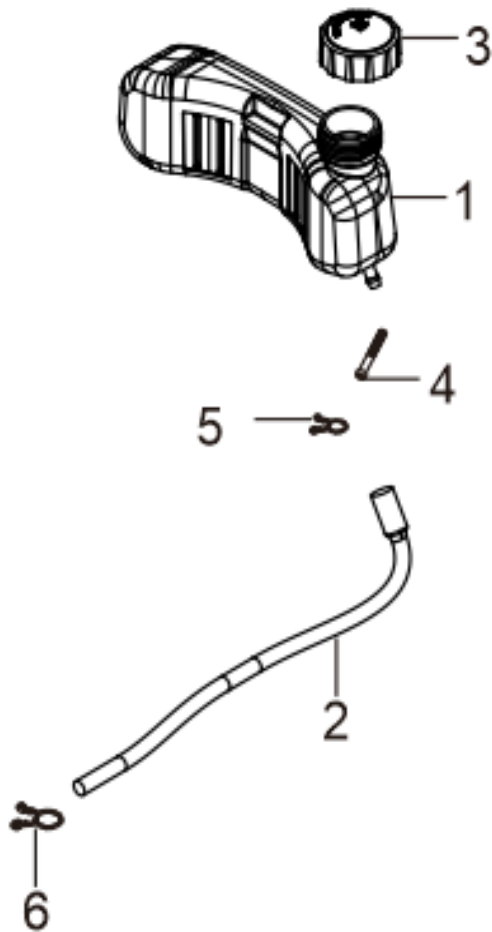
FIG.14 TANK ASSY, FUEL ( F03 )
