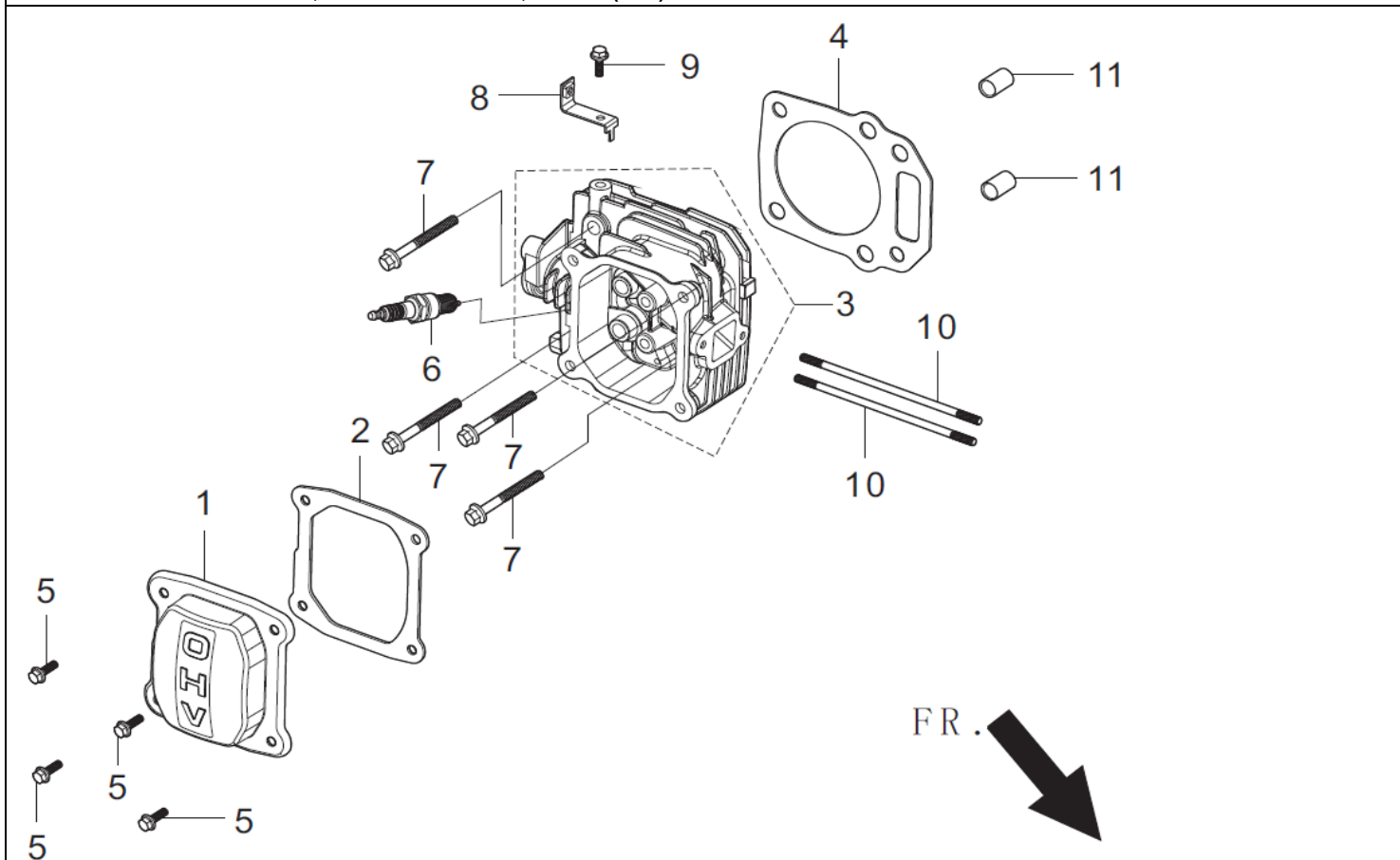
FIG.3 HEAD SUBASSEMBLY, CYLINDER / PLUG,SPARK (E03)
