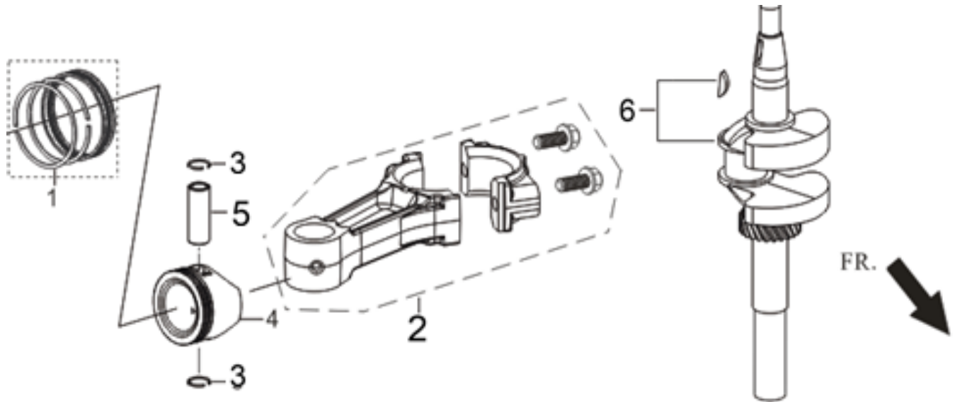
FIG.4 ROD,CRANKSHAFT CONNETING (E04)
