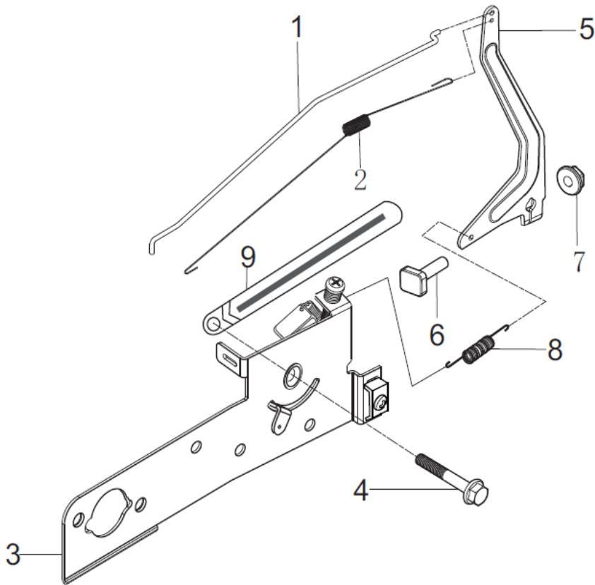
FIG.10 CONTROL ASSY, THROTTLE (E10)
