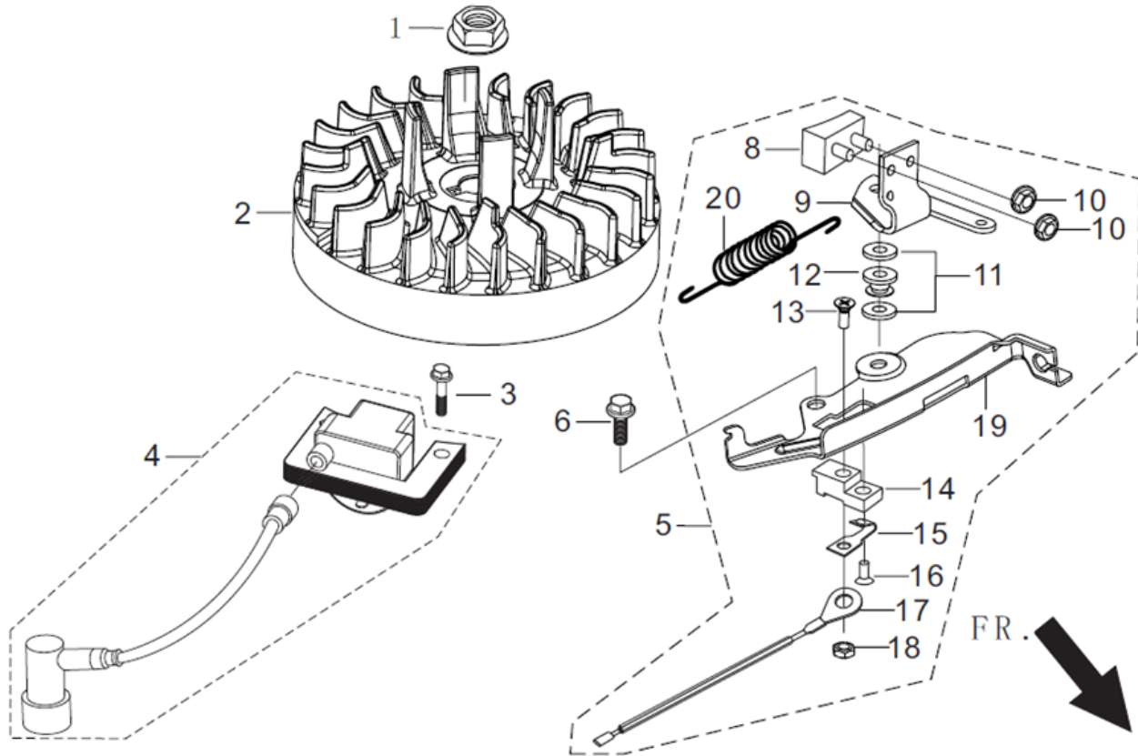
FIG.9 FLYWHEEL / IMPELLER / STARTER PULLEY / IGNITION COIL (E09)
