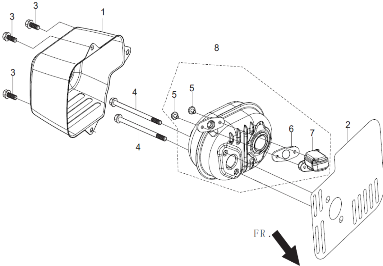
FIG.12 MUFFLER (F02)
