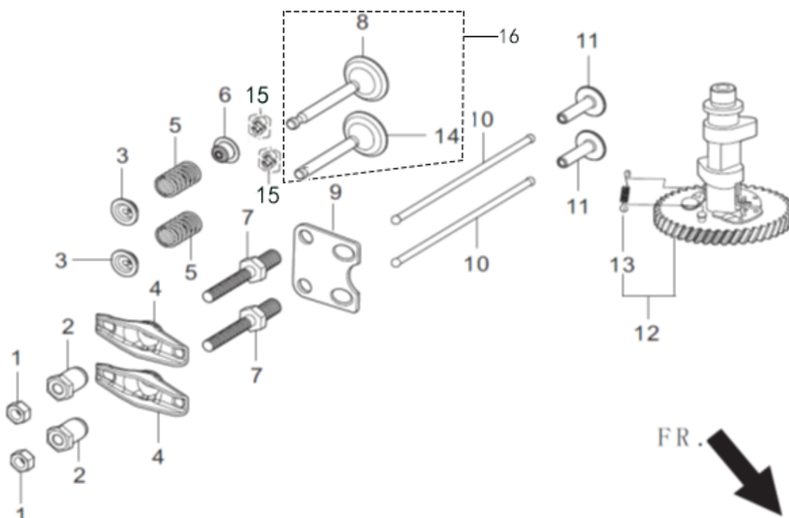
FIG.5 TRAIN,VALVE / CAMSHAFT SUBASSEMBLY (E05)
