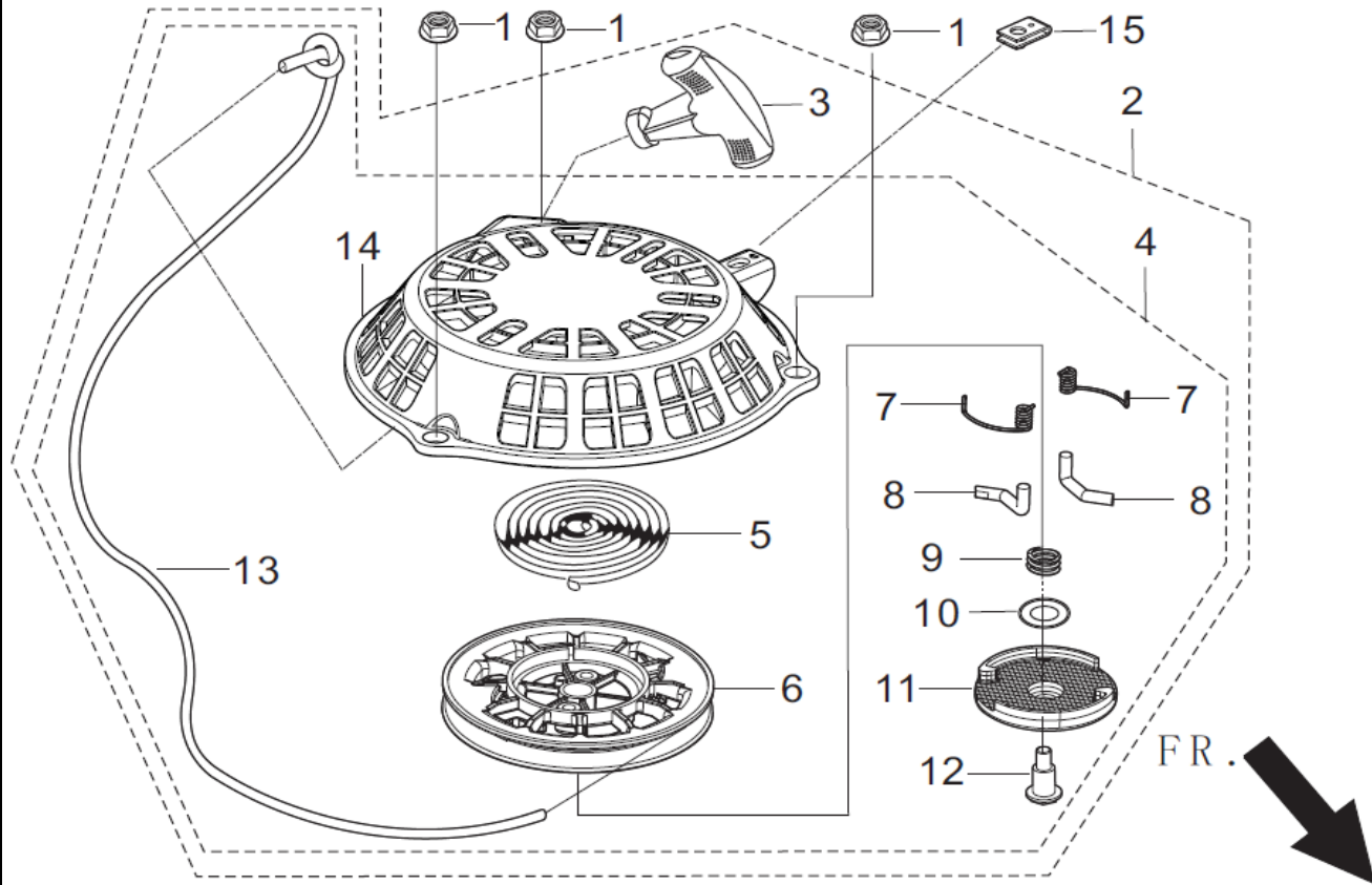
FIG.6 STARTER,RECOIL (E06)
