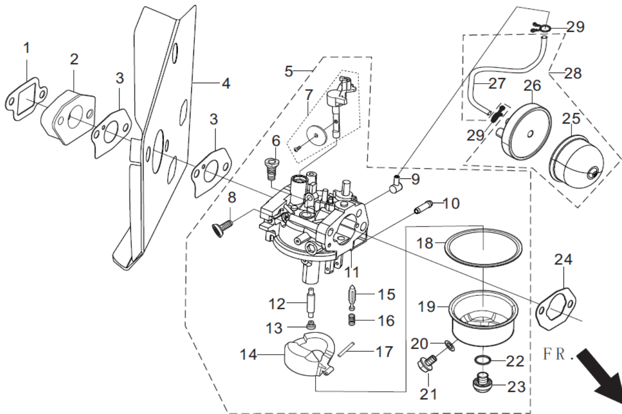
FIG.8 CARBURETOR ASSY. (E08)
