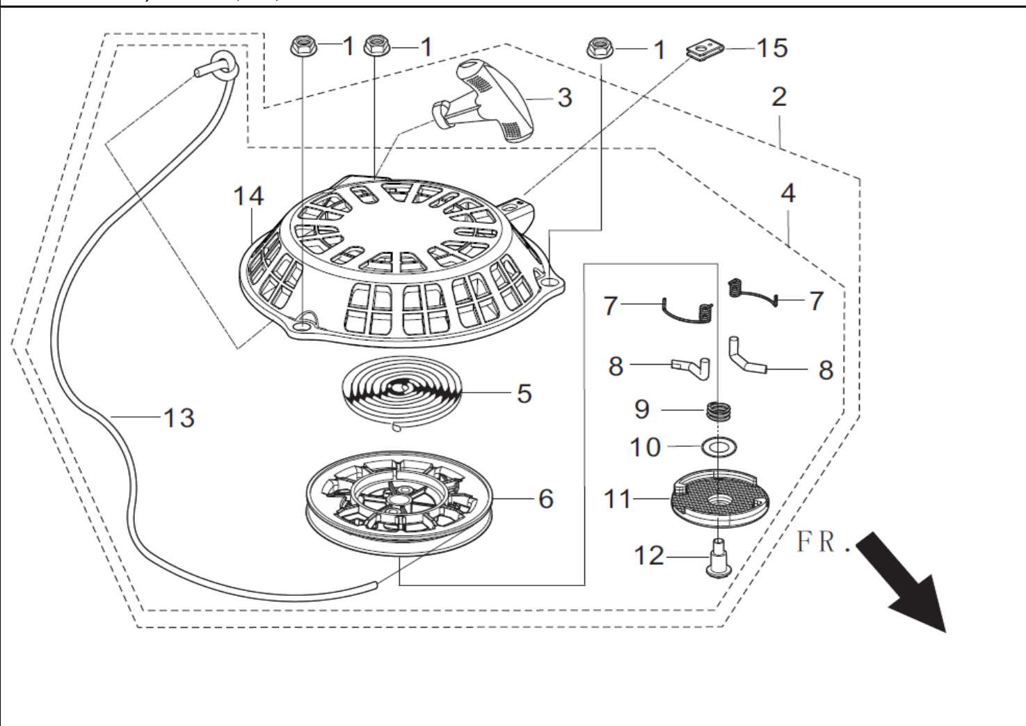
FIG.6 STARTER,RECOIL (E06)
