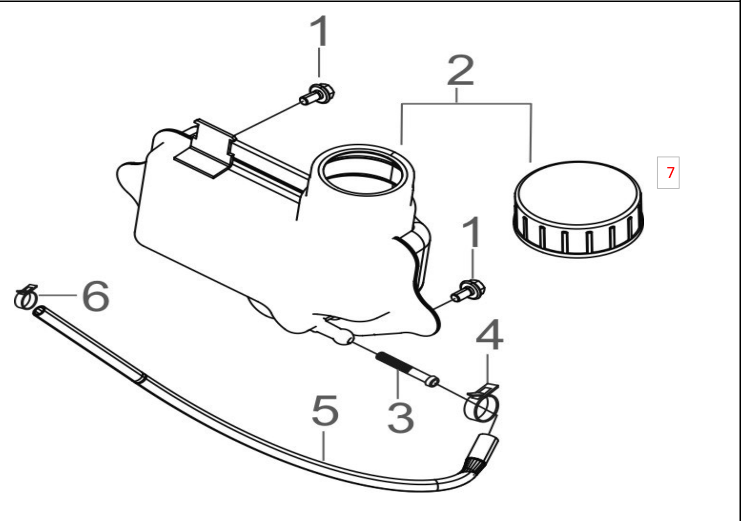
FIG.13 TANK, FUEL (F03)
