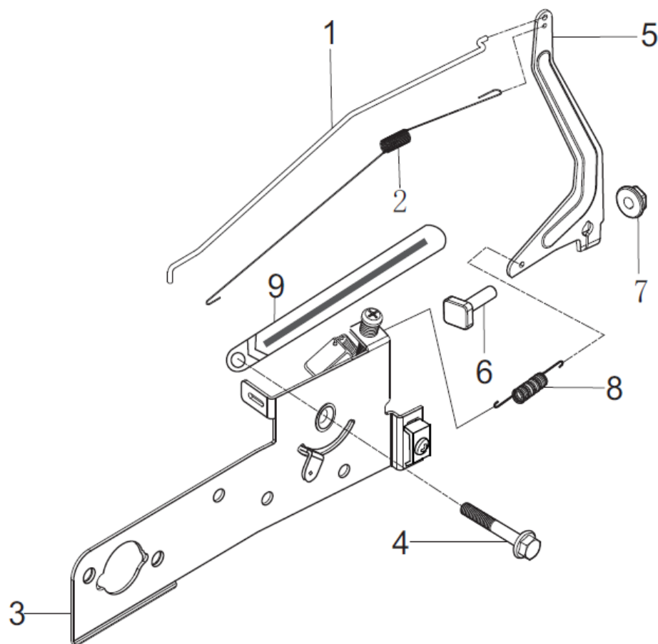
FIG.10 CONTROL ASSY, THROTTLE (E10)
