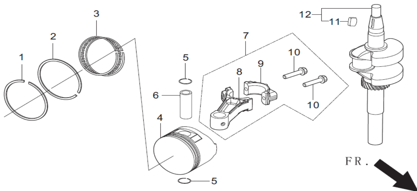
FIG.4 ROD,CRANKSHAFT CONNETING (E04)
