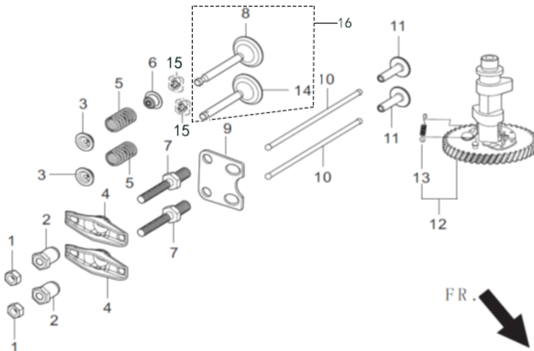
FIG.5 TRAIN,VALVE / CAMSHAFT SUBASSEMBLY (E05)
