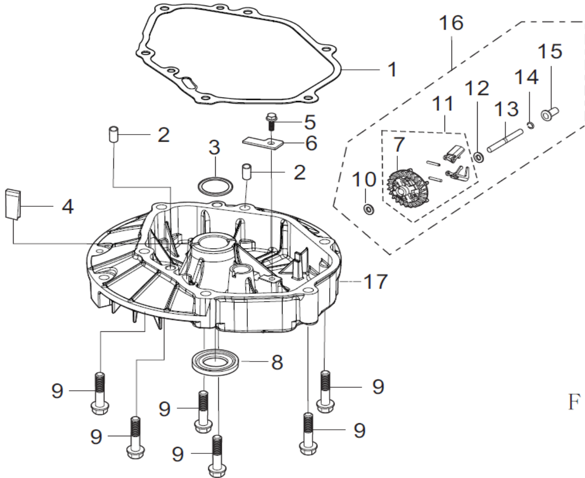
FIG.2 COVER SUBASSEMBLY, CRANKCASE / GEAR ASSY, GOVERNOR (E02)
