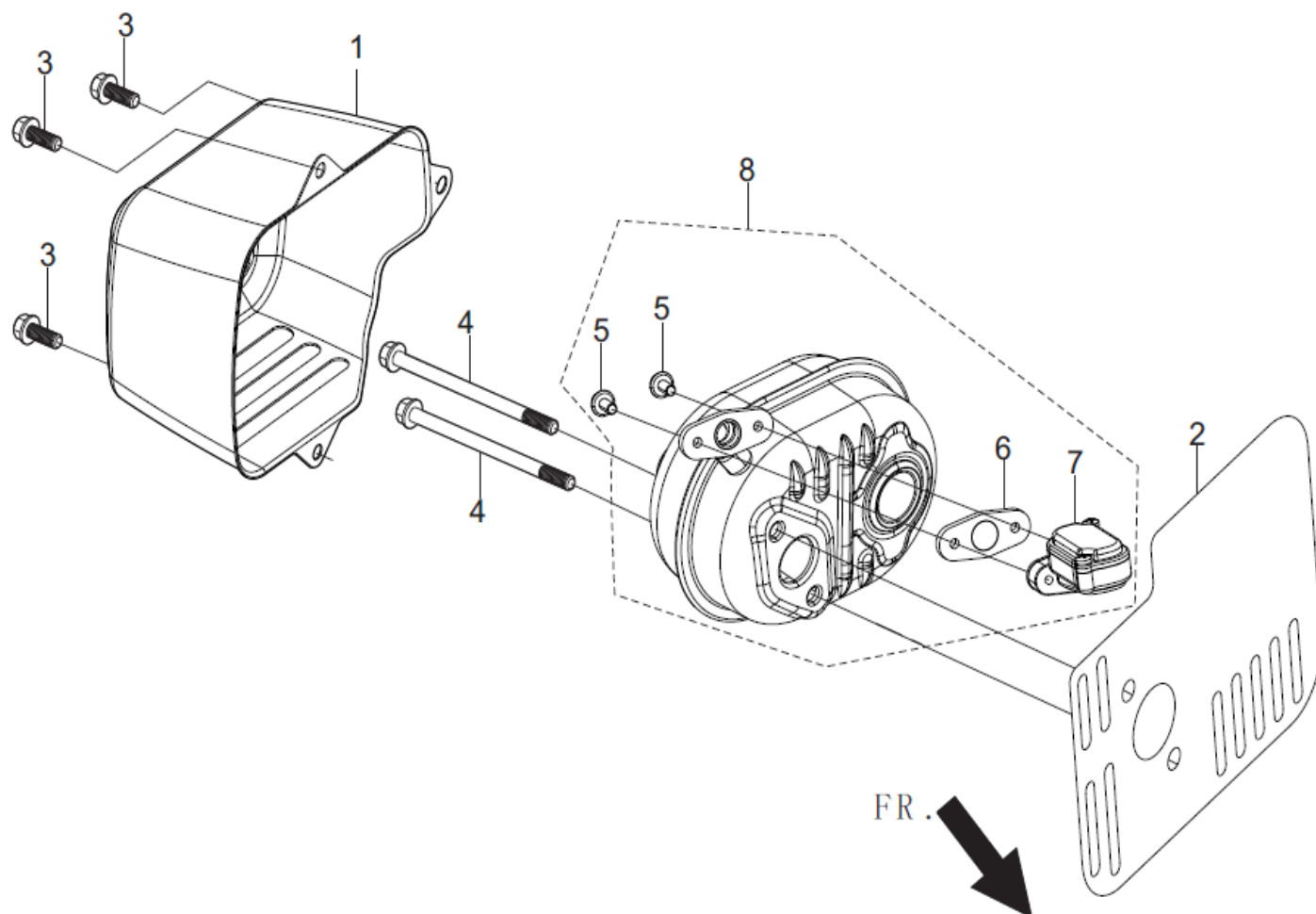
FIG.12 MUFFLER (F02)
