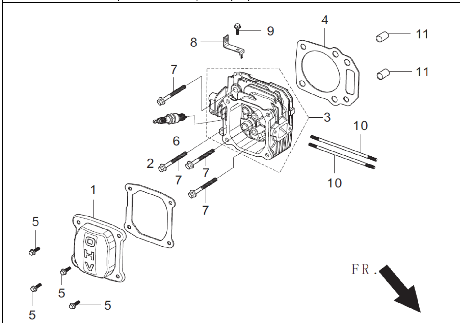
FIG.3 HEAD SUBASSEMBLY, CYLINDER / PLUG, SPARK (E03)
