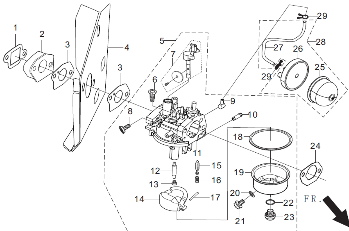
FIG.8 CARBURETOR ASSY. (E08)
