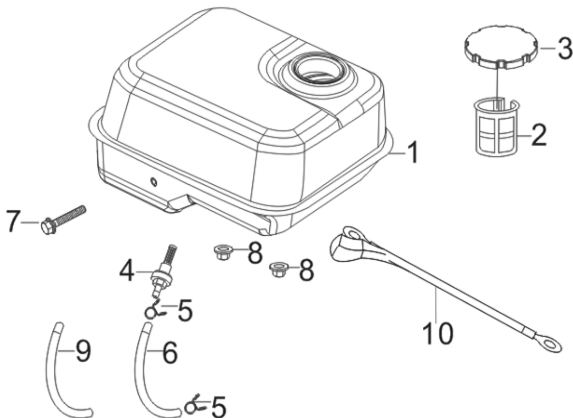
FIG.14 TANK ASSY, FUEL (F03)
