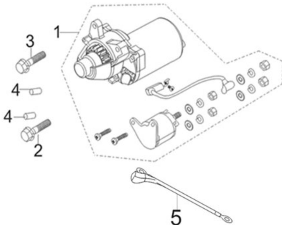
FIG.15 START-UP ELECTRIC MACHINE COMPONENTS (E12)
