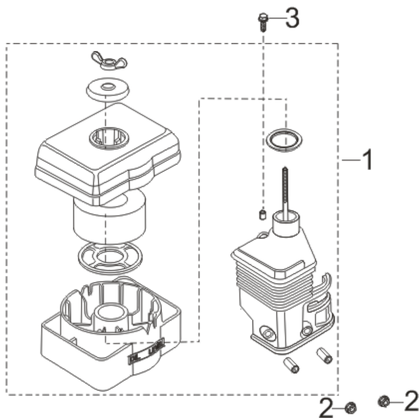
FIG.12 CLEANER, AIR (F01)
