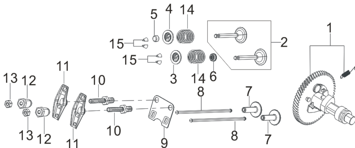
FIG.6 TRAIN,VALVE / CAMSHAFT SUBASSEMBLY (E06)
