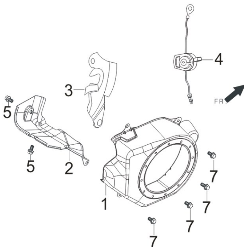
FIG.8 SHROUD / SHIELD,LOWER (E08)
