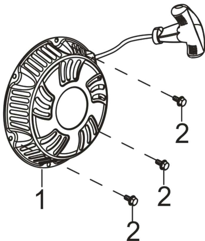
FIG.7 STARTER,RECOIL (E07)
