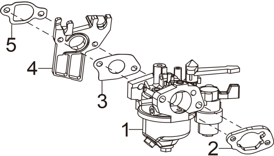
FIG.9 CARBURETOR ASSY. (E09)
