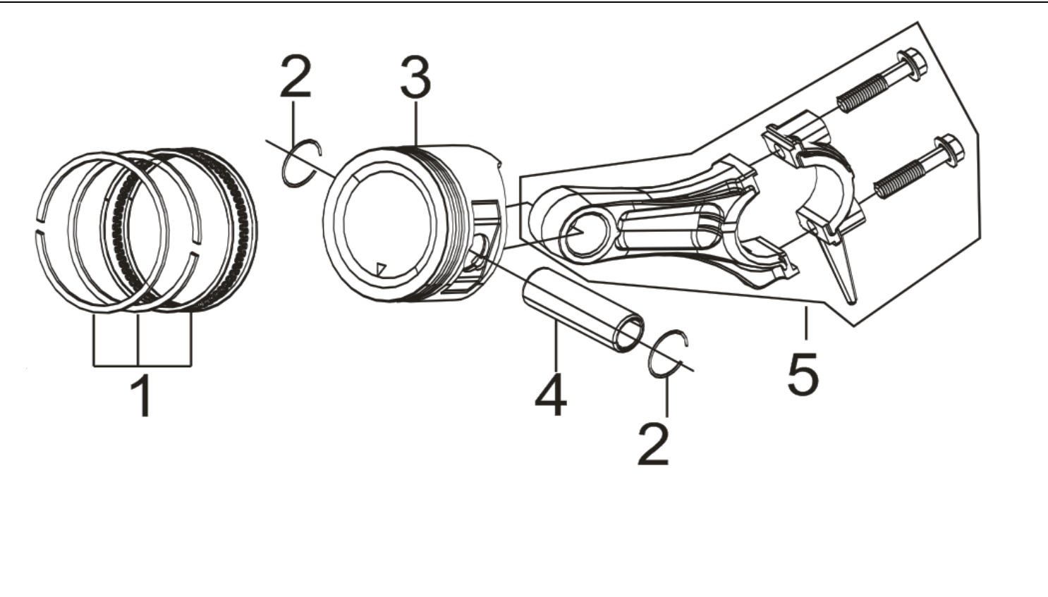
FIG.5 RING SET,OIL / ROD,CRANKSHAFT CONNETING (E05)
