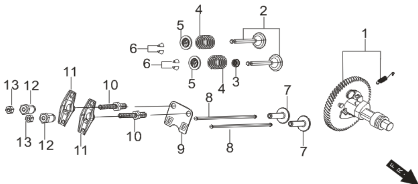
FIG.6 TRAIN,VALVE / CAMSHAFT SUBASSEMBLY. (E06)
