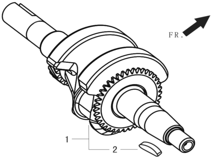
FIG.4 ROD,CRANKSHAFT CONNETING (E04)
