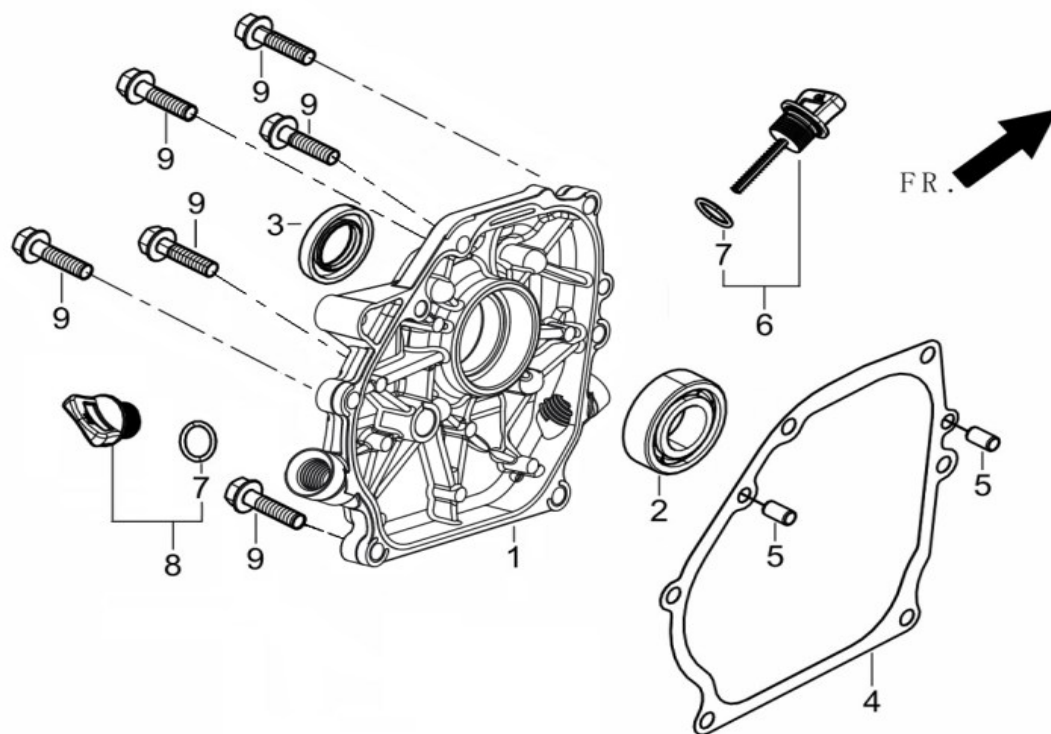
FIG.2 COVER SUBASSEMBLY, CRANKCASE. (E02)
