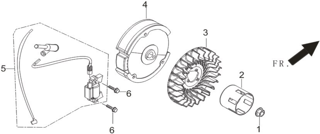
FIG.10 FLYWHEEL / IMPELLER / STARTER PULLEY / IGNITION COIL. (E10)
