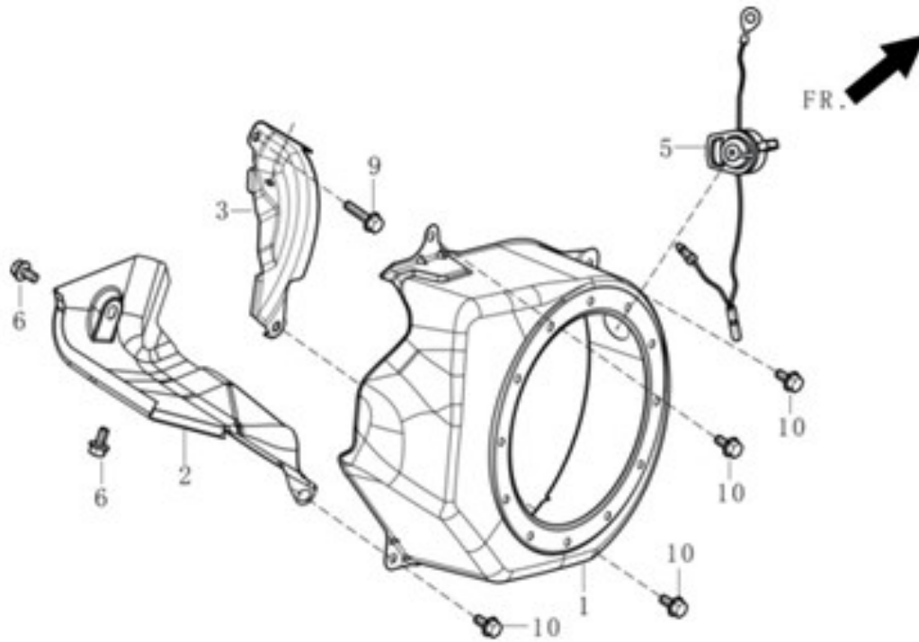
FIG.8 SHROUD / SHIELD,LOWER. (E08)
