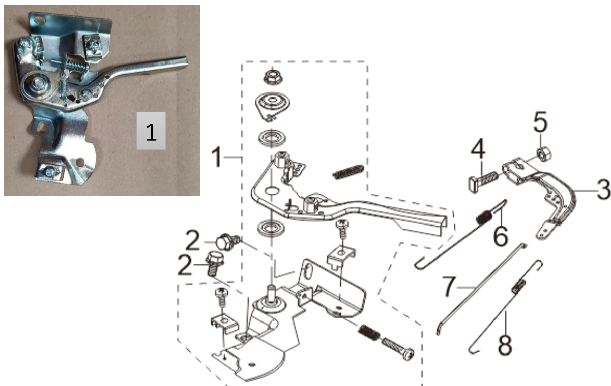
FIG.11 CONTROL ASSY, THROTTLE. (E11)
