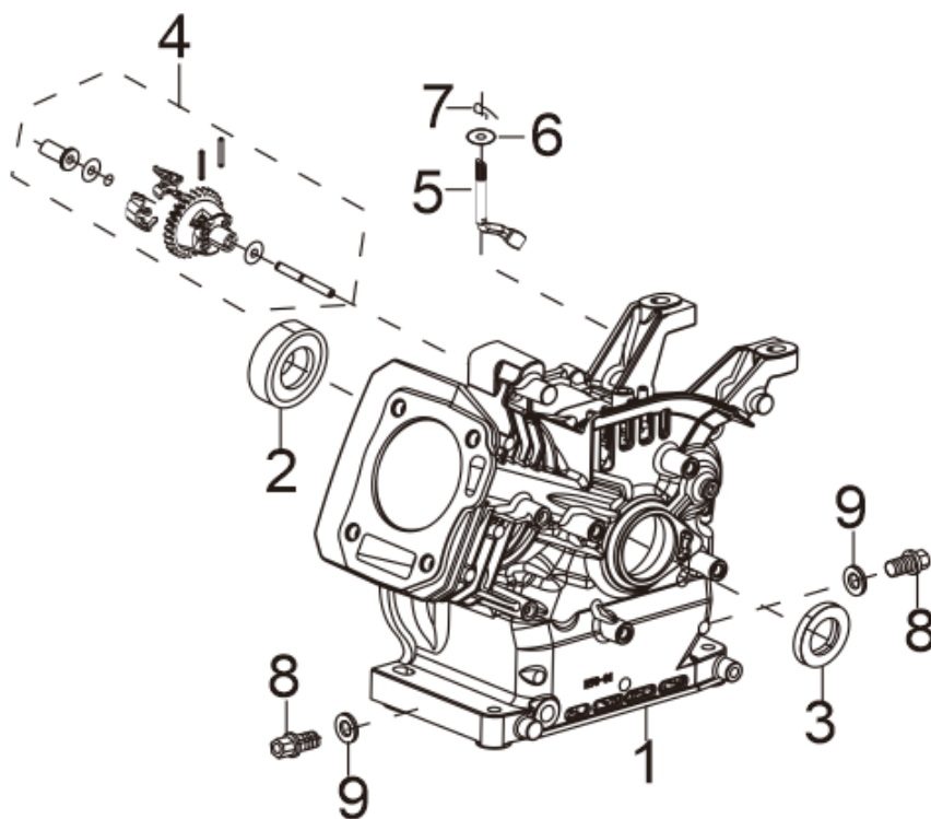
FIG.1 CRANKCASE. / GEAR ASSY, GOVERNOR. (E01)
