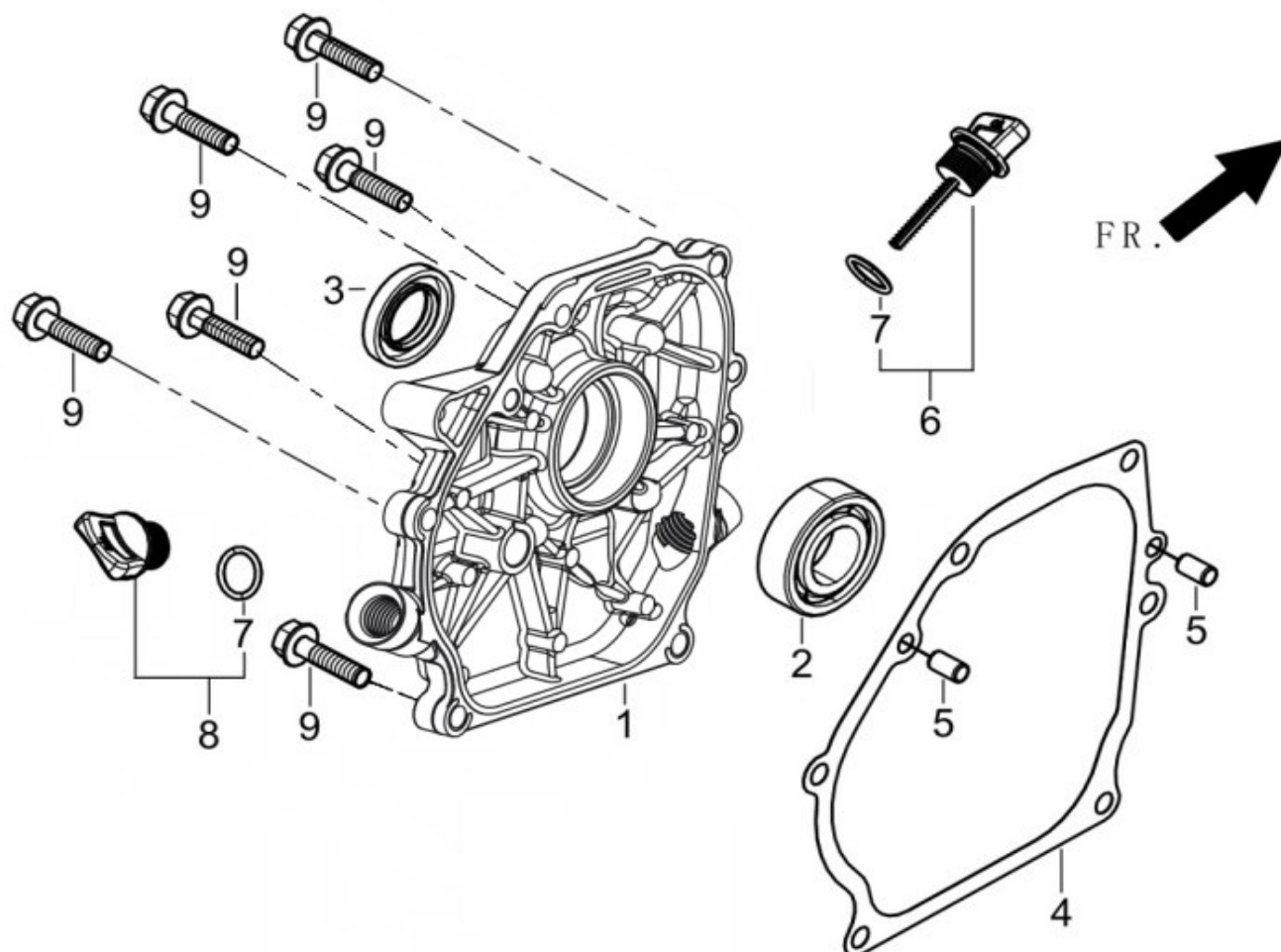
FIG.2 COVER SUBASSEMBLY, CRANKCASE(E02)
