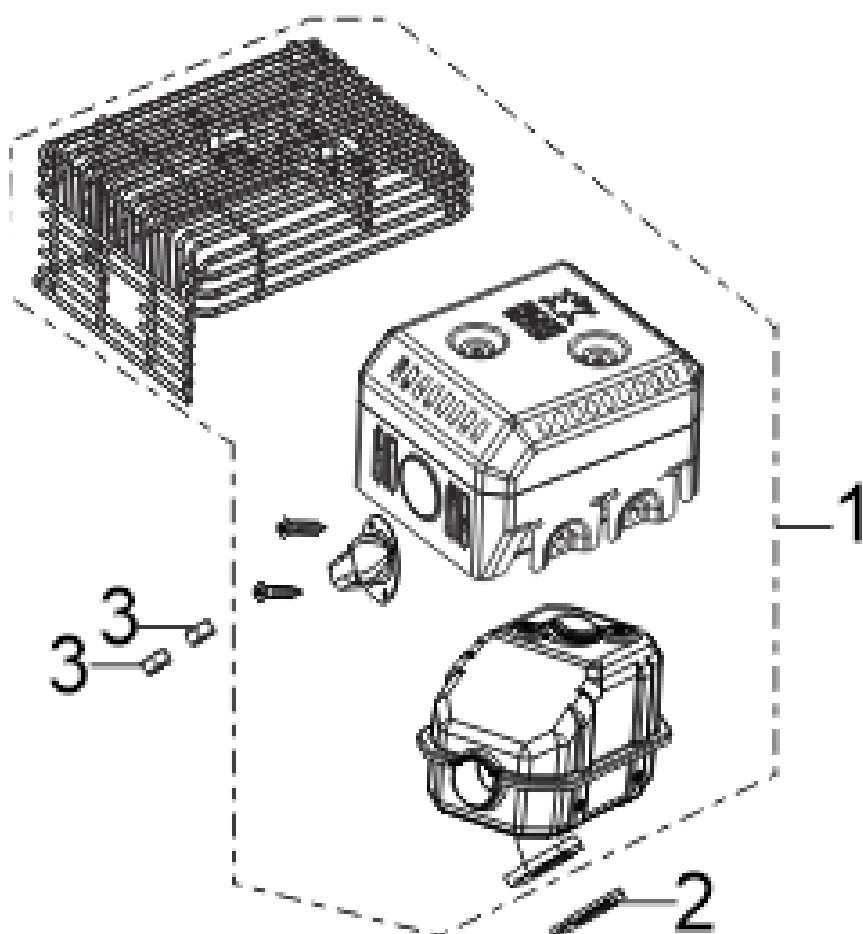
FIG.13 MUFFLER ASSY. (F02)
