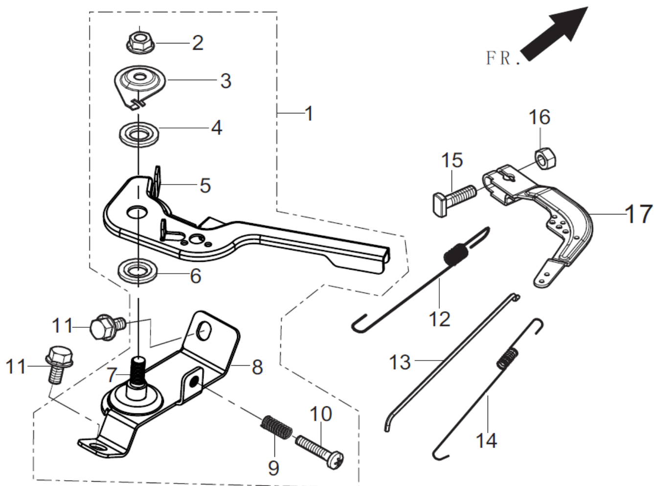
FIG.11 CONTROL ASSY, THROTTLE (E11)
