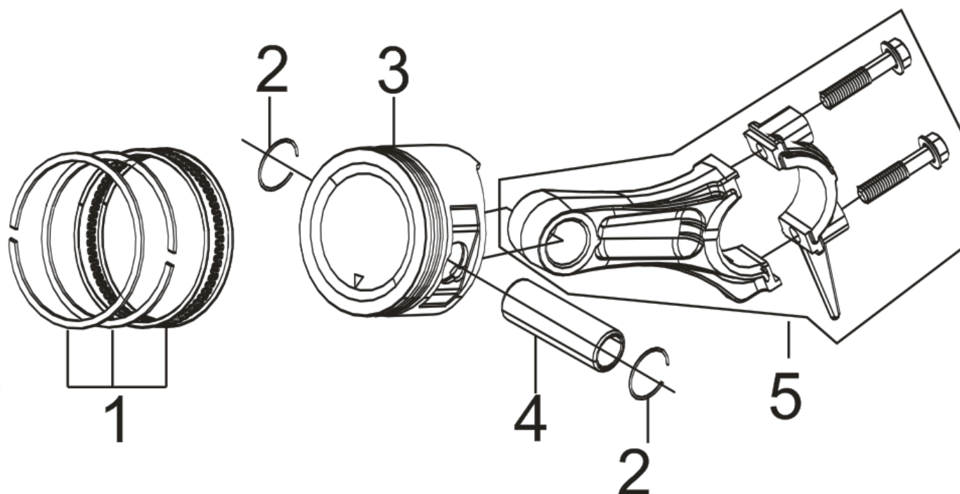
FIG.5 RING SET,OIL / ROD,CRANKSHAFT CONNETING (E05)
