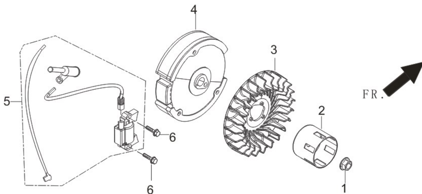
FIG.10 FLYWHEEL / IMPELLER / STARTER PULLEY / IGNITION COIL (E10)
