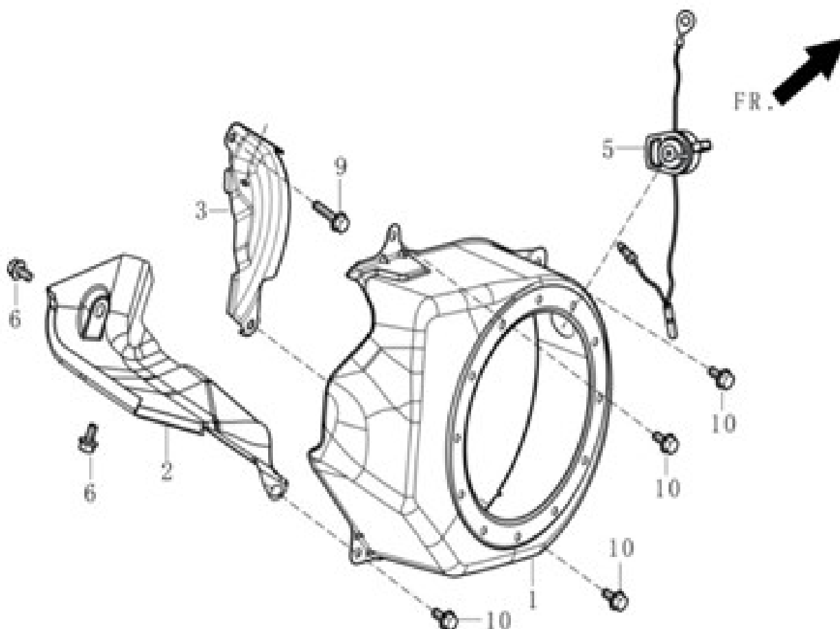
FIG.8 SHROUD / SHIELD,LOWER (E08)
