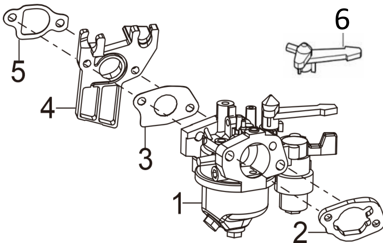
FIG.9 CARBURETOR ASSY. (E09)
