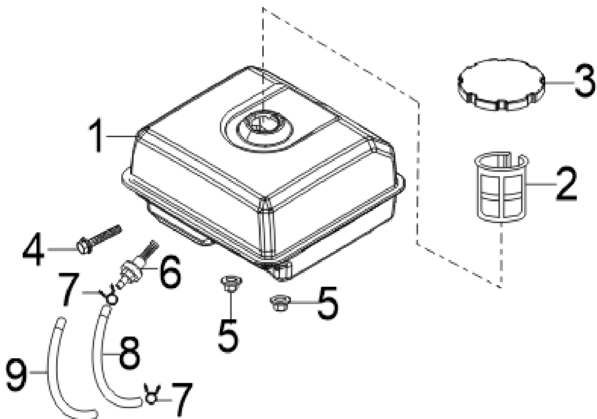
FIG.14 TANK ASSY, FUEL (F03)
