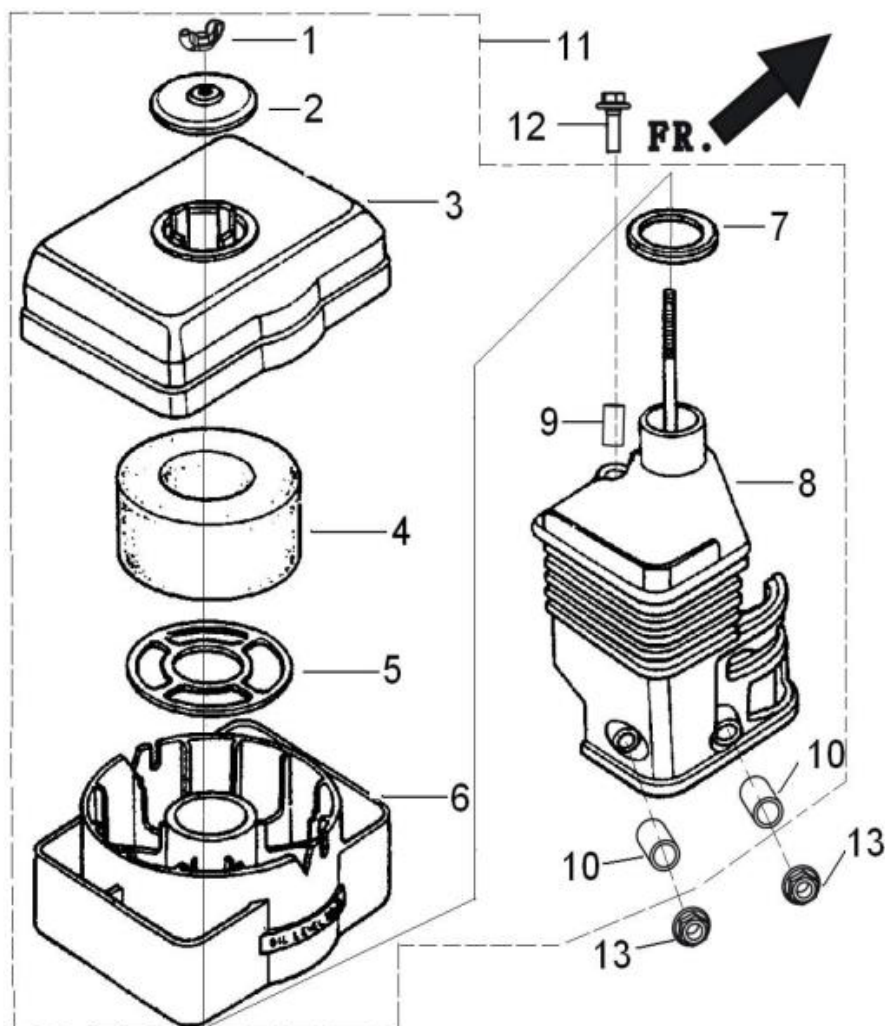
FIG.12 CLEANER, AIR (F01)
