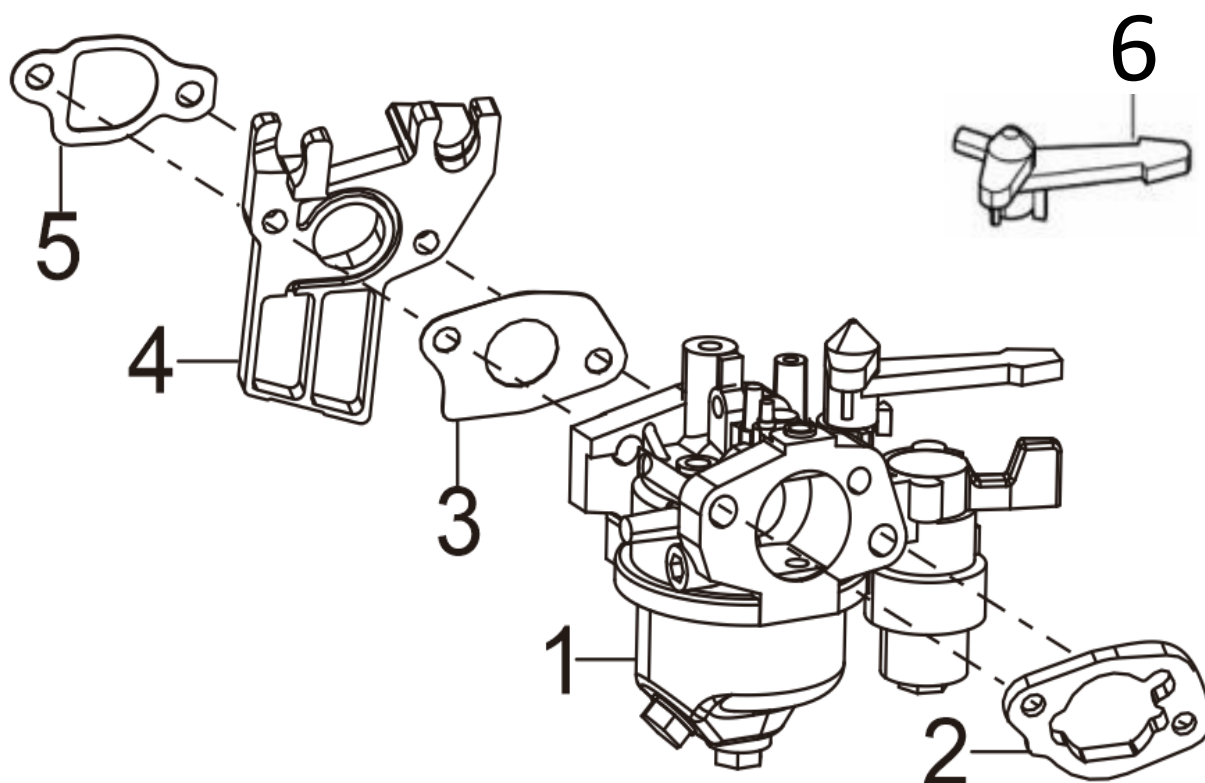
FIG.9 CARBURETOR ASSY. (E09)
