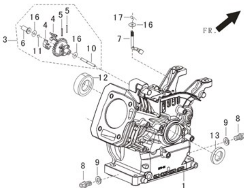
FIG.1 CRANKCASE. / GEAR ASSY, GOVERNOR.(E01)
