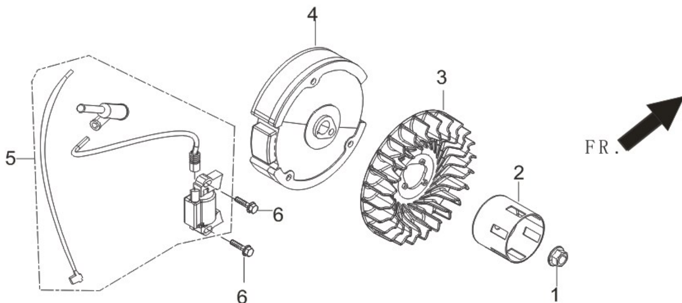
FIG.10 FLYWHEEL / IMPELLER / STARTER PULLEY / IGNITION COIL (E10)
