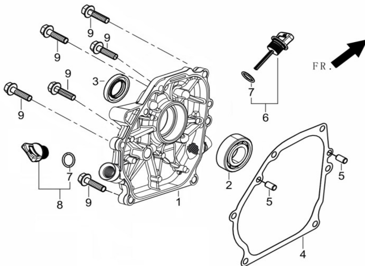
FIG.2 COVER SUBASSEMBLY, CRANKCASE(E02)
