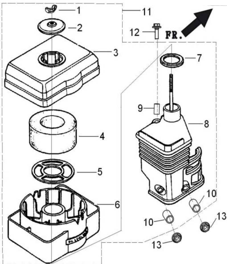
FIG.12 CLEANER, AIR (F01)
