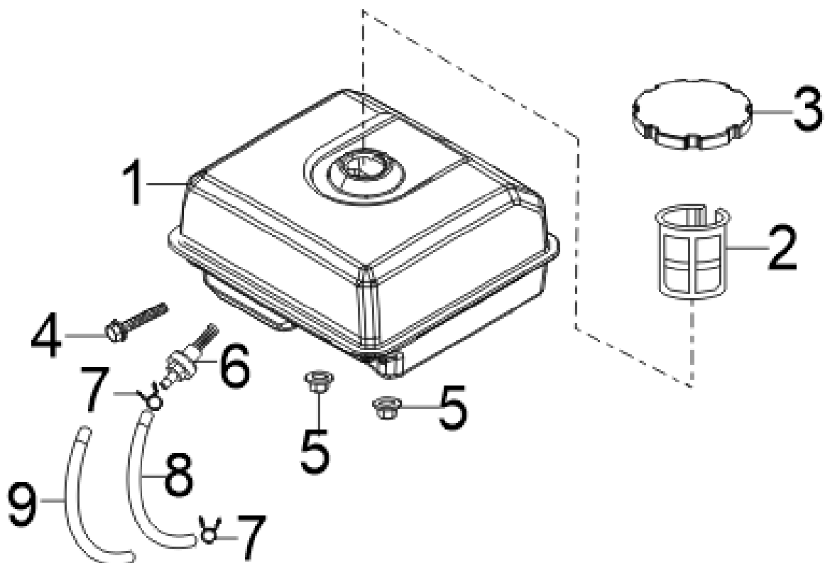
FIG.14 TANK ASSY, FUEL (F03)
