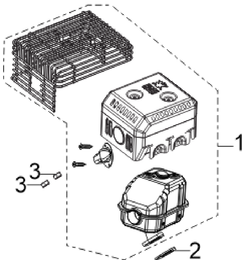
FIG.13 MUFFLER ASSY. (F02)
