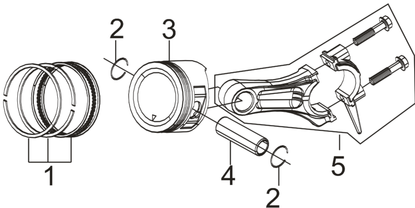
FIG.5 RING SET,OIL / ROD,CRANKSHAFT CONNETING (E05)
