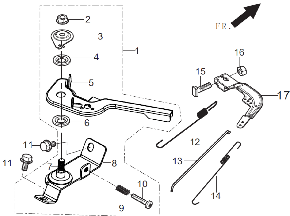
FIG.11 CONTROL ASSY, THROTTLE (E11)
