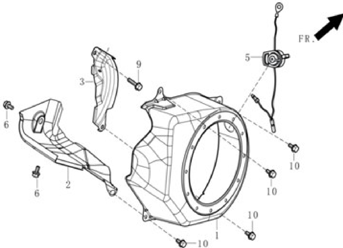
FIG.8 SHROUD / SHIELD,LOWER (E08)
