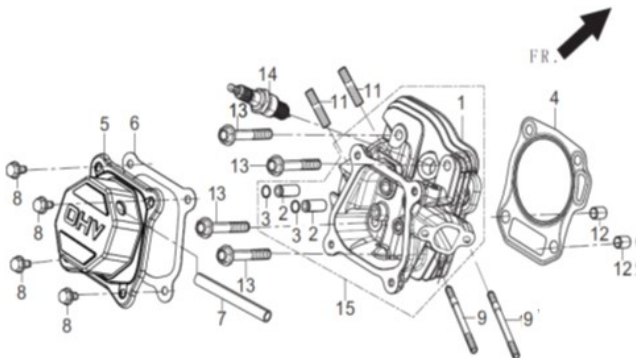
FIG.3 HEAD SUBASSEMBLY, CYLINDER / PLUG,SPARK (E03)
