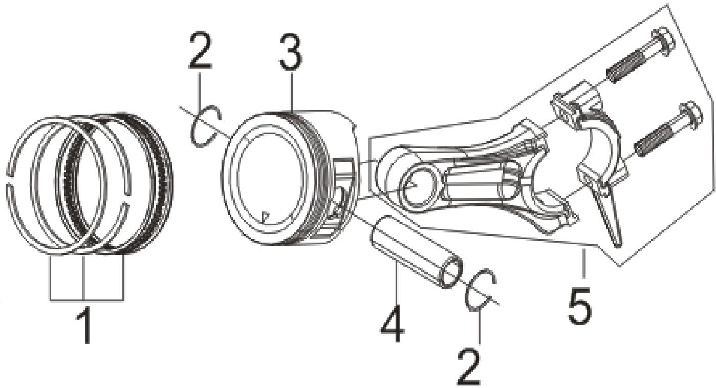
FIG.5 RING SET,OIL / ROD,CRANKSHAFT CONNETING.(E05)
