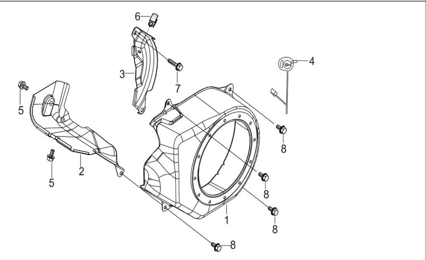
FIG.8 SHROUD / SHIELD,LOWER.(E08)
