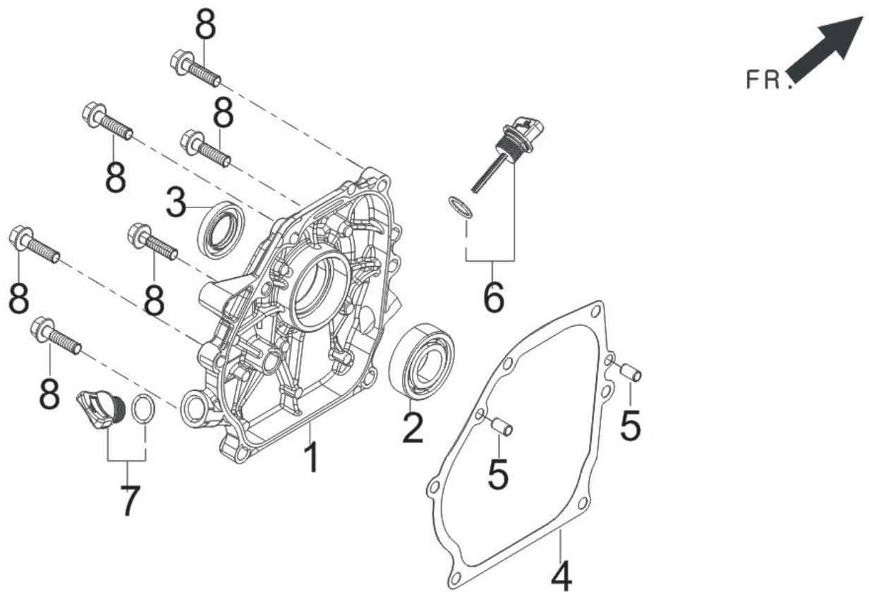
FIG.2 COVER SUBASSEMBLY, CRANKCASE.(E02)
