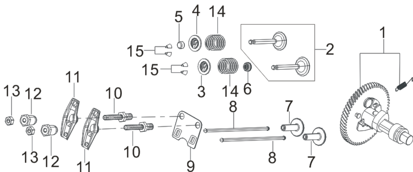
FIG.6 TRAIN,VALVE / CAMSHAFT SUBASSEMBLY.(E06)
