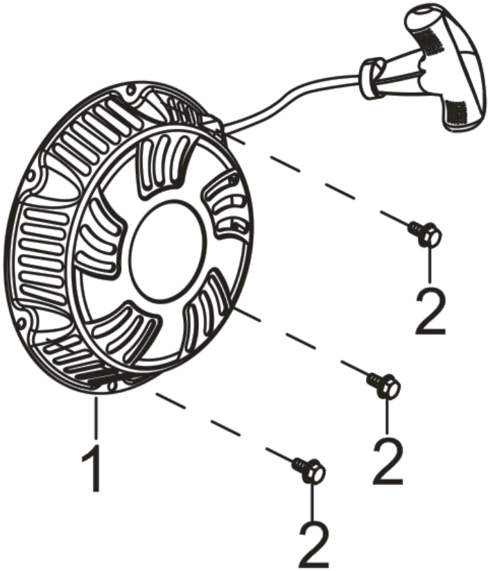
FIG.7 STARTER,RECOIL.(E07)
