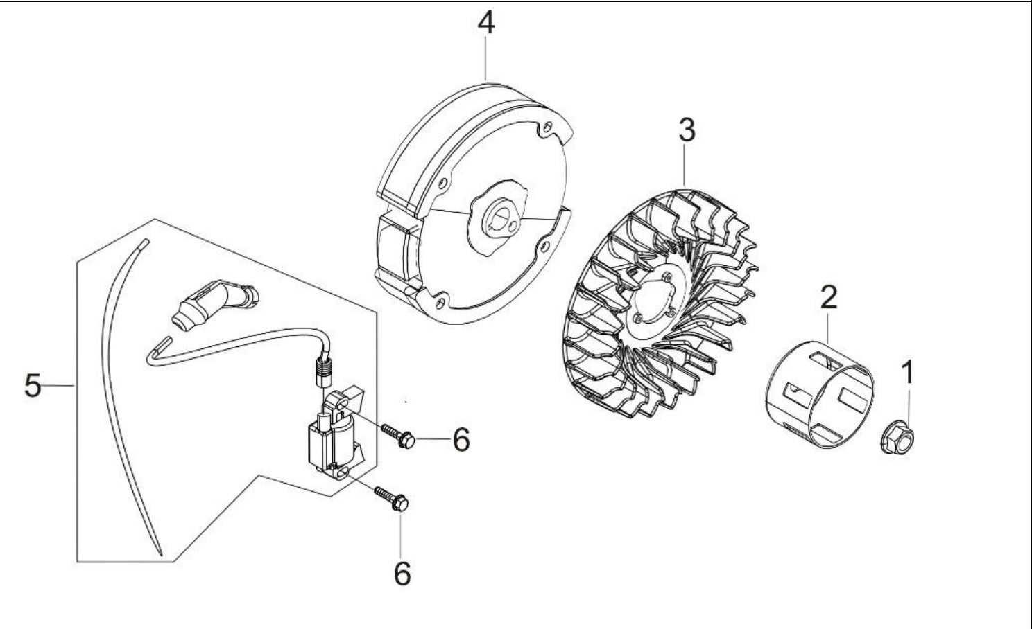
FIG.10 FLYWHEEL / IMPELLER / STARTER PULLEY / IGNITION COIL.(E10)
