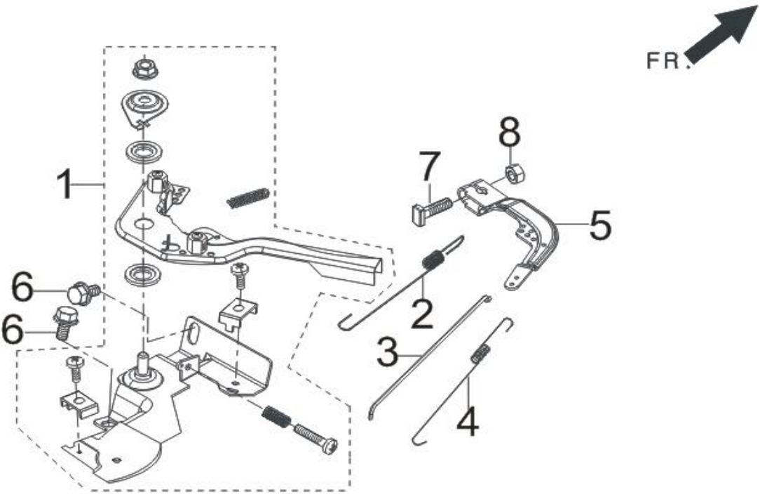
FIG.11 CONTROL ASSY, THROTTLE.(E11)
