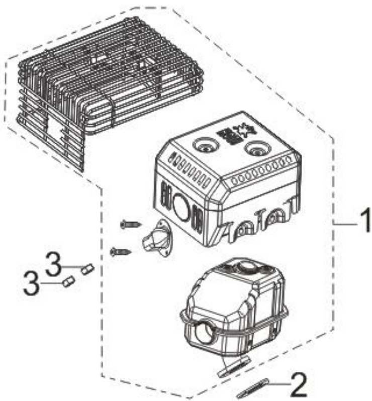
FIG.13 MUFFLER ASSY.(F02)
