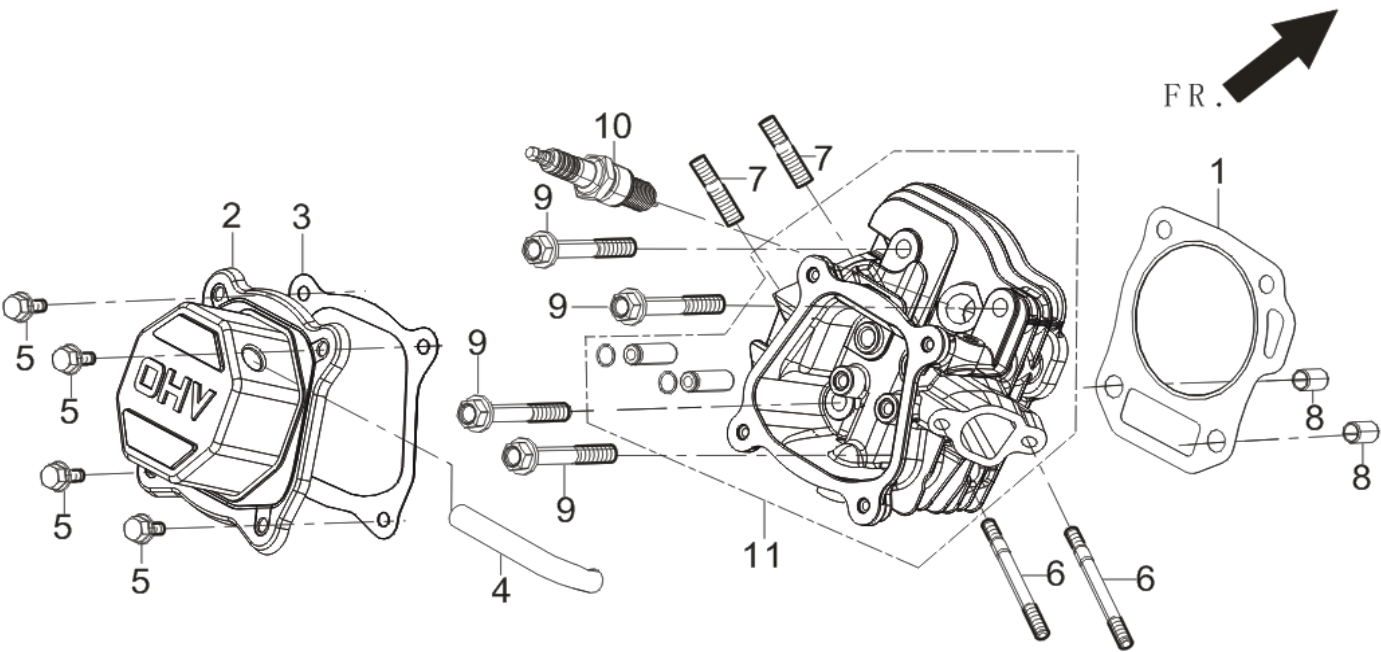
FIG.3 HEAD SUBASSEMBLY, CYLINDER / PLUG,SPARK.(E03)
