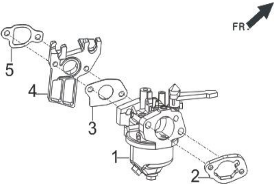
FIG.9 CARBURETOR ASSY.(E09)
