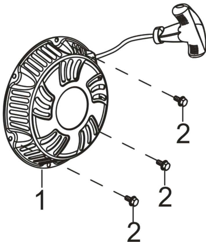
FIG.7 STARTER,RECOIL.(E07)
