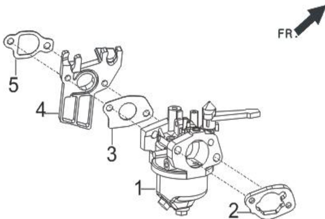
FIG.9 CARBURETOR ASSY.(E09)
