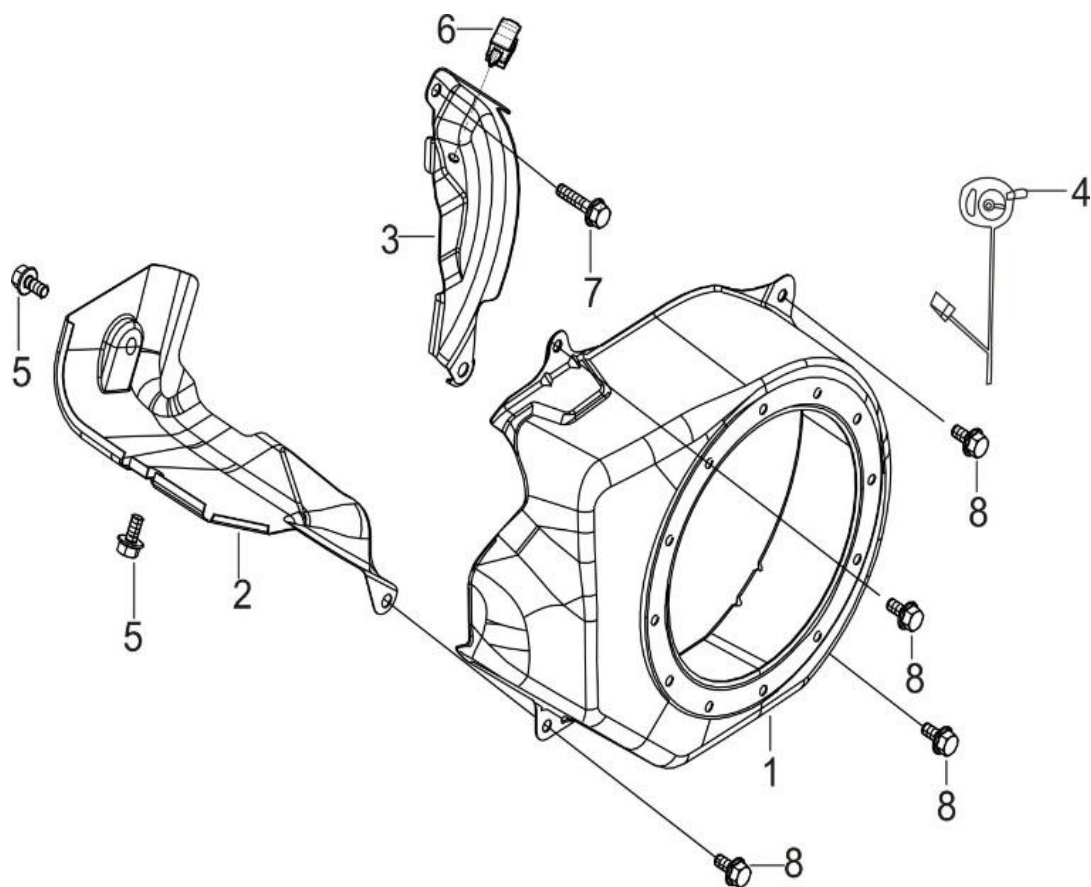
FIG.8 SHROUD / SHIELD,LOWER.(E08)
