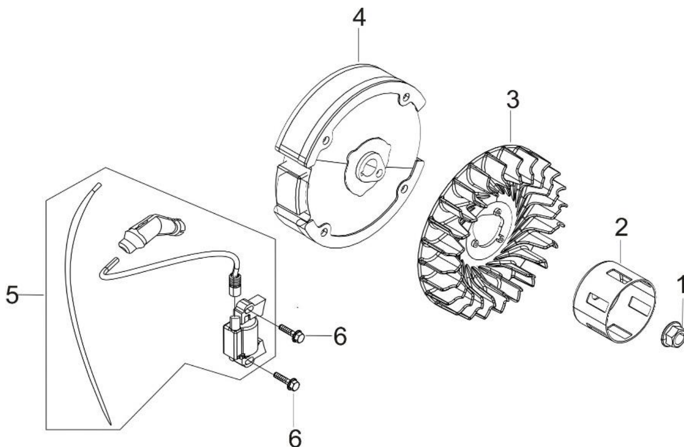
FIG.10 FLYWHEEL / IMPELLER / STARTER PULLEY / IGNITION COIL.(E10)
