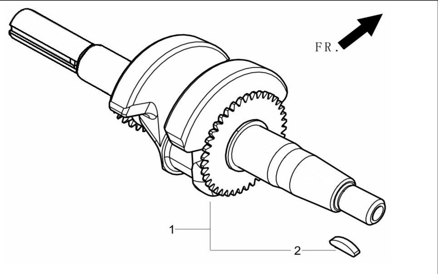
FIG.4 ROD,CRANKSHAFT CONNETING.(E04)
