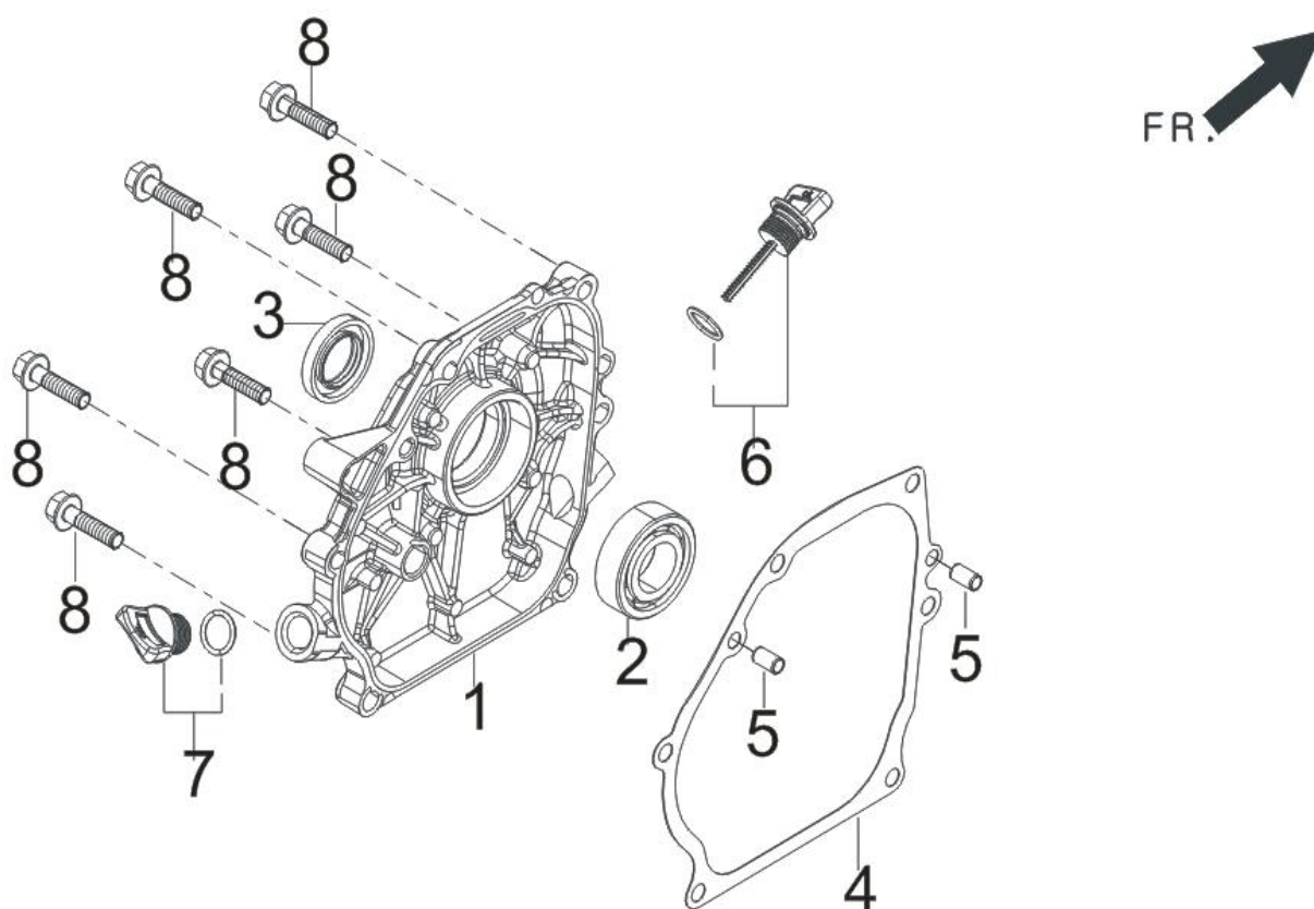
FIG.2 COVER SUBASSEMBLY, CRANKCASE.(E02)
