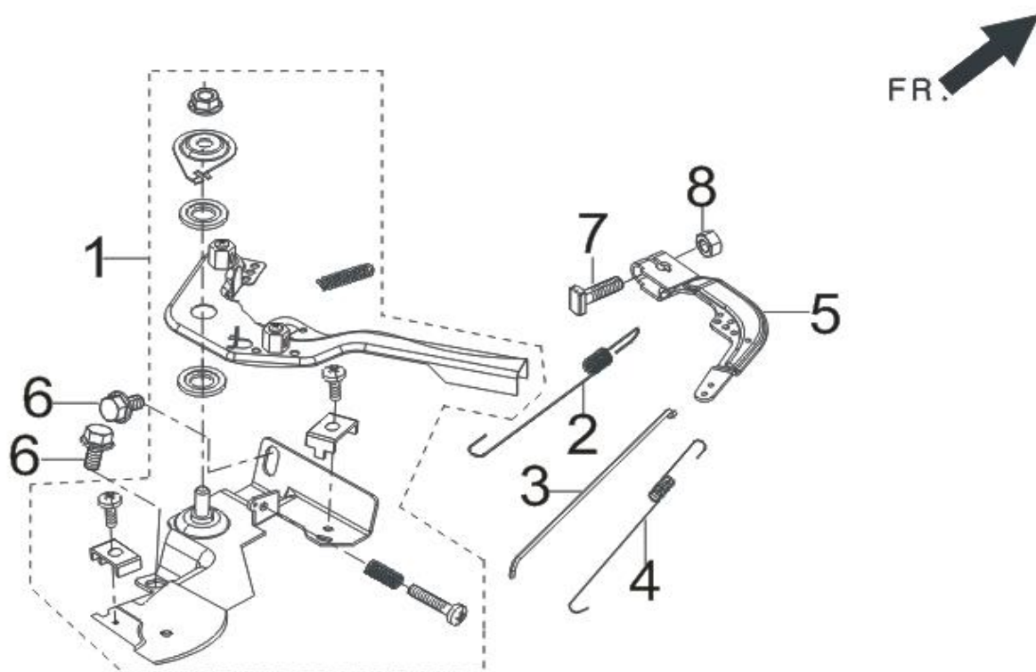
FIG.11 CONTROL ASSY, THROTTLE.(E11)
