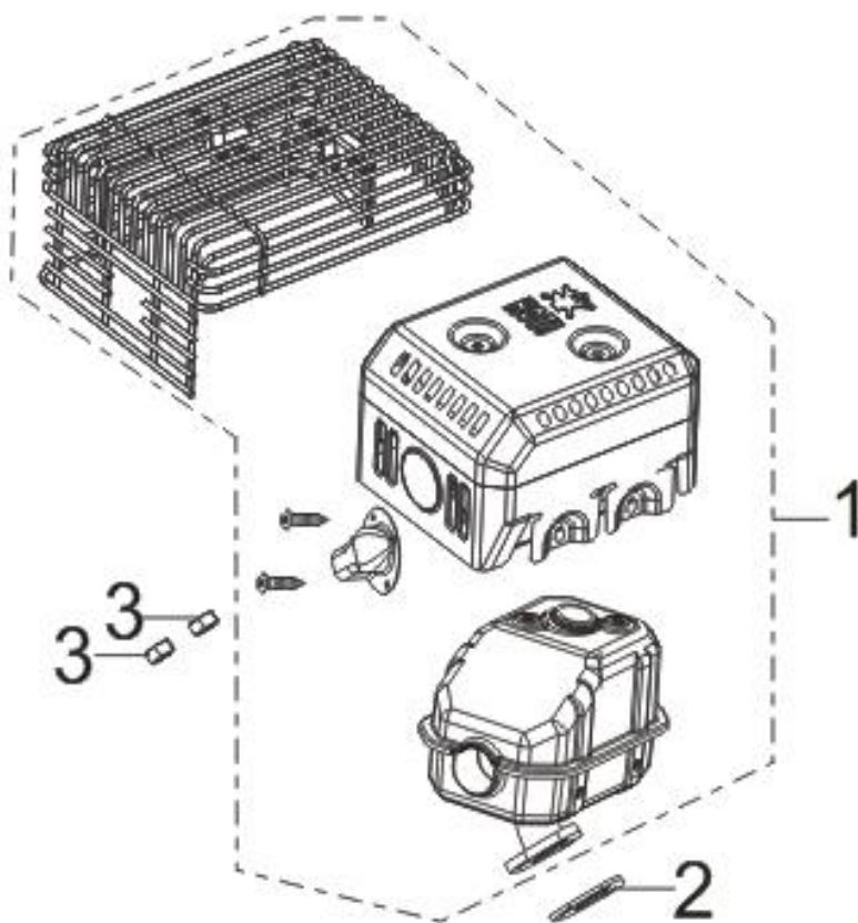
FIG.13 MUFFLER ASSY.(F02)
