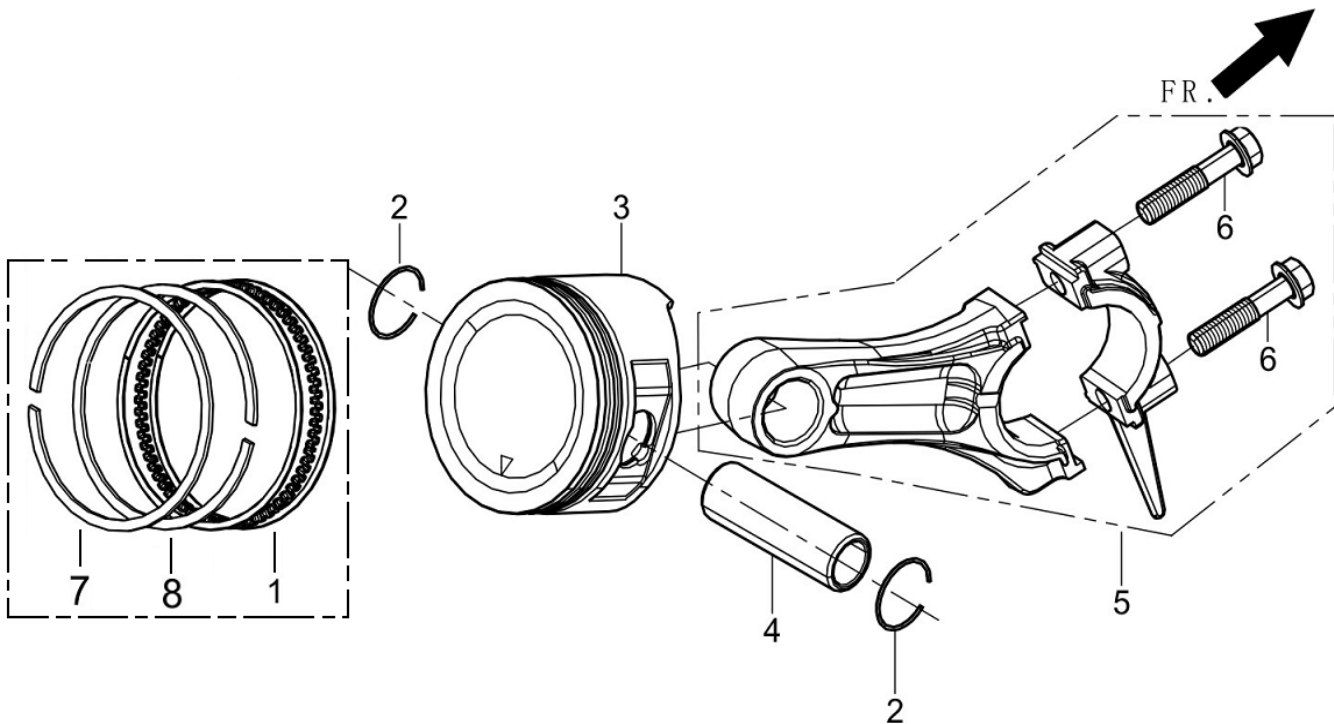
FIG.5 RING SET,OIL / ROD,CRANKSHAFT CONNETING (E06)
