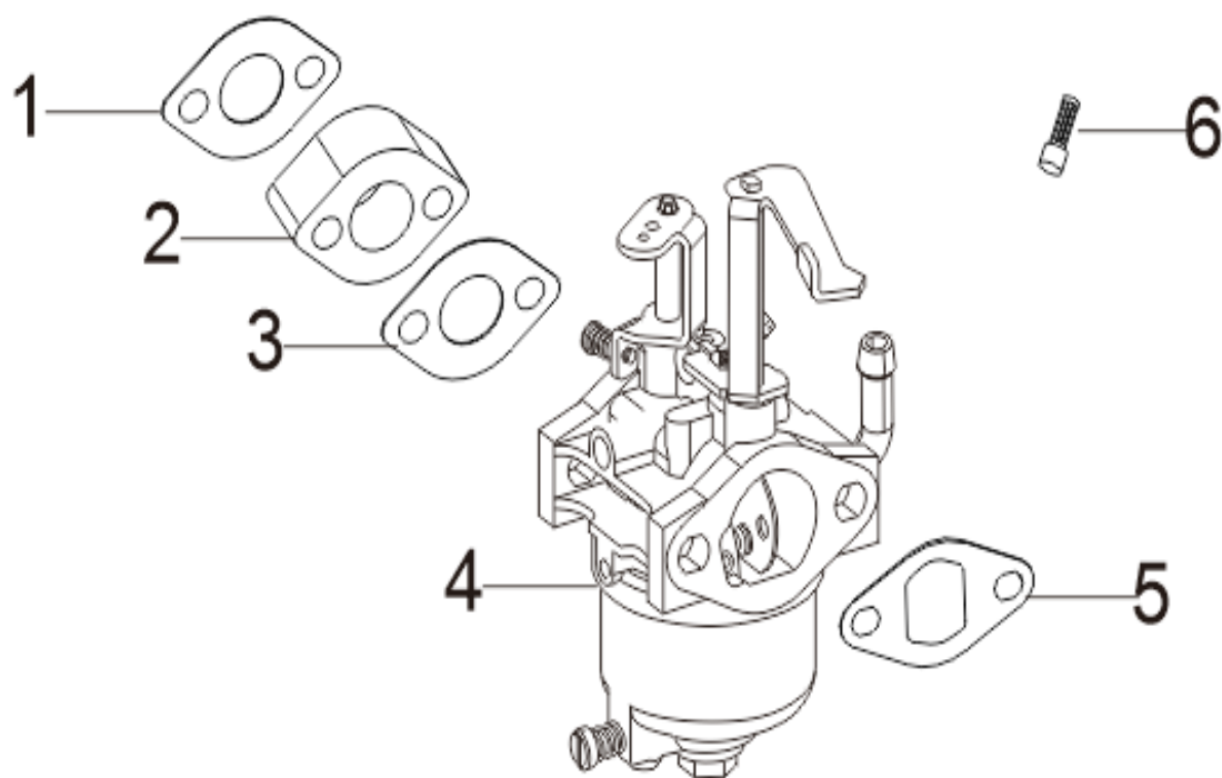
FIG.9 CARBURETOR ASSY. (E11)
