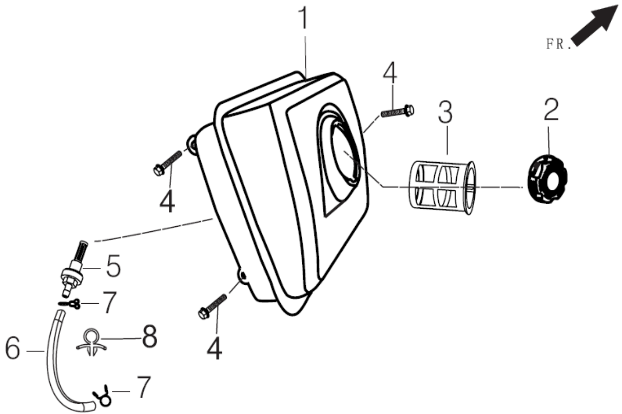
FIG.12 TANK ASSY, FUEL (F01)
