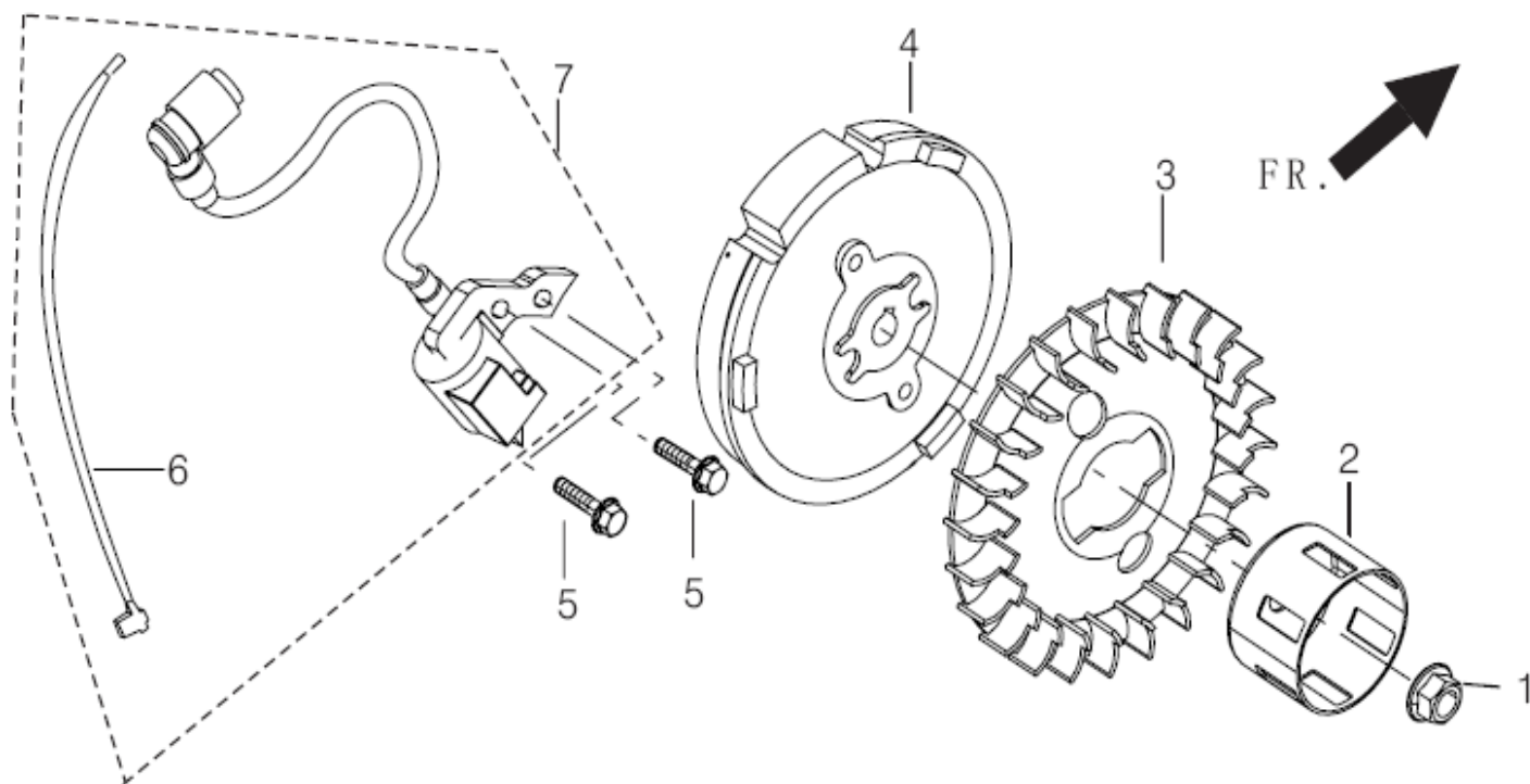
FIG.13 FLYWHEEL / IMPELLER / STARTER PULLEY / IGNITION COIL (E15)
