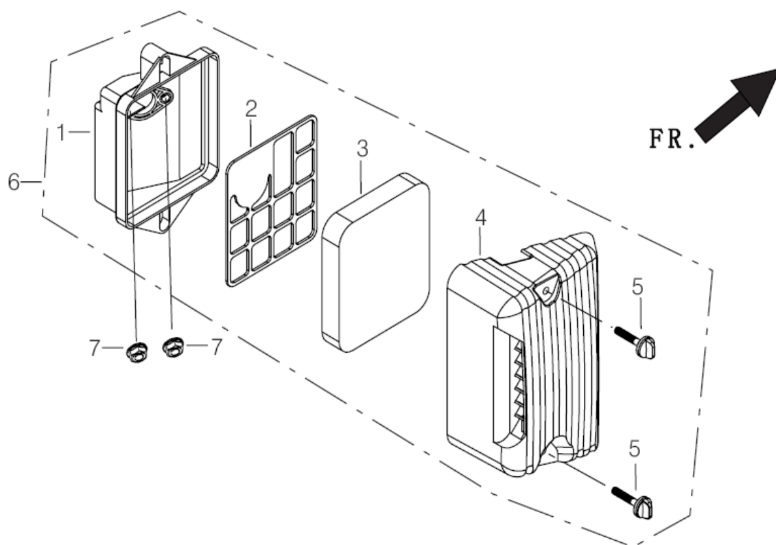
FIG.10 CLEANER, AIR (F02)
