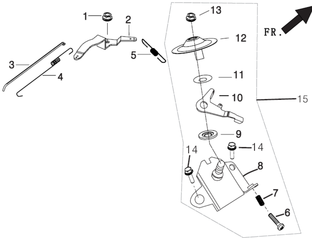
FIG.14 CONTROL ASSY, THROTTLE (E13)
