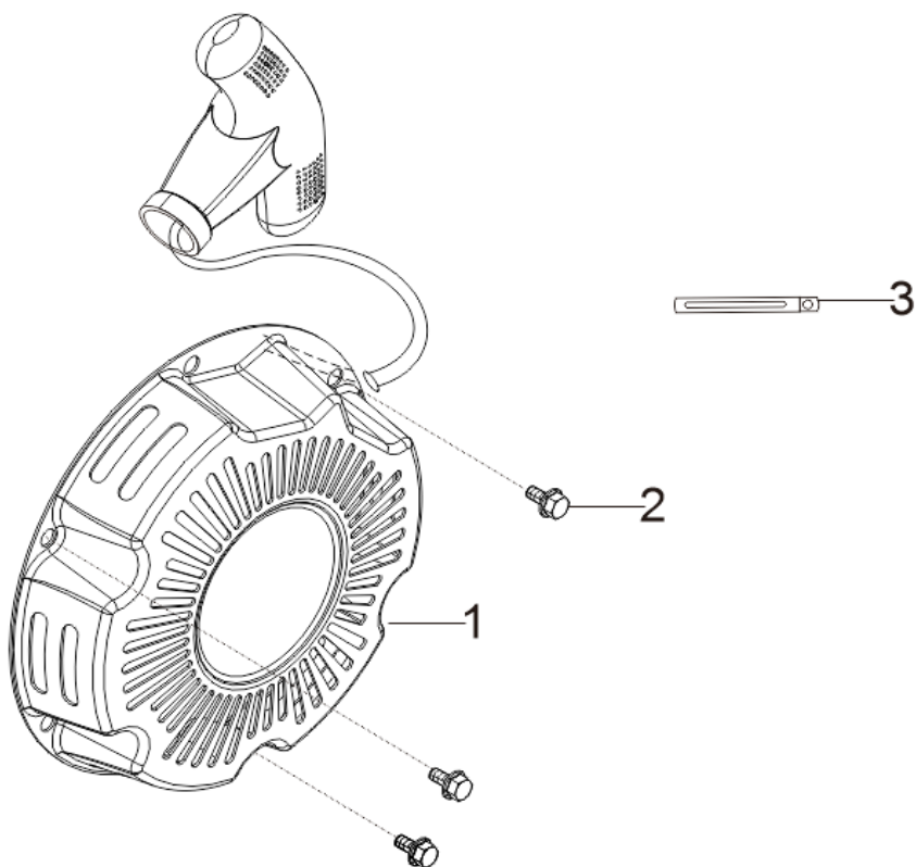
FIG.7 STARTER,RECOIL (E08)
