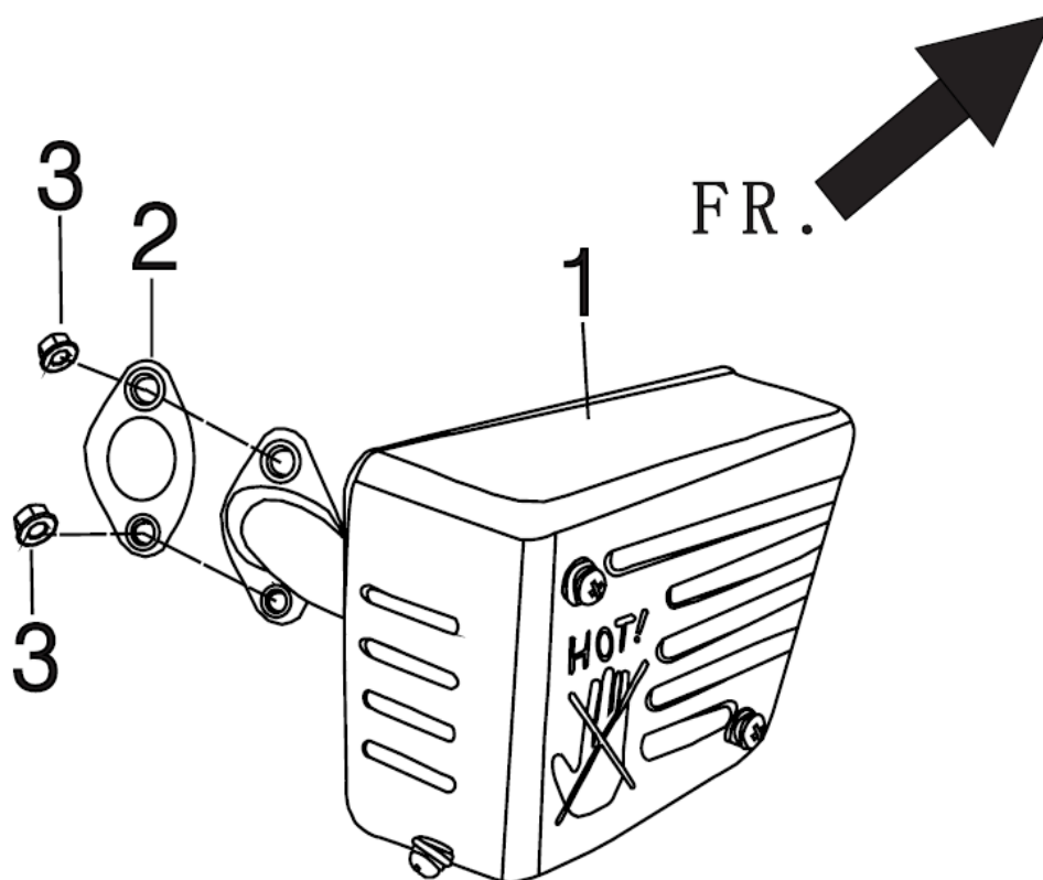
FIG.11 MUFFLER ASSY. (F04)
