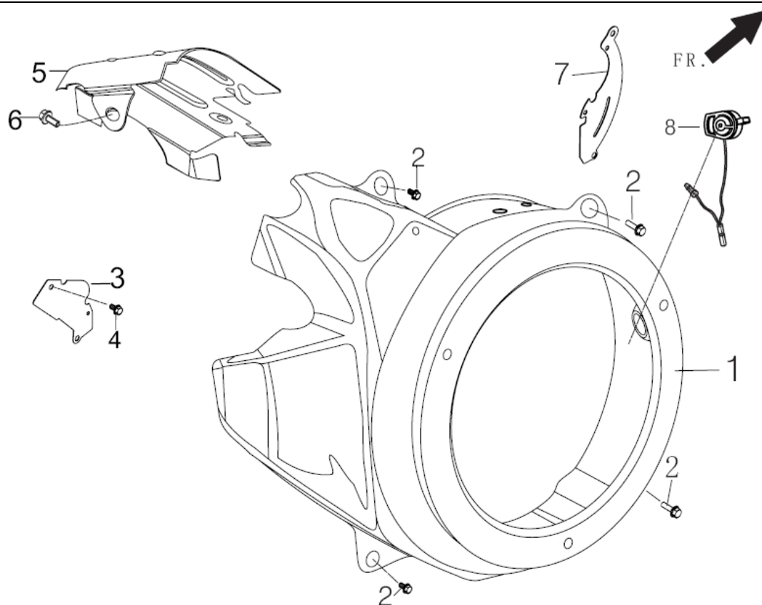
FIG.8 SHROUD / SHIELD,LOWER (E14)
