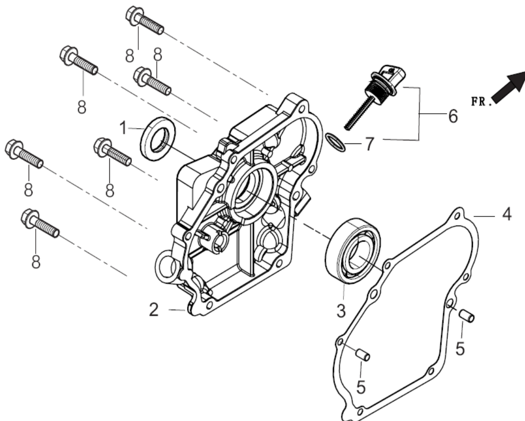
FIG.3 COVER SUBASSEMBLY, CRANKCASE (E01)
