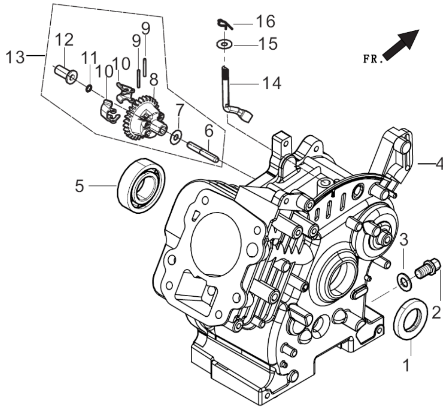
FIG.2 CRANKCASE. / GEAR ASSY, GOVERNOR. (E17)
