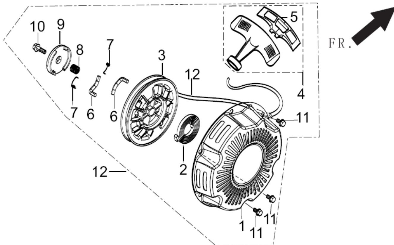
FIG.7 STARTER,RECOIL (E08)
