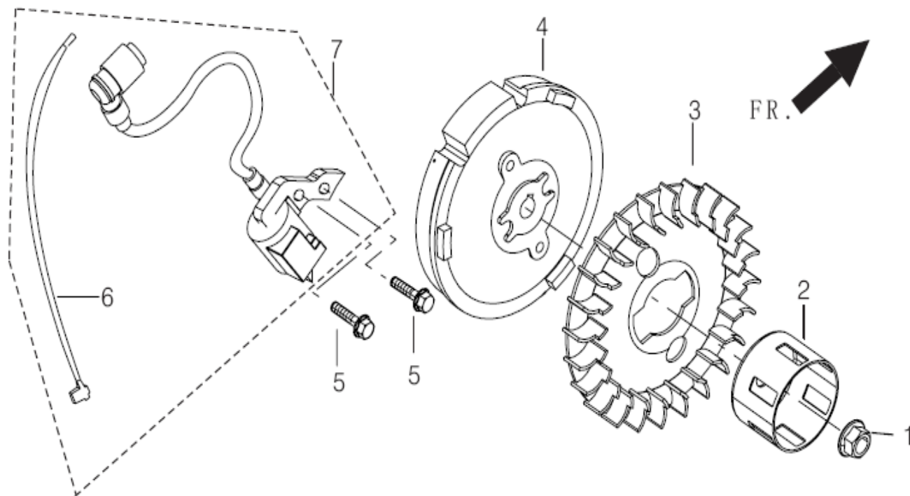
FIG.13 FLYWHEEL / IMPELLER / STARTER PULLEY / IGNITION COIL (E15)
