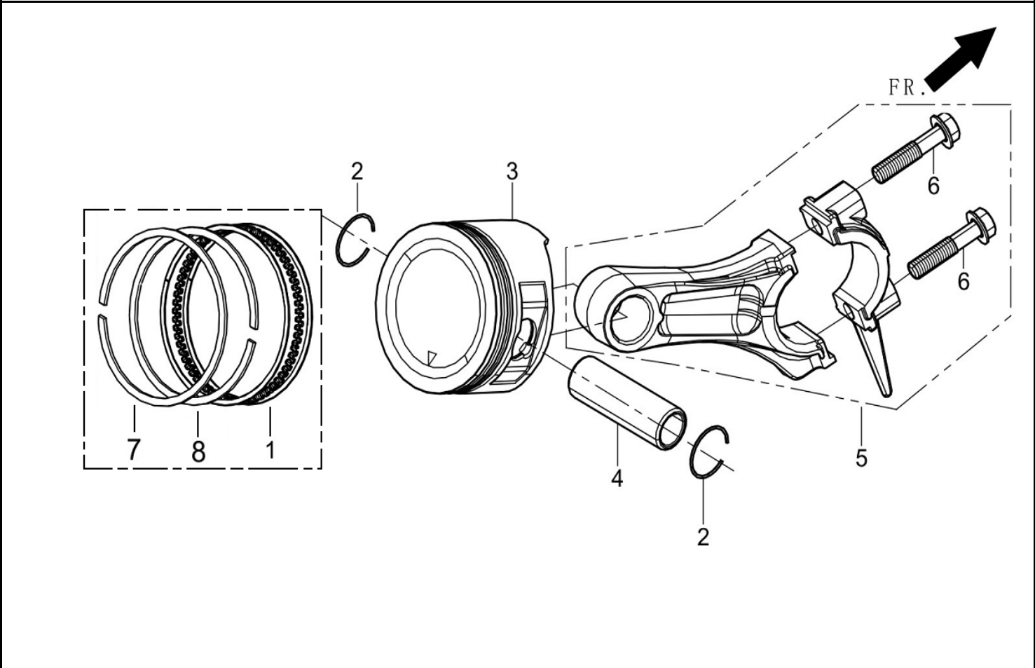
FIG.5 RING SET,OIL / ROD,CRANKSHAFT CONNETING (E06)
