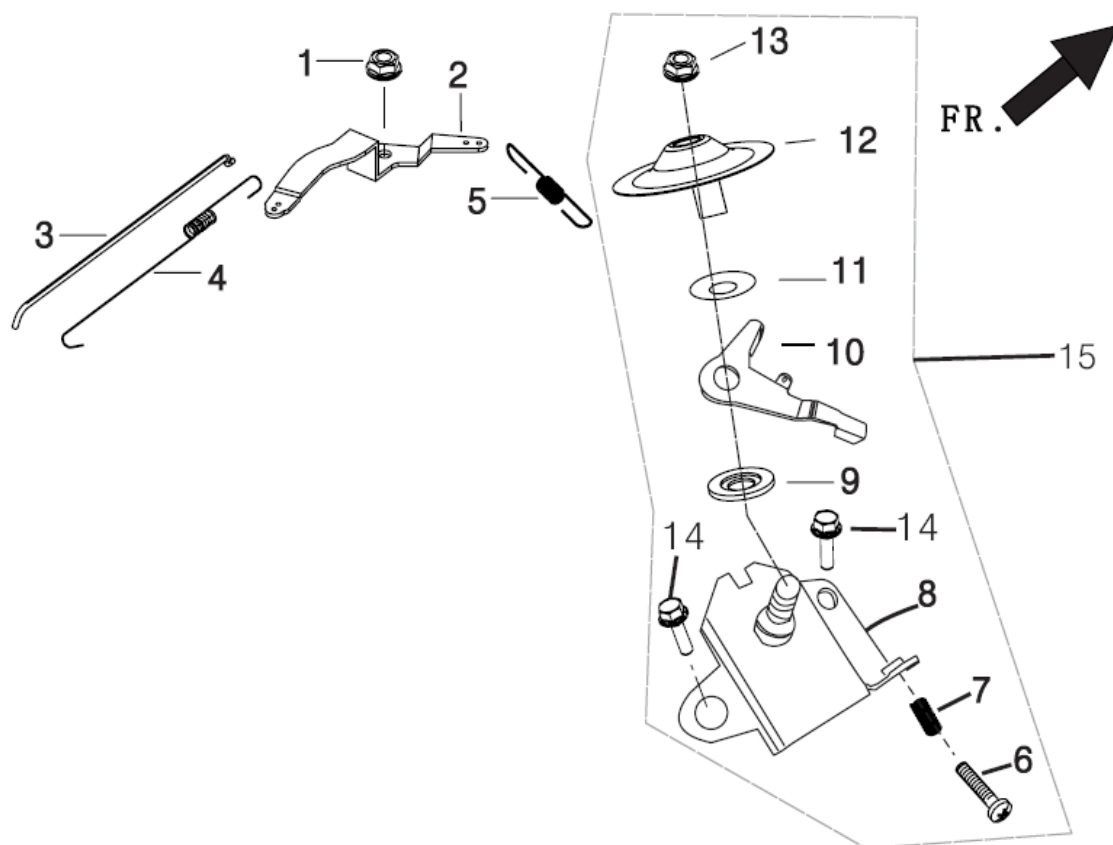
FIG.14 CONTROL ASSY, THROTTLE (E13)
