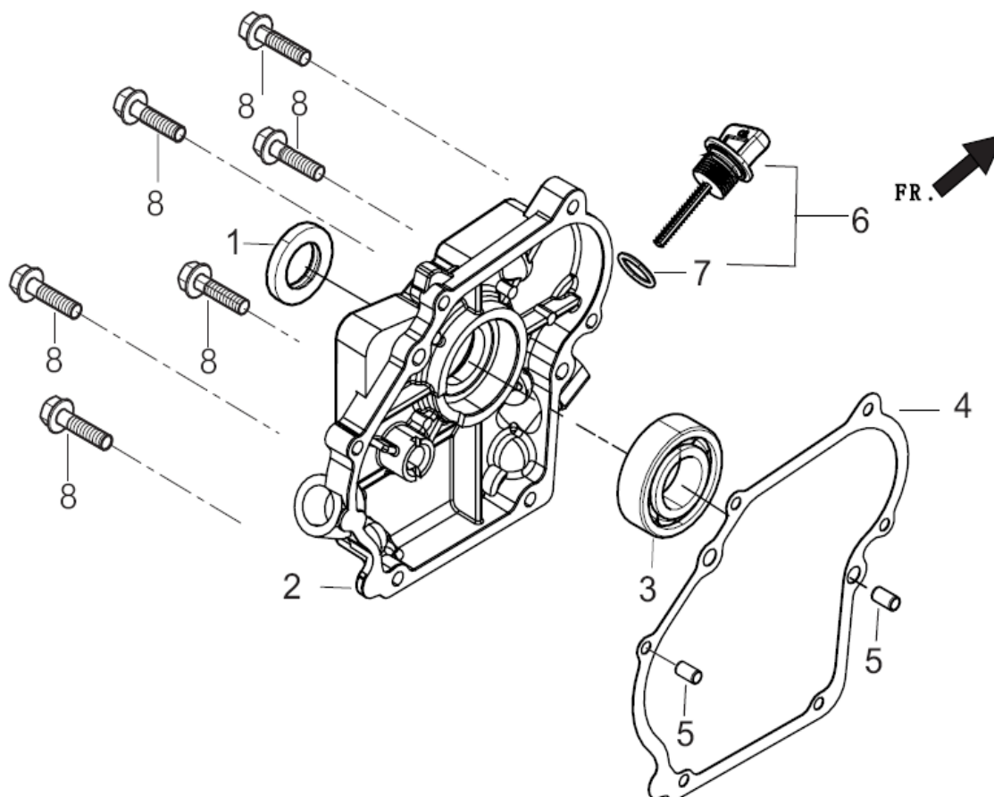
FIG.3 COVER SUBASSEMBLY, CRANKCASE (E01)
