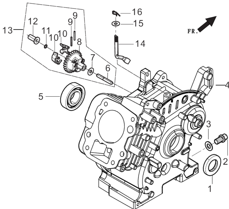
FIG.2 CRANKCASE. / GEAR ASSY, GOVERNOR. (E17)
