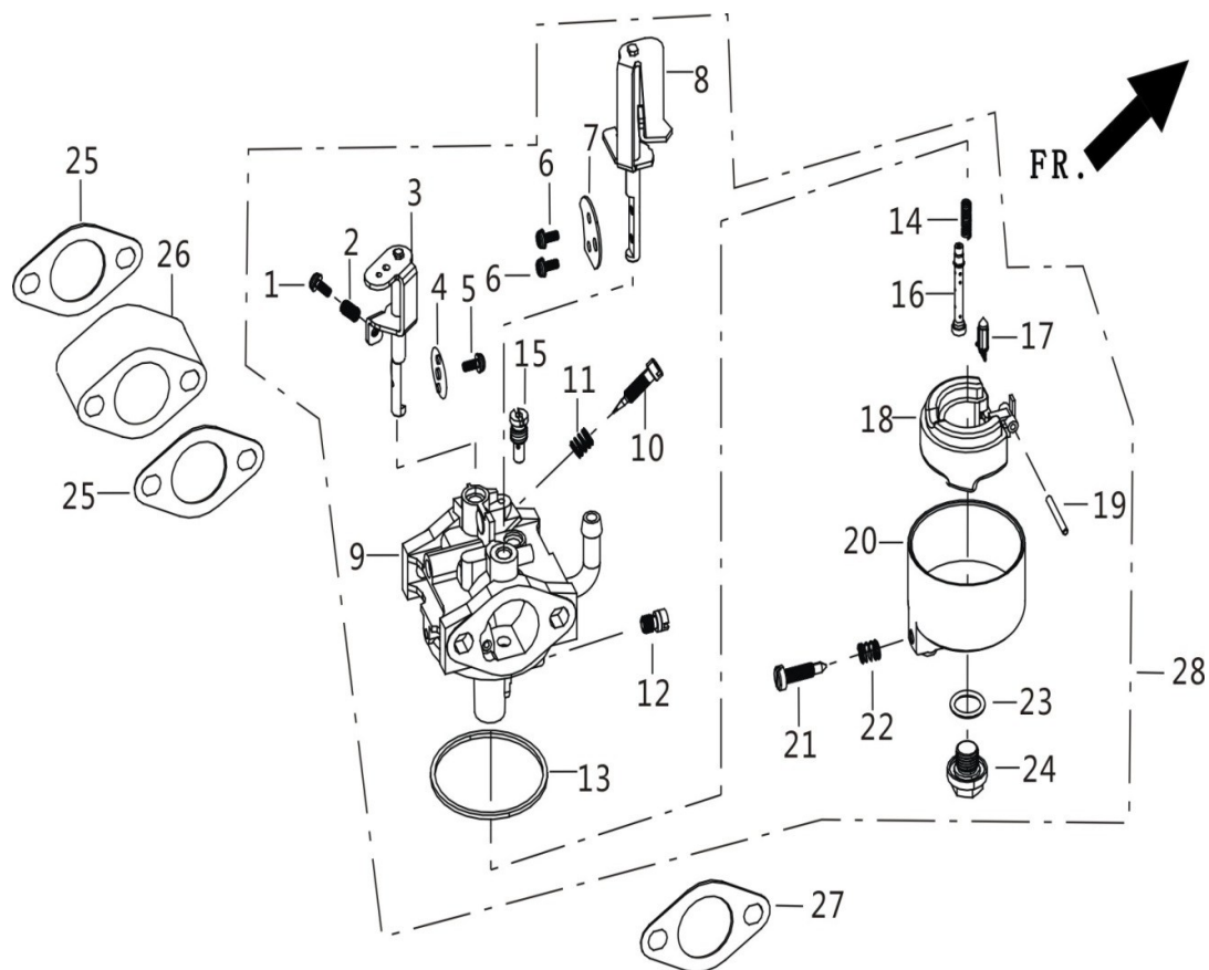
FIG.9 CARBURETOR ASSY. (E11)
