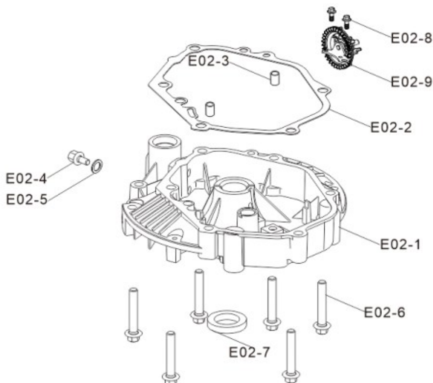
FIG.2 COVER SUBASSEMBLY, CRANKCASE. (E02)
