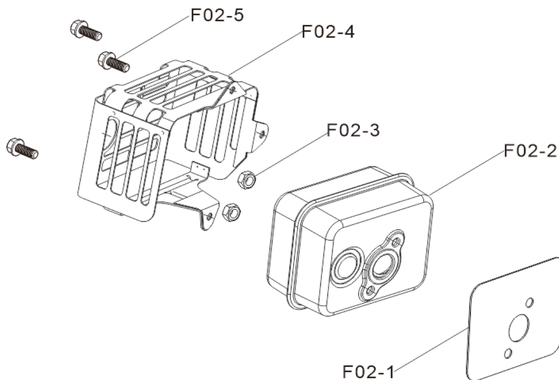
FIG.12 MUFFLER ASSY. (F02)
