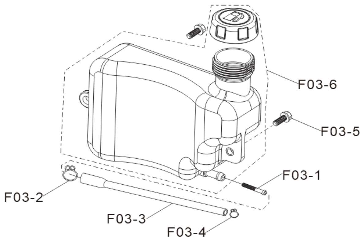
FIG.13 TANK ASSY, FUEL. (F03)
