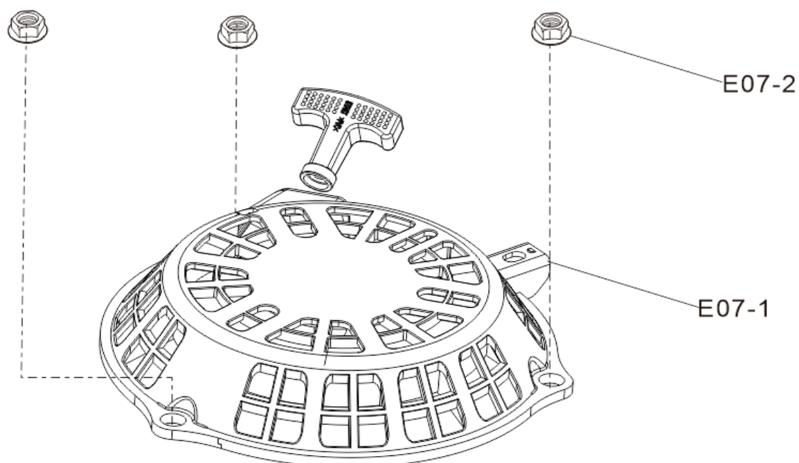
FIG.6 STARTER,RECOIL. (E07)
