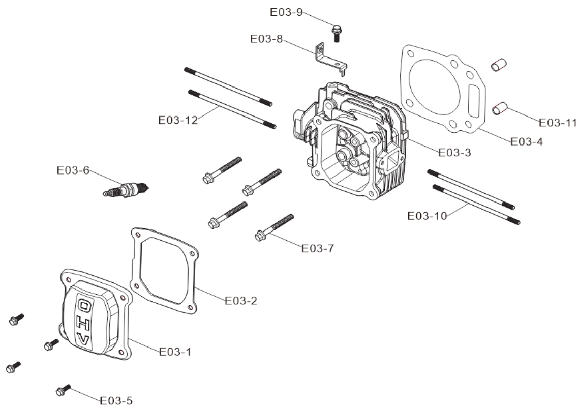
FIG.3 HEAD SUBASSEMBLY, CYLINDER / PLUG, SPARK. (E03)
