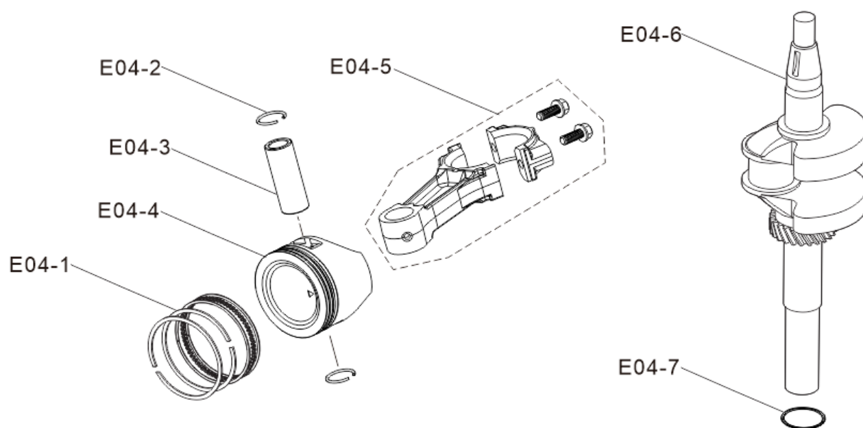
FIG.4 ROD,CRANKSHAFT CONNETING. (E04)
