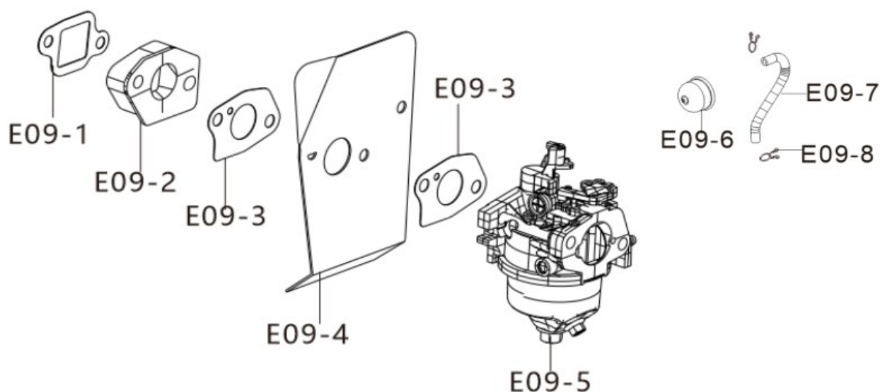
FIG.8 CARBURETOR ASSY. (E09)
