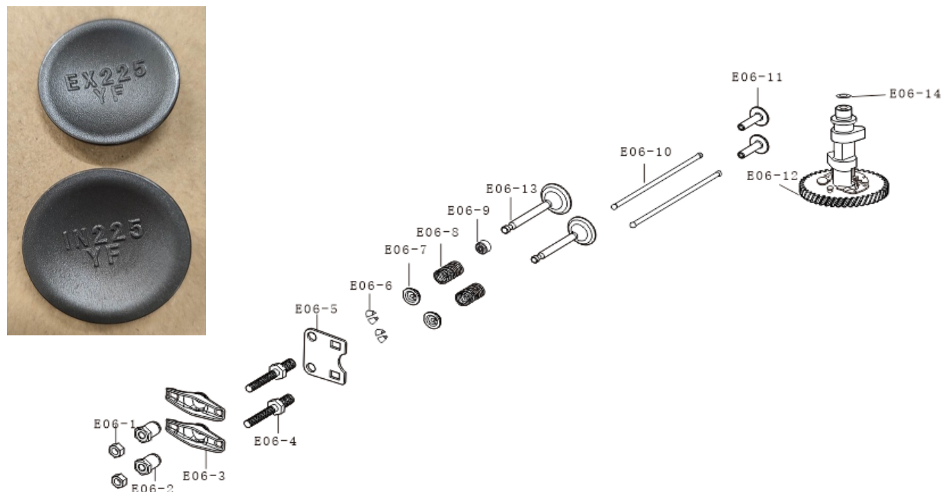
FIG.5 TRAIN,VALVE / CAMSHAFT SUBASSEMBLY. (E06)
