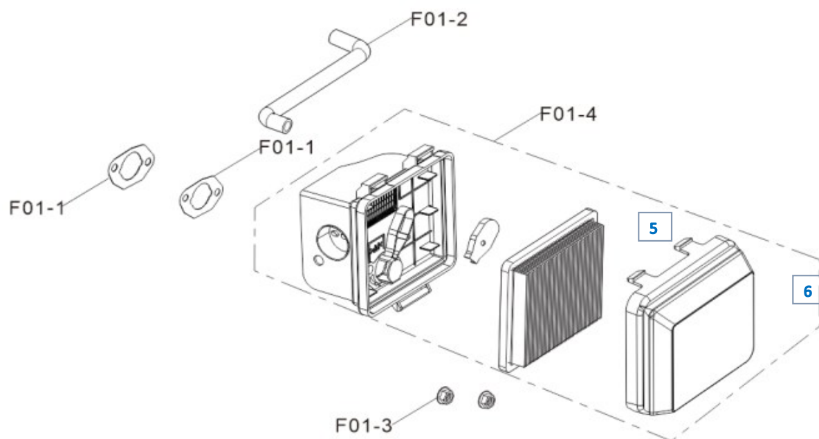
FIG.11 CLEANER, AIR. (F01)
