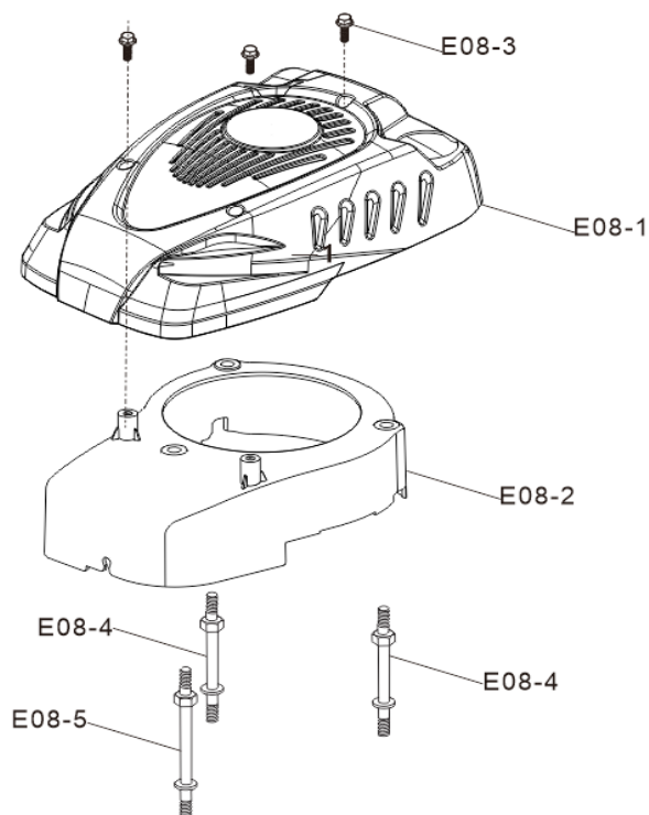
FIG.7 SHIELD,FAN. (E08)
