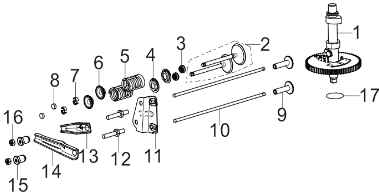
FIG.5 DISTRIBUTION - TRAIN VALVE / CAMSHAFT (E06)
