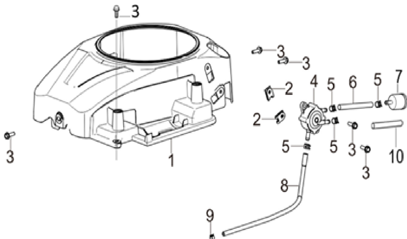
FIG.8 VOLUTE - SHROUD (E08)
