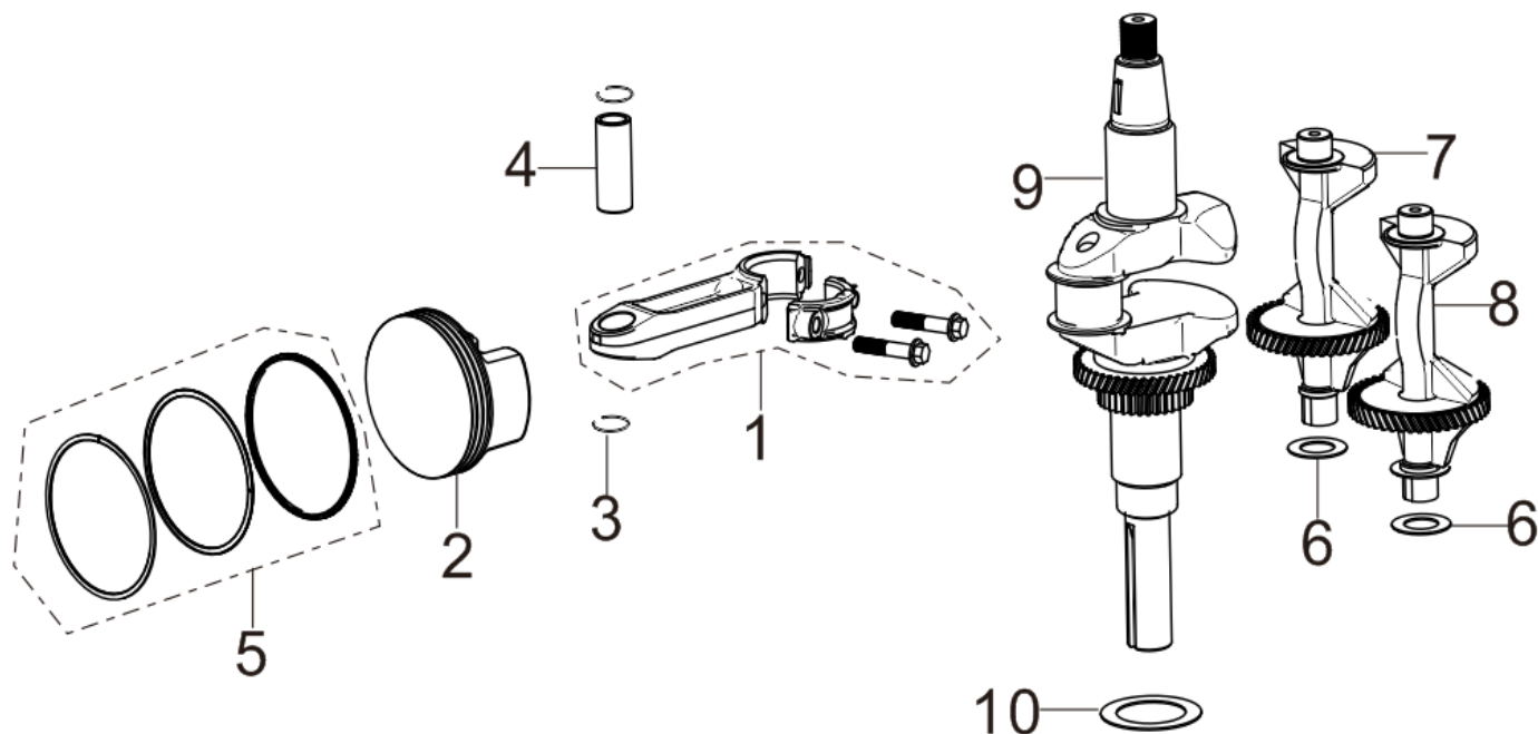
FIG.4 EMBIELLAGE - ROD,CRANKSHAFT (E04)
