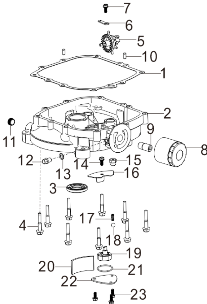
FIG.2 CARTER INFERIEUR - COVER CRANKCASE (E02)
