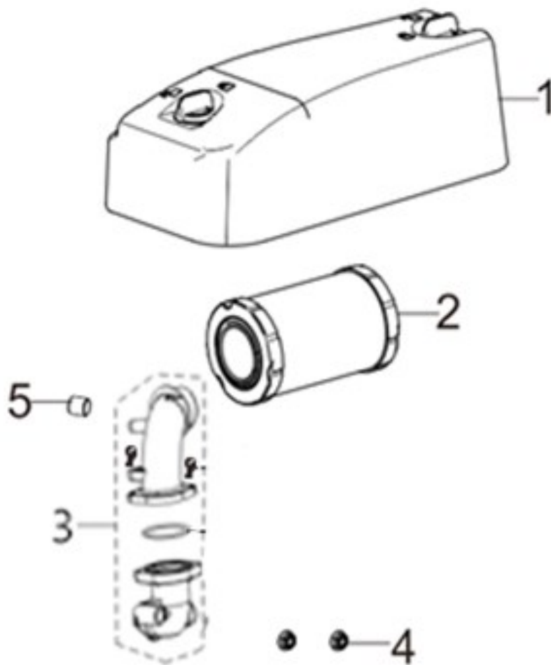
FIG.13 FILTRE A AIR - AIR CLEANER (F01)
