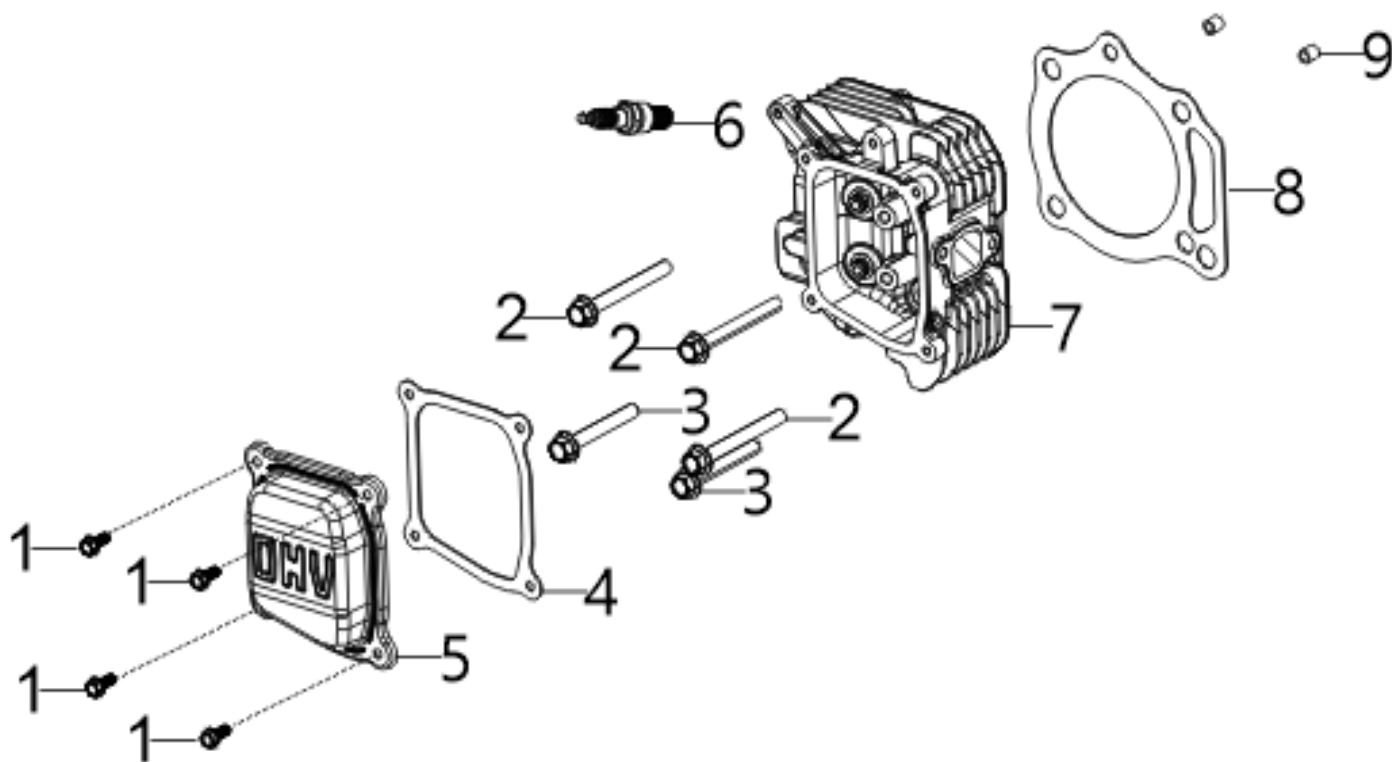
FIG.3 CULASSE - CYLINDER HEAD (E03)
