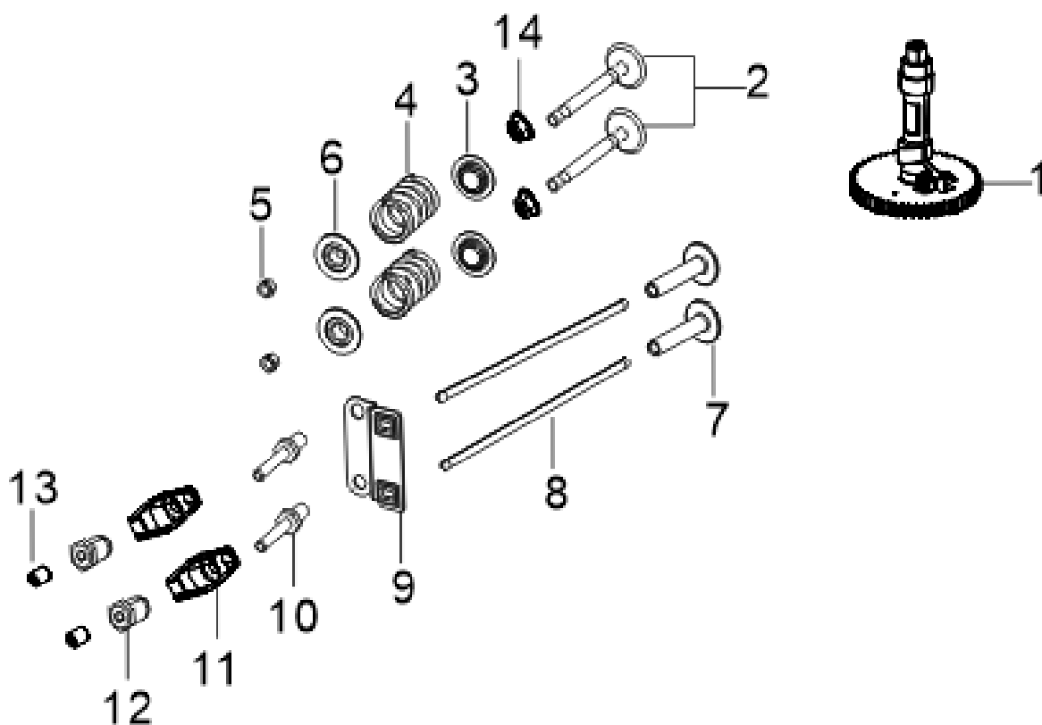
FIG.5 DISTRIBUTION - TRAIN,VALVE / CAMSHAFT (E06)
