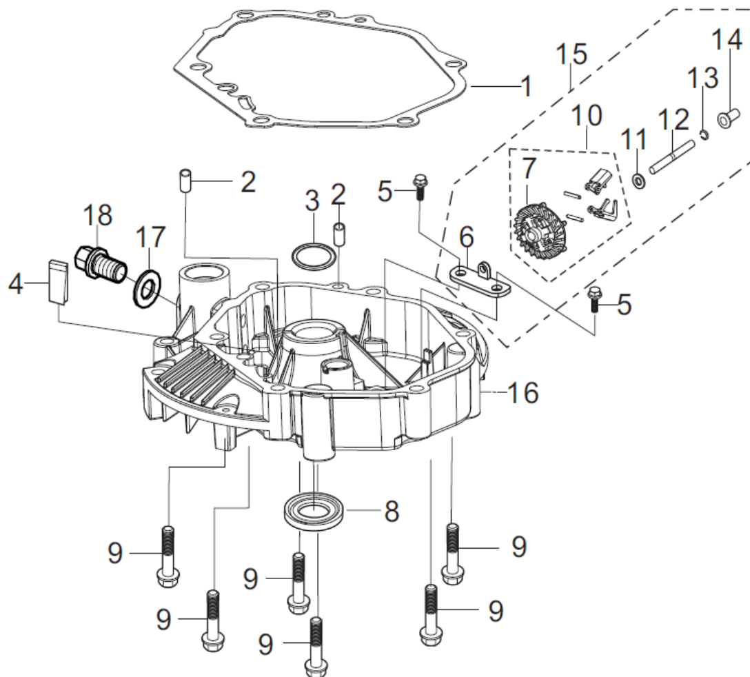
FIG.3 COVER SUBASSEMBLY, CRANKCASE / GEAR ASSY, GOVERNOR (E16)
