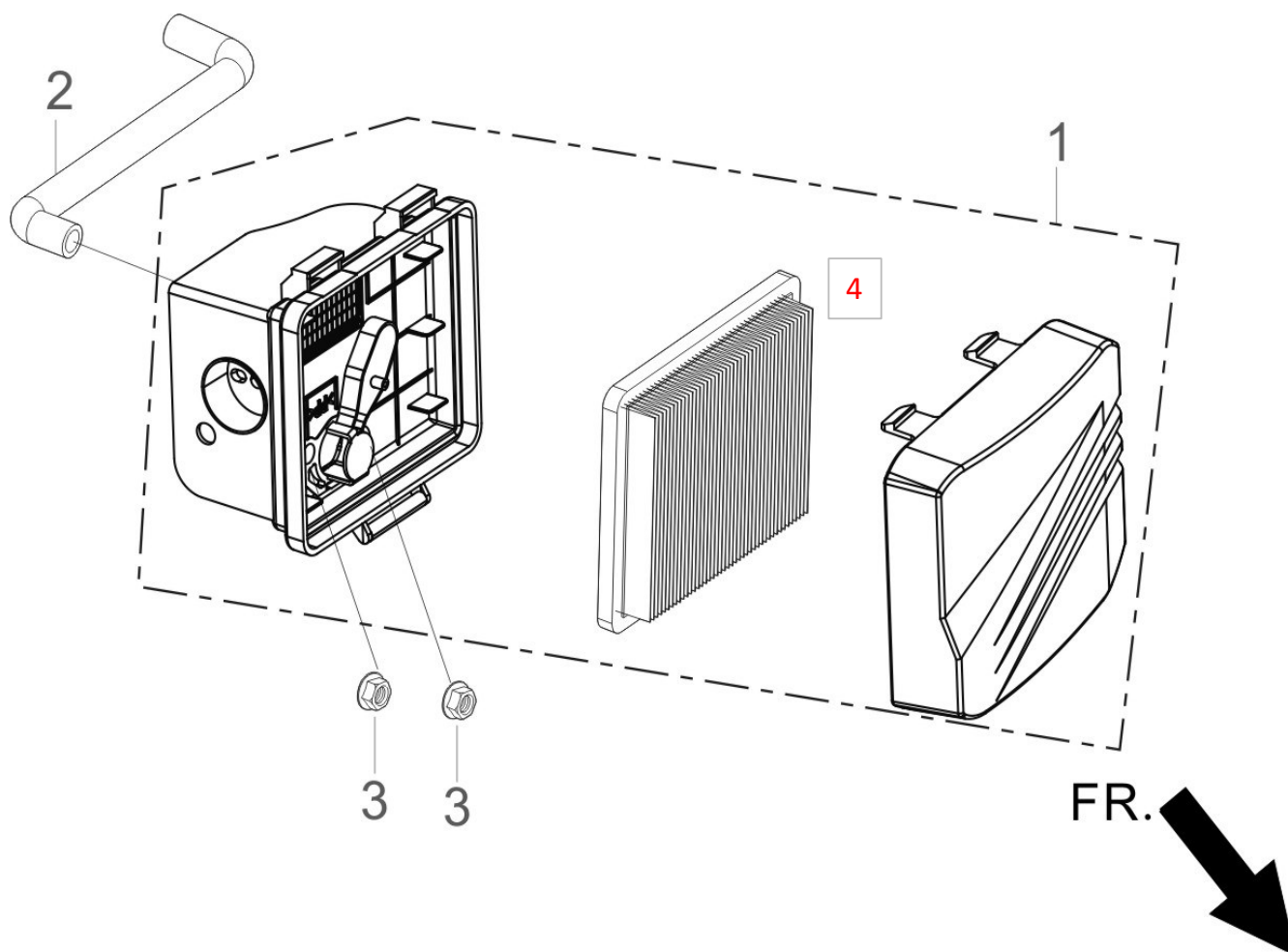
FIG.9 CLEANER, AIR (F02)
