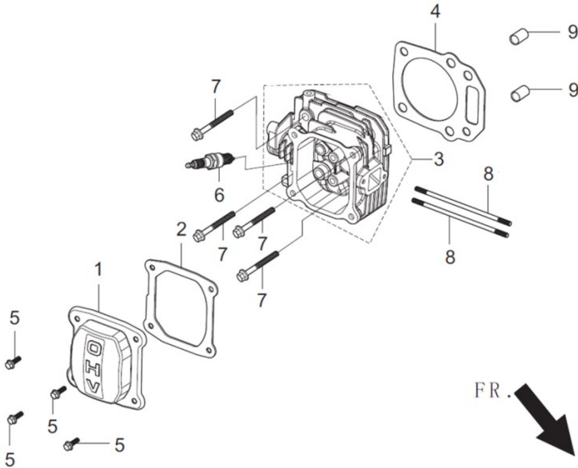
FIG.1 HEAD SUBASSEMBLY, CYLINDER / PLUG,SPARK (E04)
