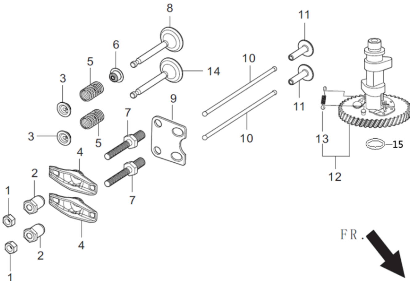
FIG.5 TRAIN,VALVE / CAMSHAFT SUBASSEMBLY (E05)
