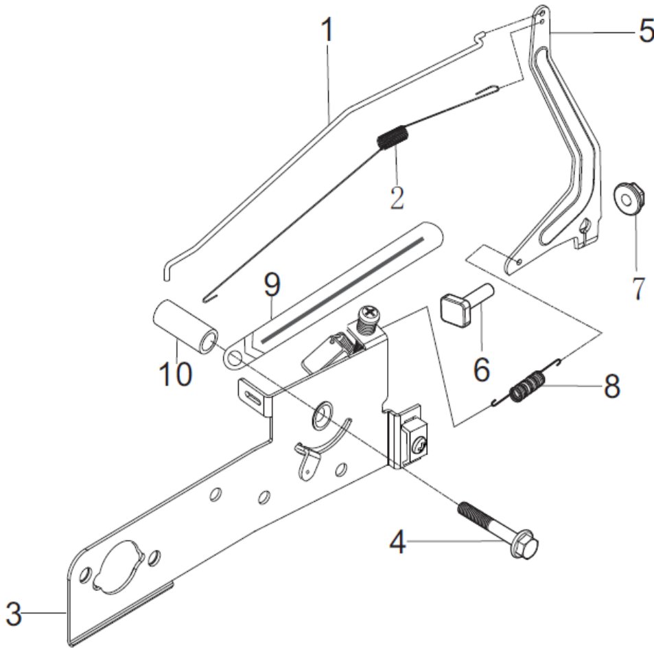
FIG.13 CONTROL ASSY, THROTTLE (E13)
