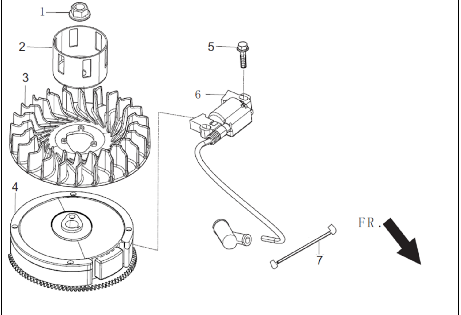
FIG.12 FLYWHEEL / IMPELLER / STARTER PULLEY / IGNITION COIL (E15)
