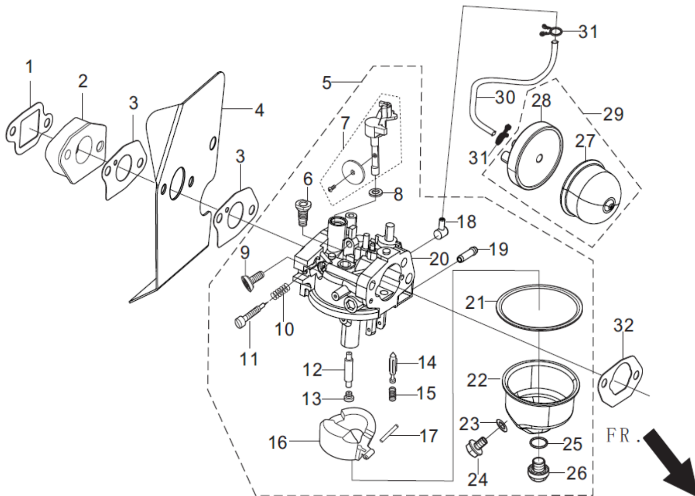
FIG.8 CARBURETOR ASSY. (E11)
