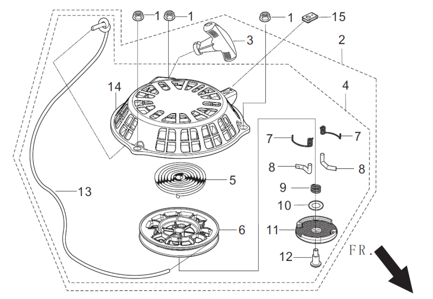
FIG.6 STARTER,RECOIL (E08)
