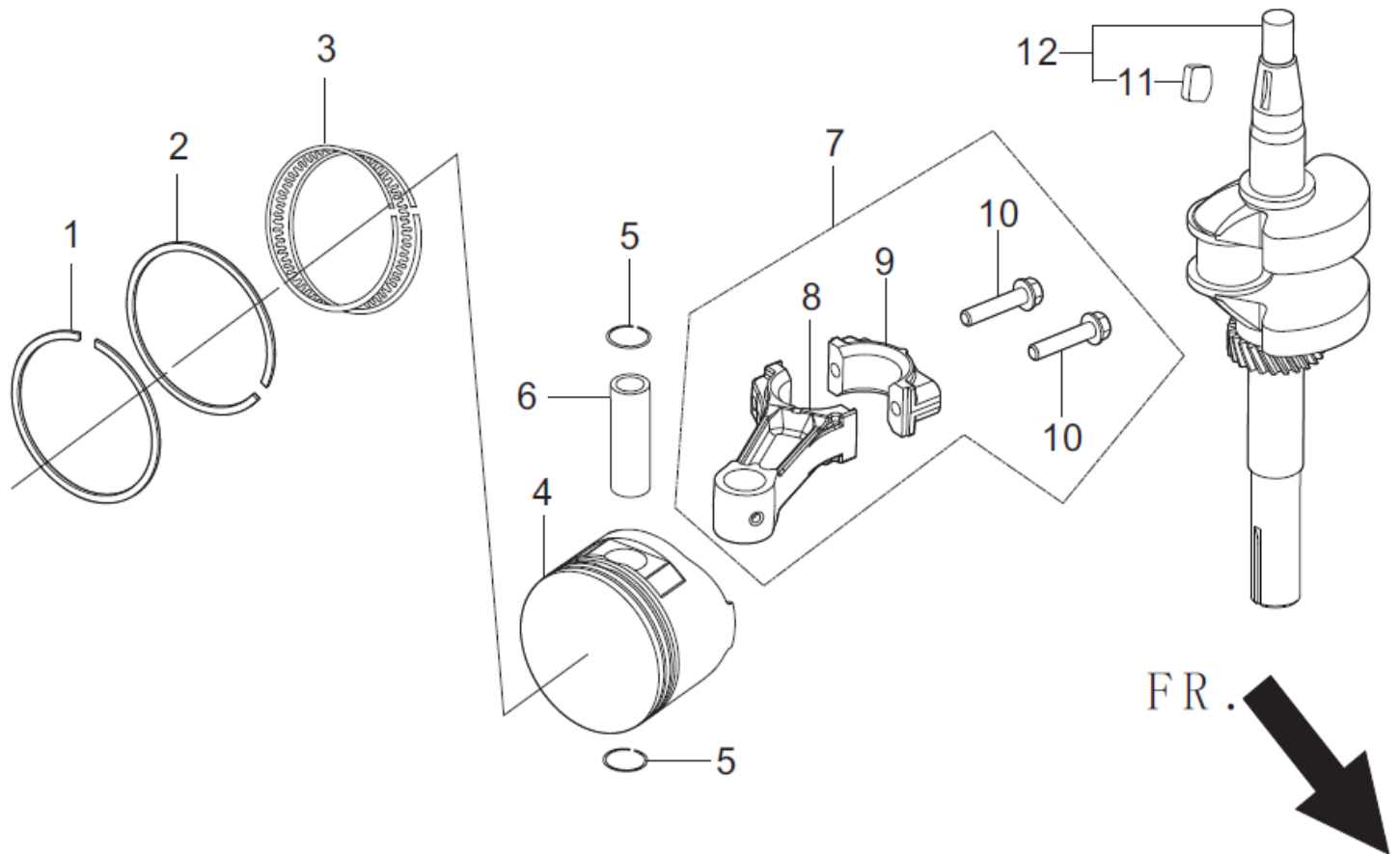
FIG.4 ROD,CRANKSHAFT CONNETING (E03)
