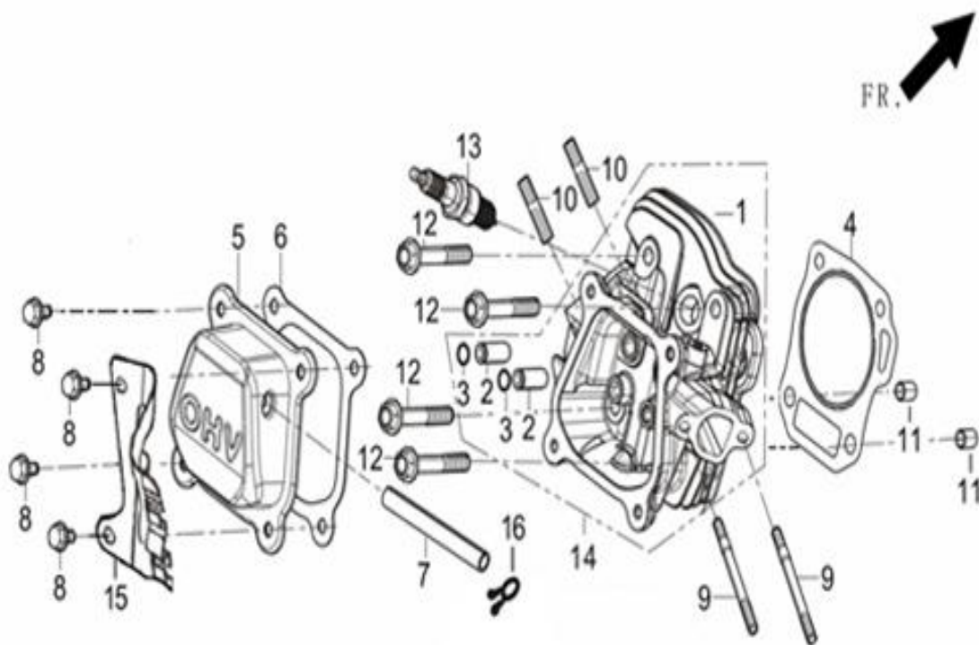
FIG.1 HEAD SUBASSEMBLY, CYLINDER / PLUG,SPARK(E04)
