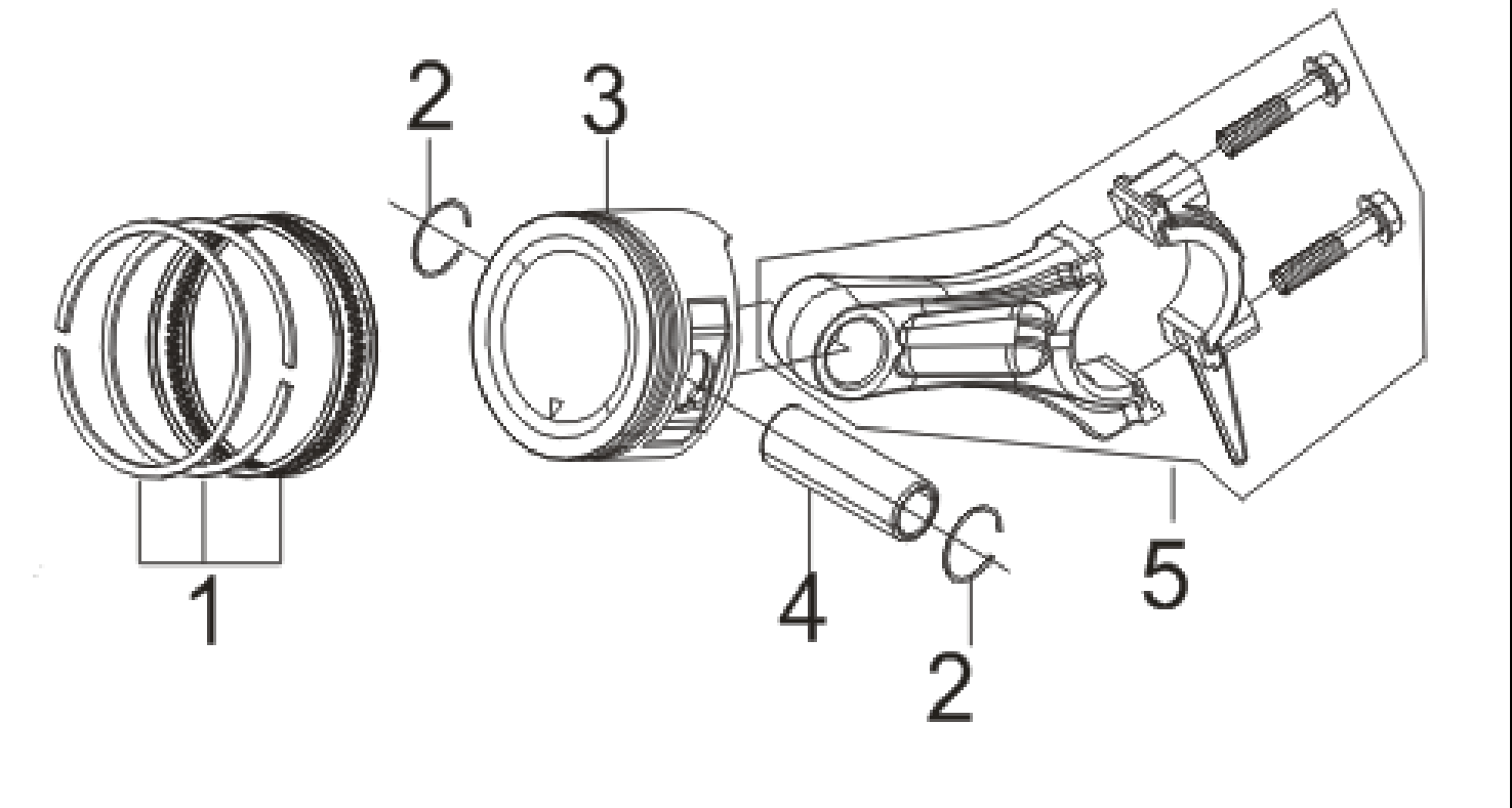
FIG.5 RING SET,OIL / ROD,CRANKSHAFT CONNETING (E03)
