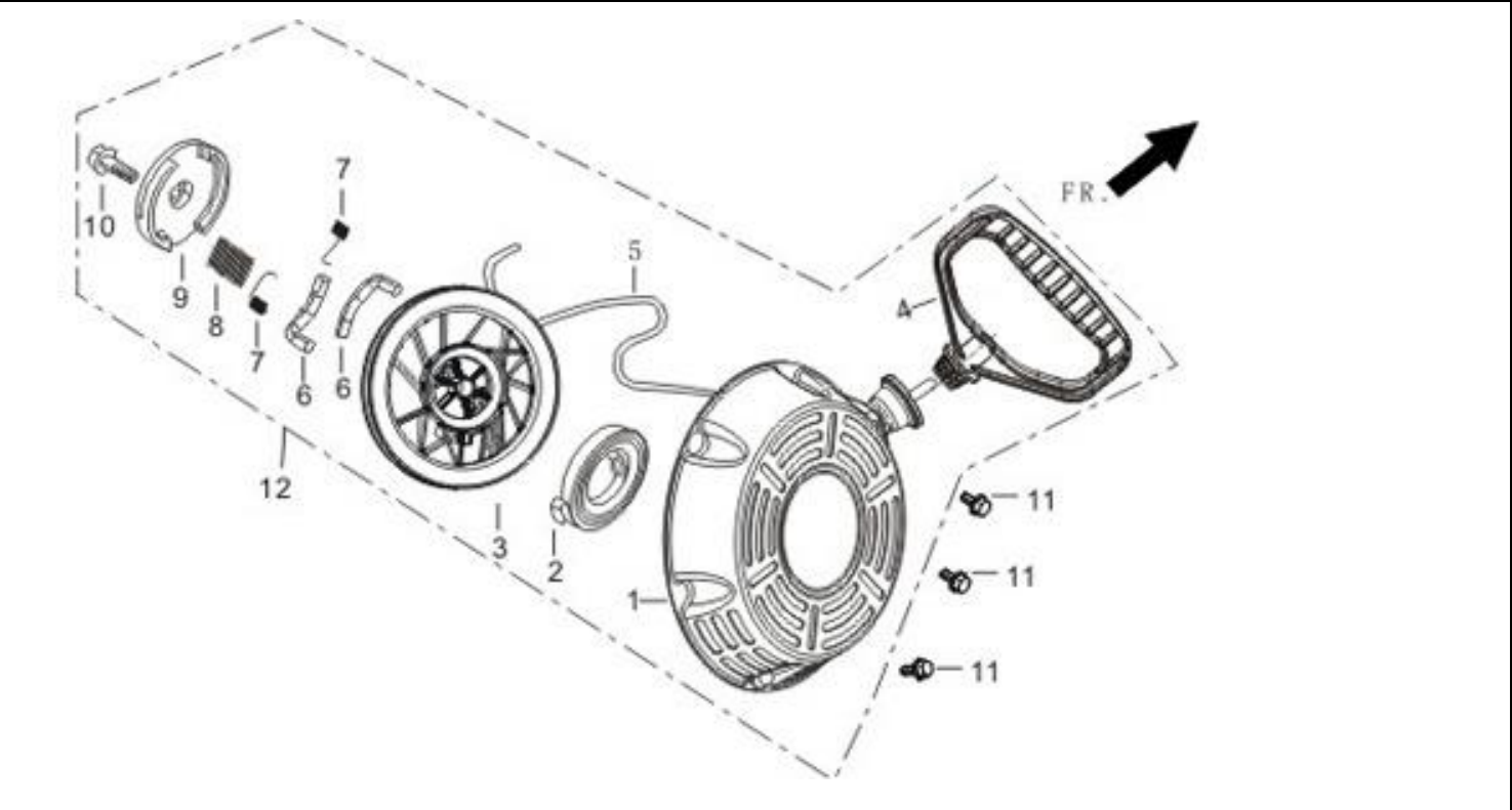
FIG.7 STARTER,RECOIL (E08)
