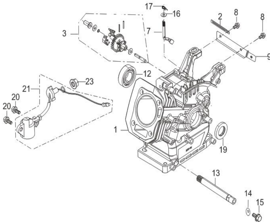
FIG.2 CRANKCASE. / GEAR ASSY, GOVERNOR.(E17)
