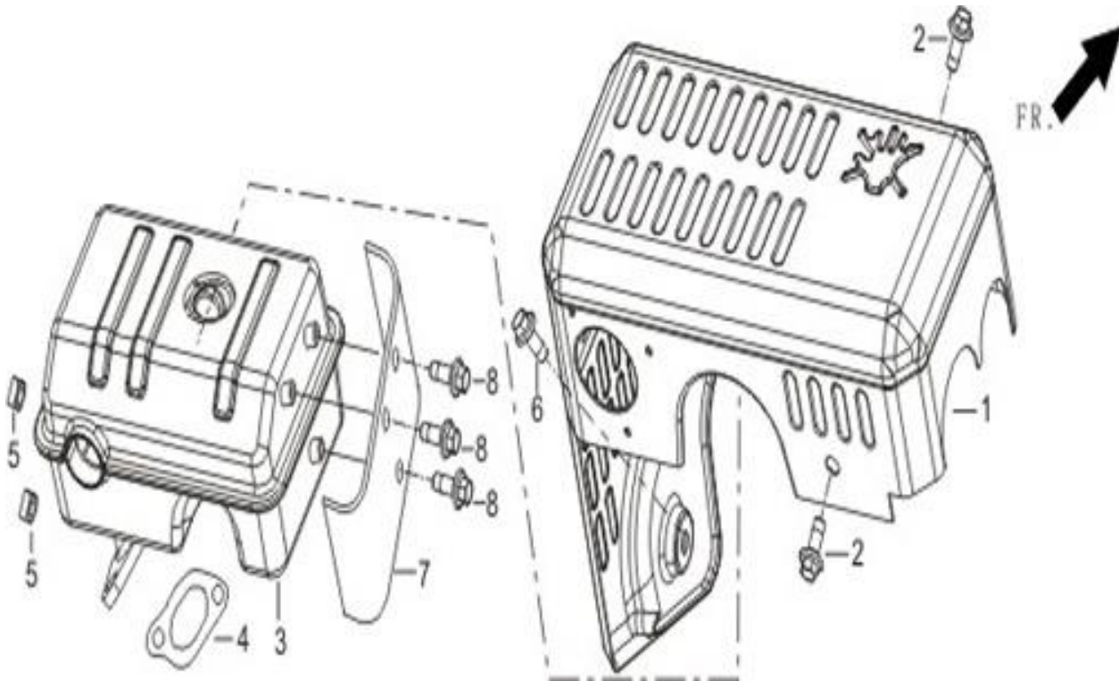
FIG.12 MUFFLER ASSY. (F04)
