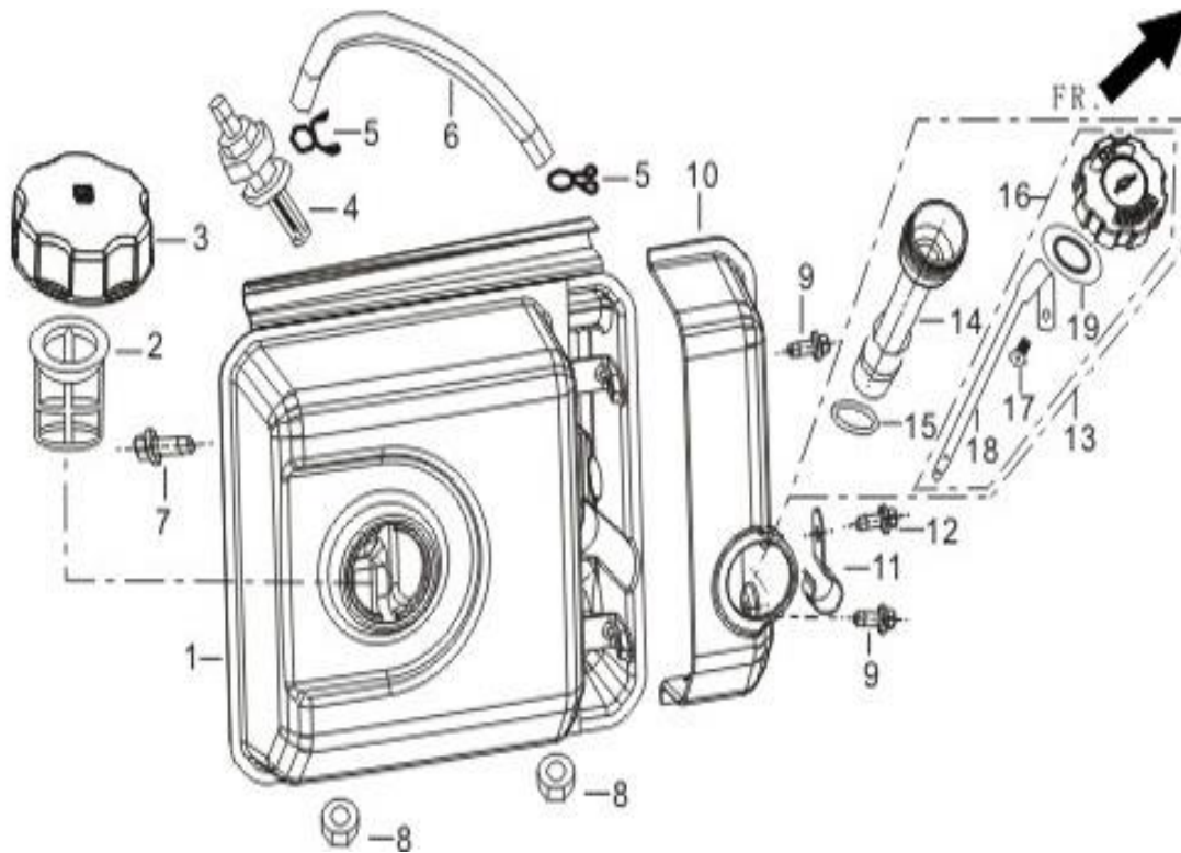
FIG.13 TANK ASSY, FUEL (F01)
