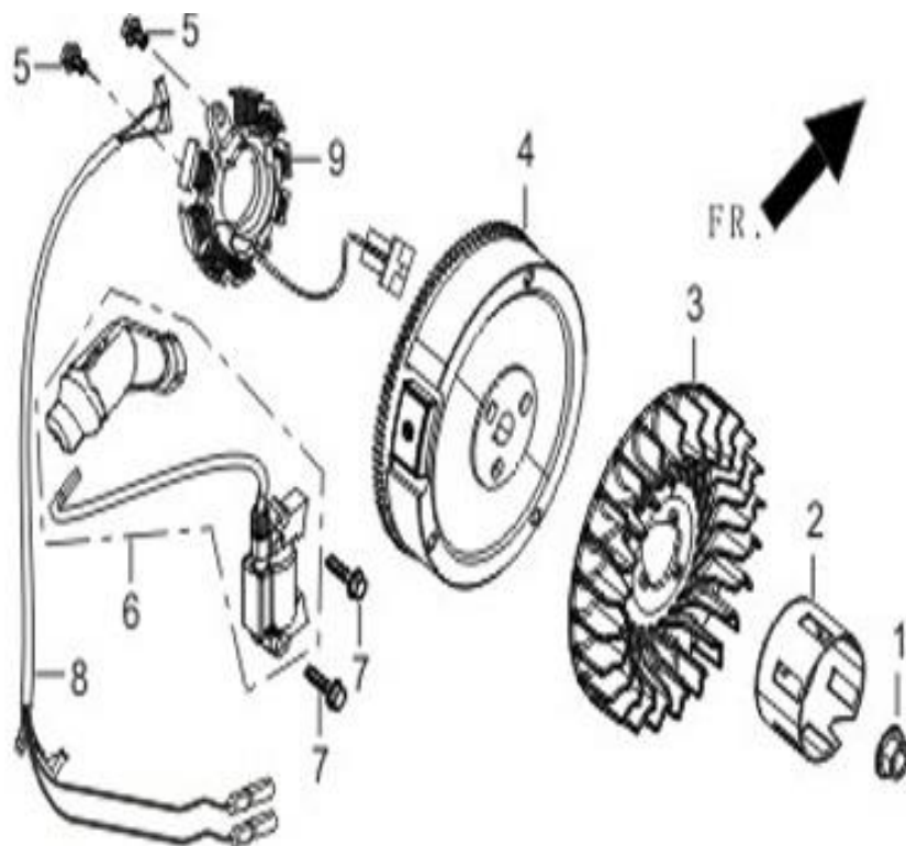
FIG.14 FLYWHEEL / IMPELLER / STARTER PULLEY / IGNITION COIL (E15)
