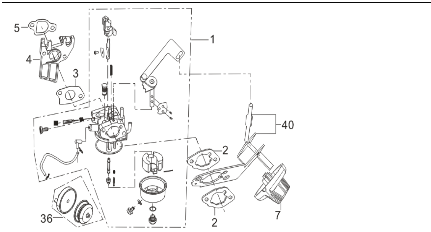
FIG.10 CARBURETOR ASSY. (E11)
