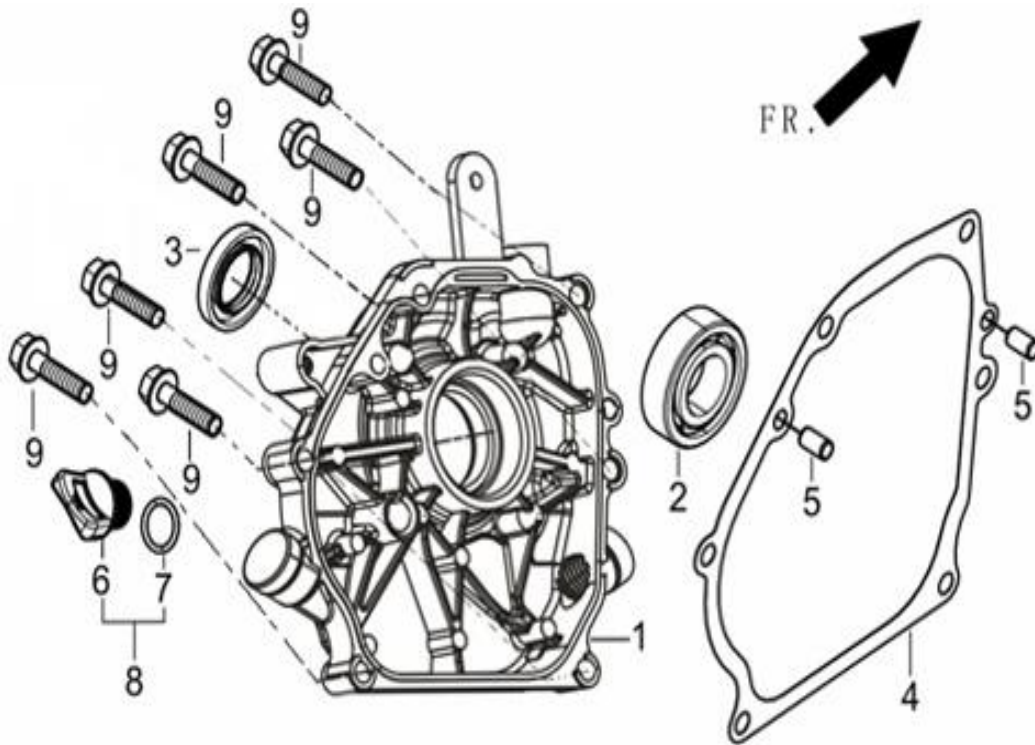
FIG.3 COVER SUBASSEMBLY, CRANKCASE (E01)
