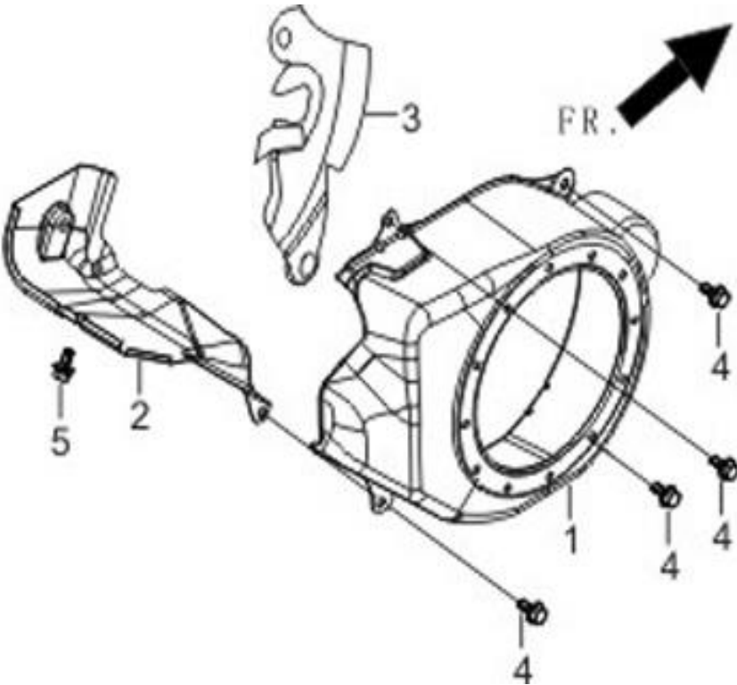
FIG.9 SHROUD / SHIELD,LOWER (E14)
