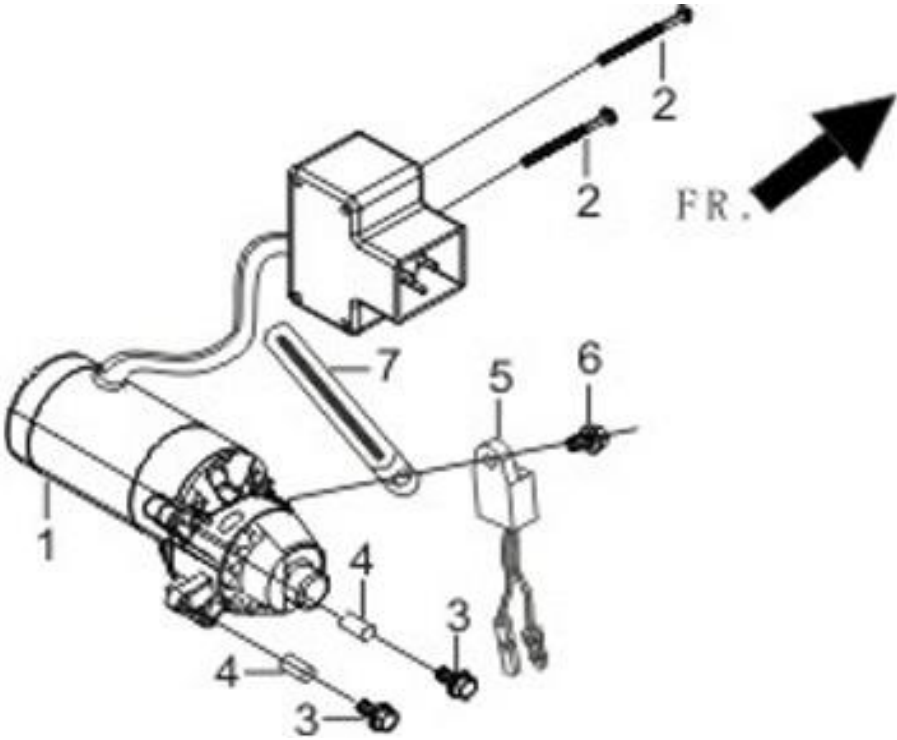
FIG.8 START-UP ELECTRIC MACHINE COMPONENTS (E09)
