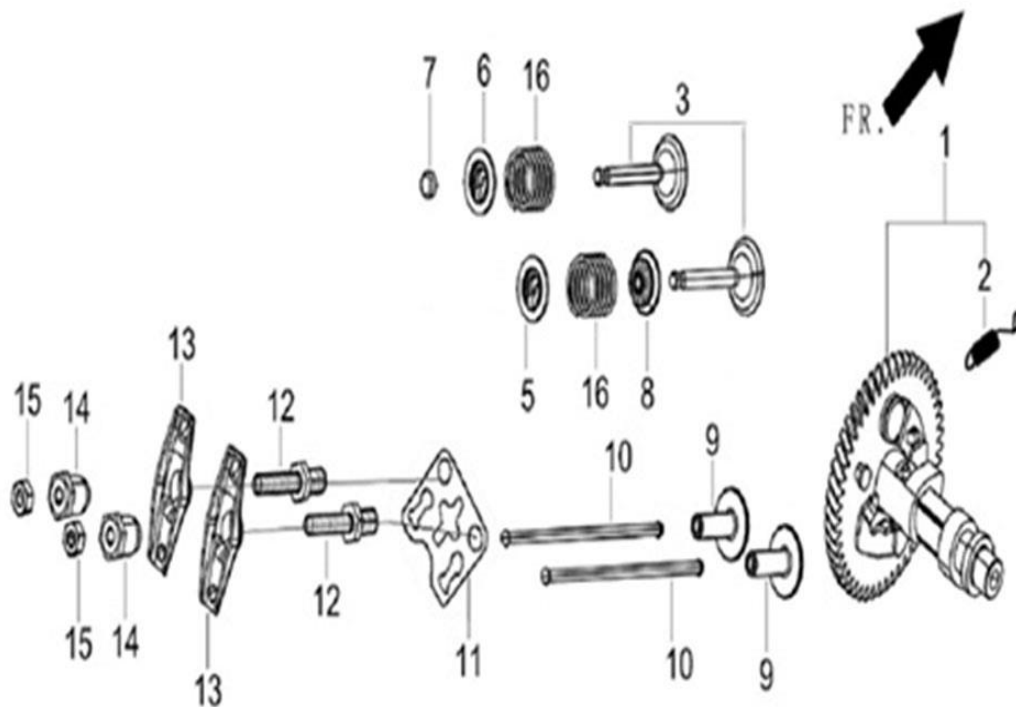
FIG.6 TRAIN,VALVE / CAMSHAFT SUBASSEMBLY (E05)
