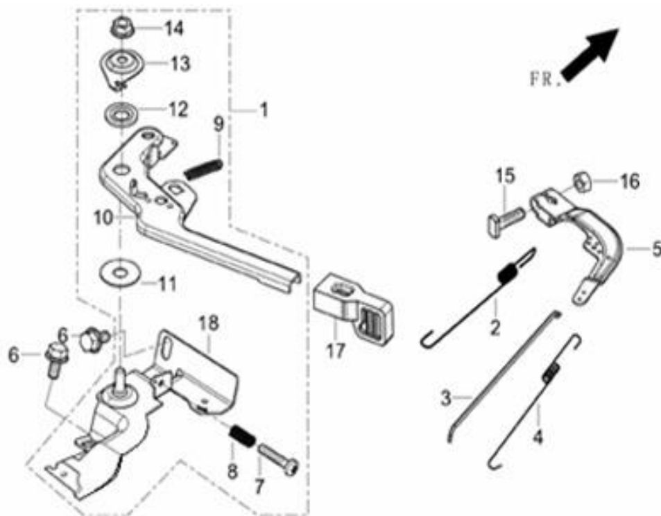
FIG.15 CONTROL ASSY, THROTTLE (E13)
