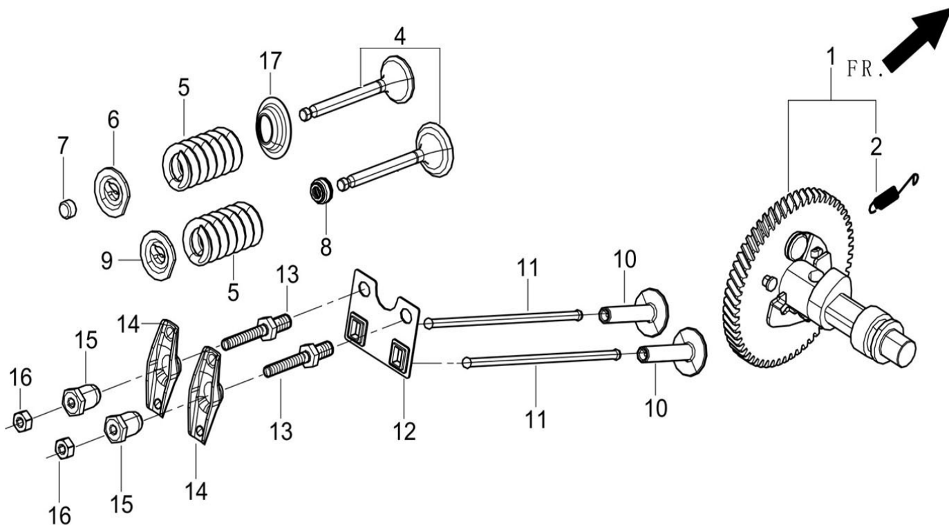
FIG.6 TRAIN,VALVE / CAMSHAFT SUBASSEMBLY (E06)
