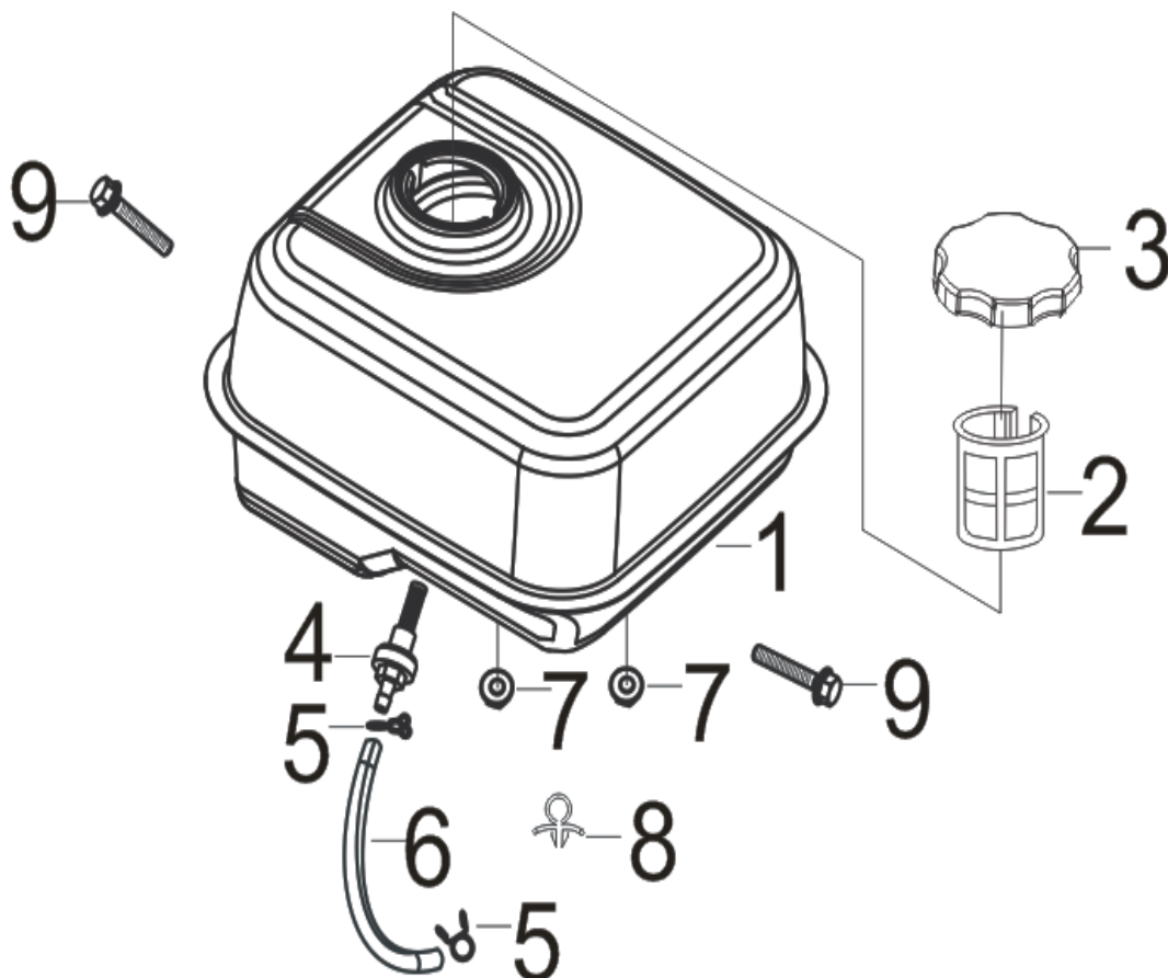
FIG.14 TANK ASSY, FUEL (F03)
