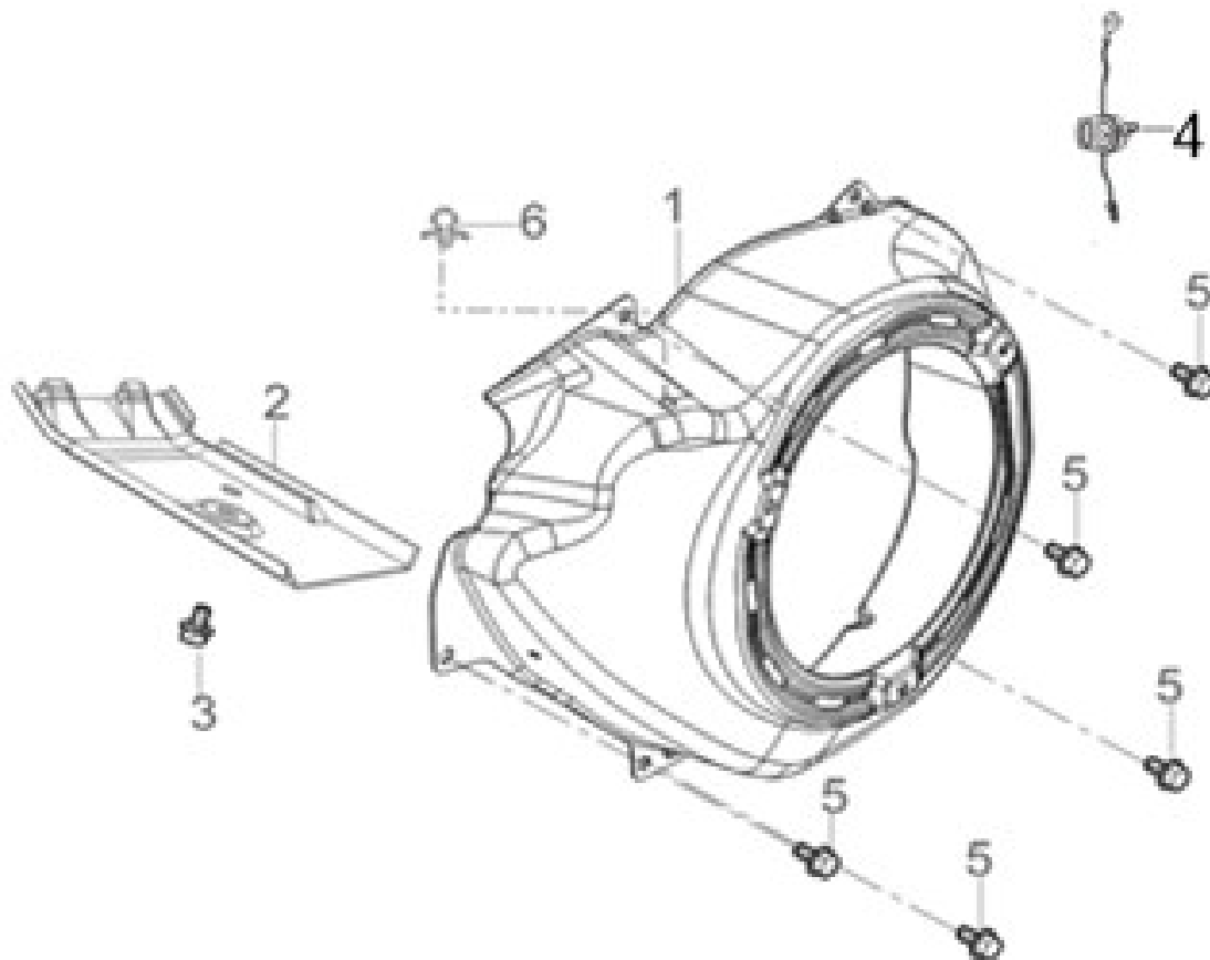
FIG.8 SHROUD / SHIELD,LOWER (E08)
