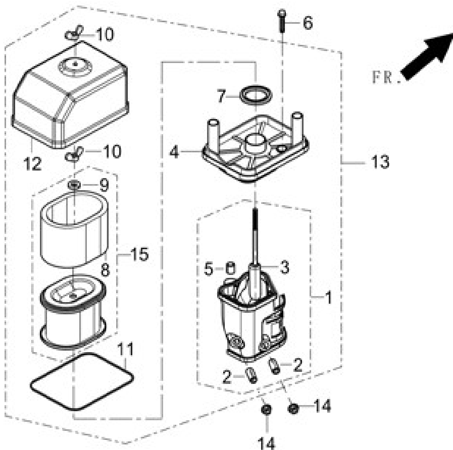
FIG.12 CLEANER, AIR (F01)
