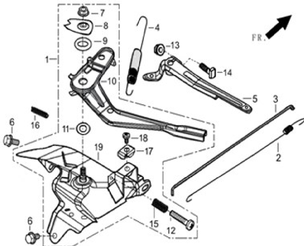
FIG.11 CONTROL ASSY, THROTTLE (E11)
