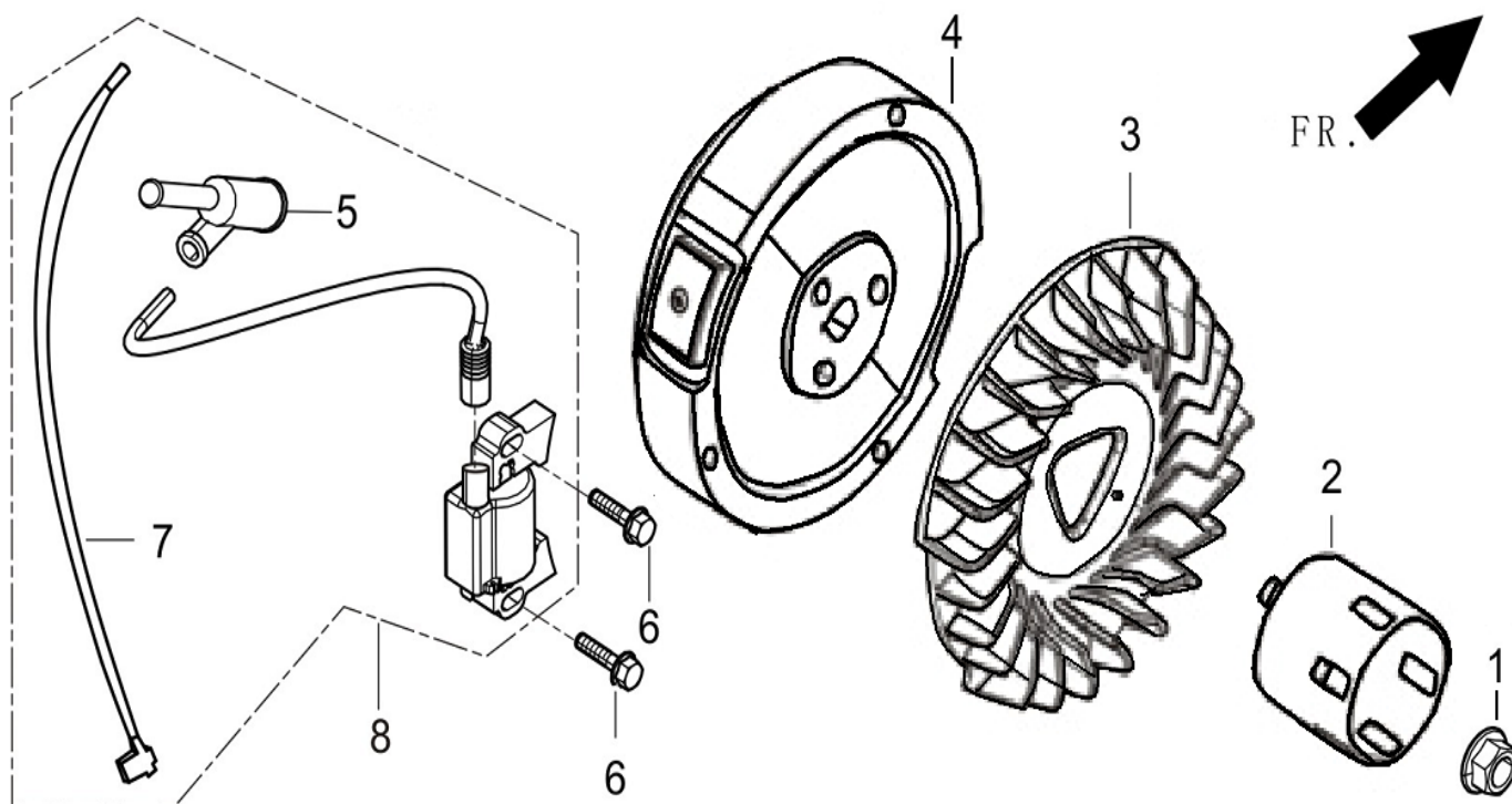
FIG.10 FLYWHEEL / IMPELLER / STARTER PULLEY / IGNITION COIL (E10)
