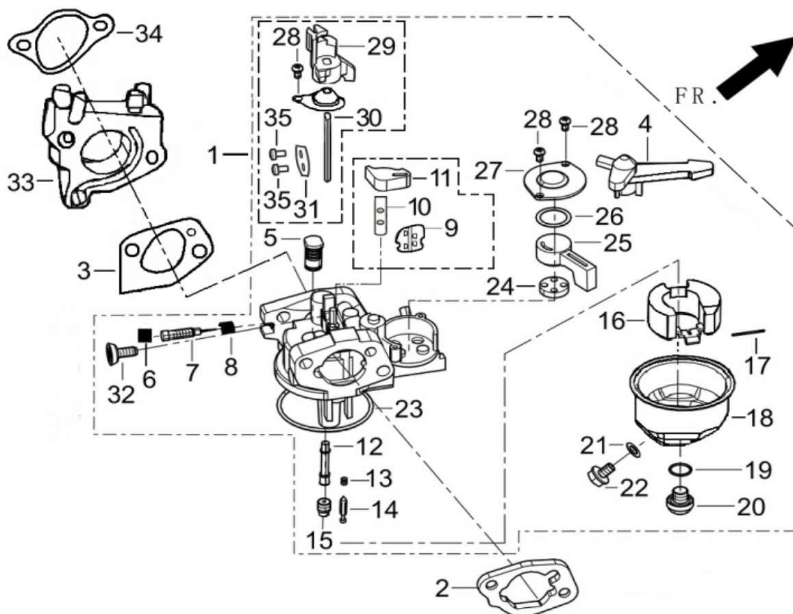
FIG.9 CARBURETOR ASSY. (E09)
