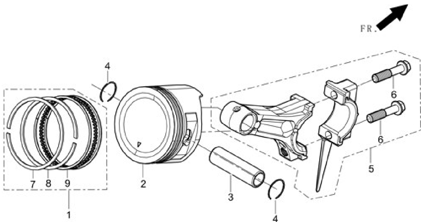
FIG.5 RING SET,OIL / ROD,CRANKSHAFT CONNETING (E05)
