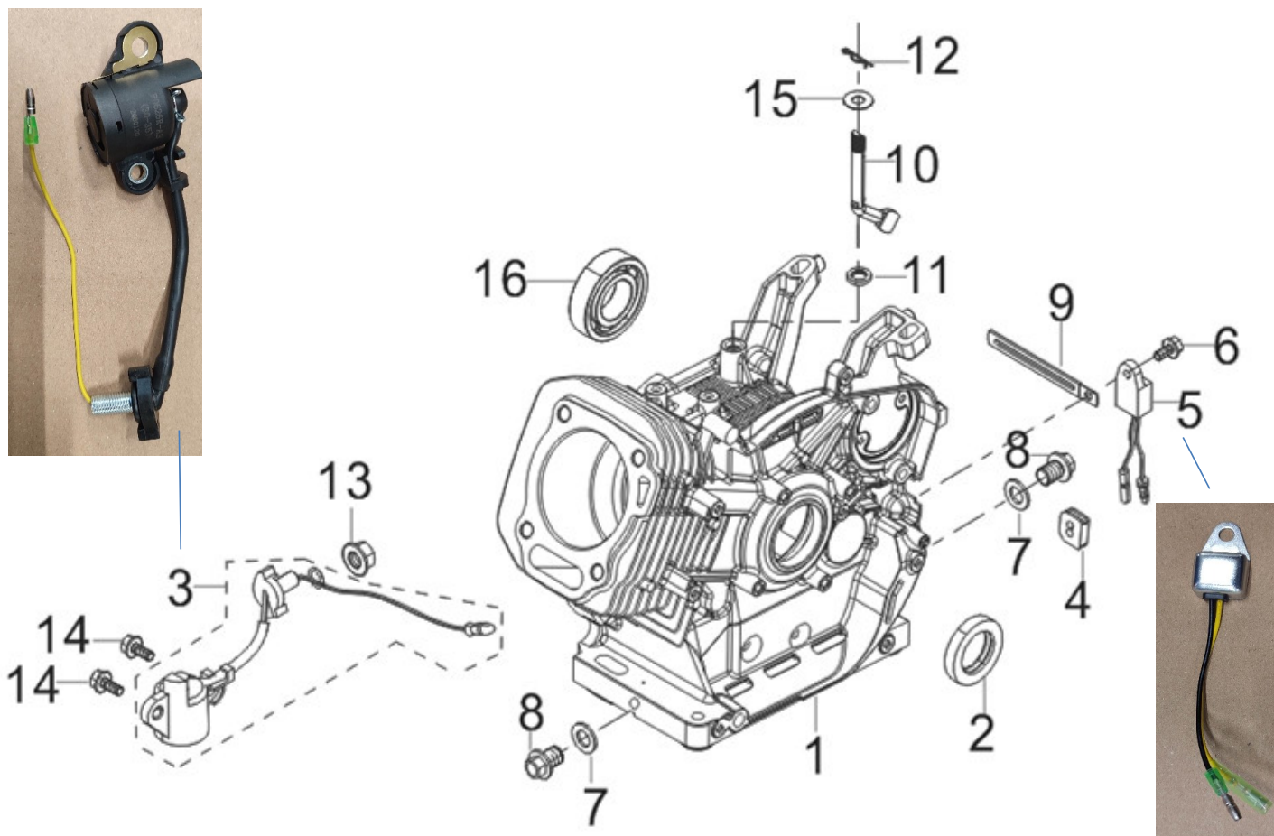
FIG.1 CRANKCASE. / GEAR ASSY, GOVERNOR
