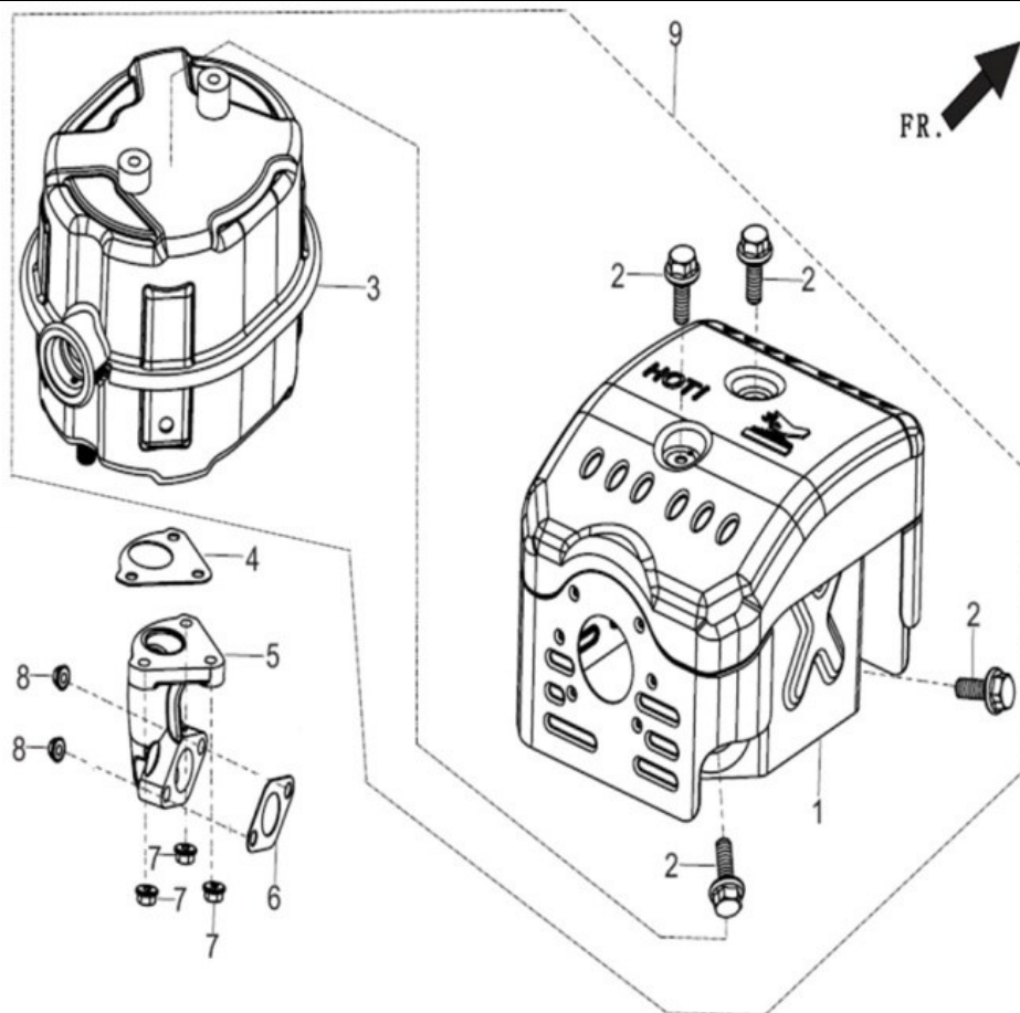
FIG.13 MUFFLER ASSY. (F02)
