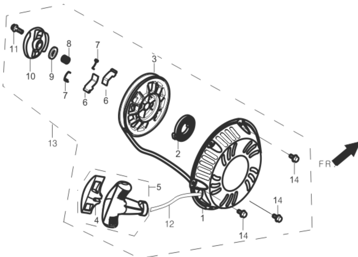
FIG.7 STARTER,RECOIL (E07)
