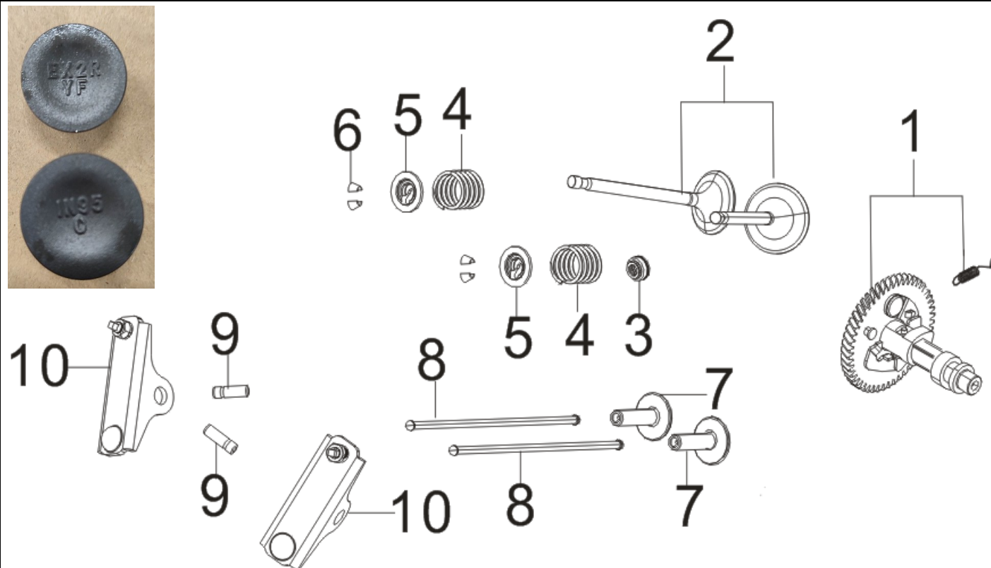
FIG.6 TRAIN,VALVE / CAMSHAFT SUBASSEMBLY (E06)
