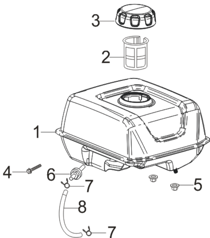
FIG.14 TANK ASSY, FUEL (F03)
