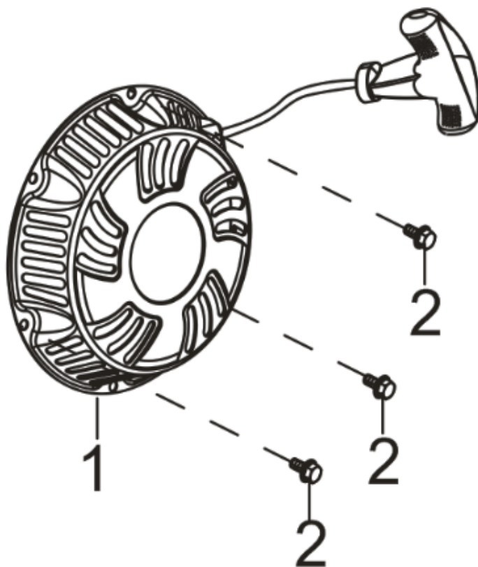
FIG.7 STARTER,RECOIL (E07)
