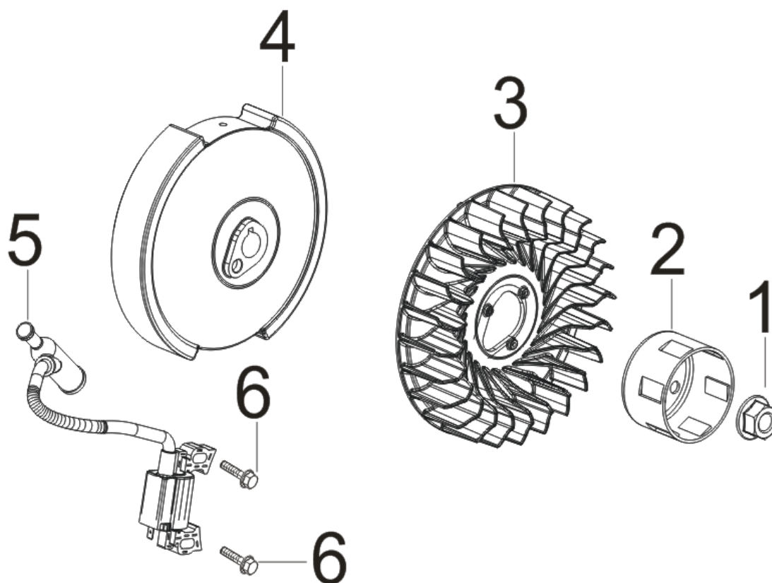
FIG.10 FLYWHEEL / IMPELLER / STARTER PULLEY / IGNITION COIL (E10)
