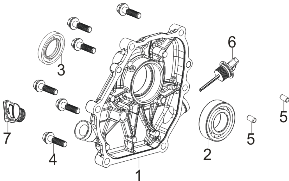
FIG.2 COVER SUBASSEMBLY, CRANKCASE (E02)
