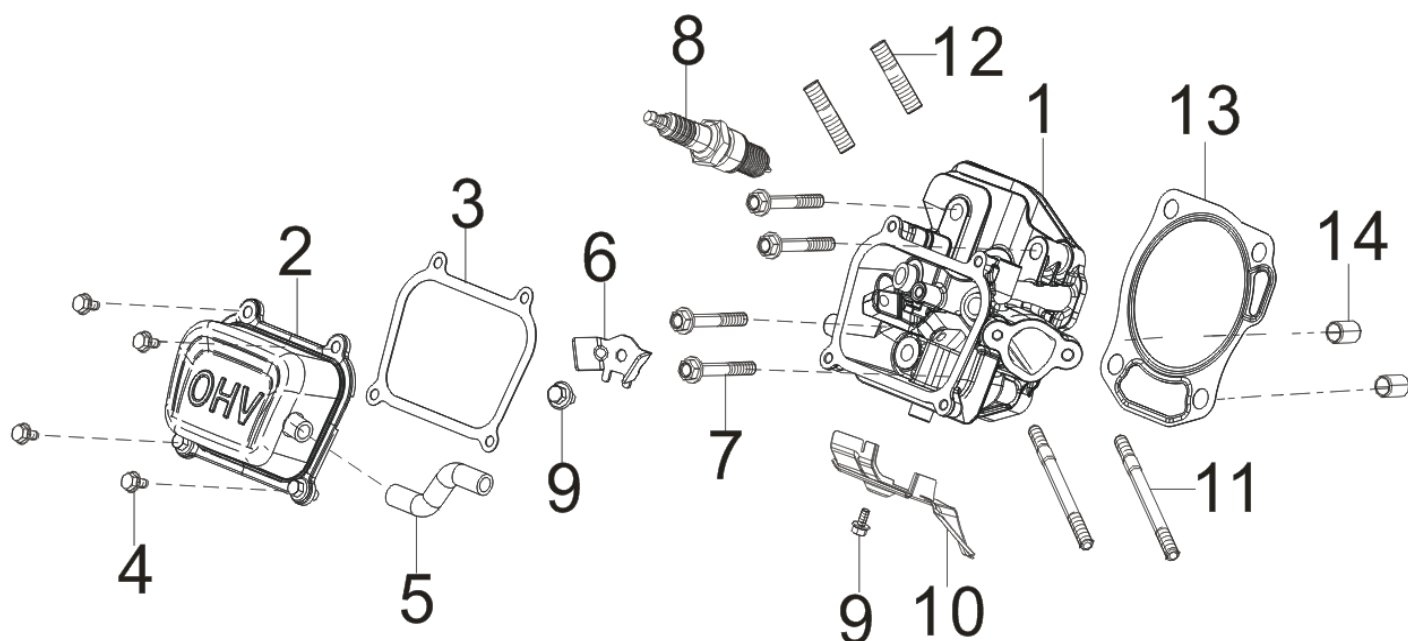
FIG.3 HEAD SUBASSEMBLY, CYLINDER / PLUG,SPARK (E03)
