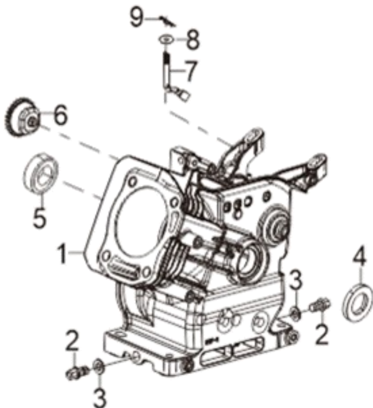
FIG.1 CRANKCASE. / GEAR ASSY, GOVERNOR (E01)
