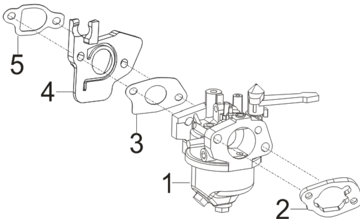
FIG.9 CARBURETOR ASSY. (E09)
