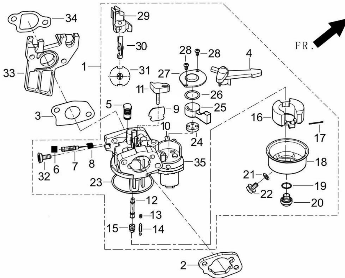
FIG.9 CARBURETOR ASSY. (E11)
