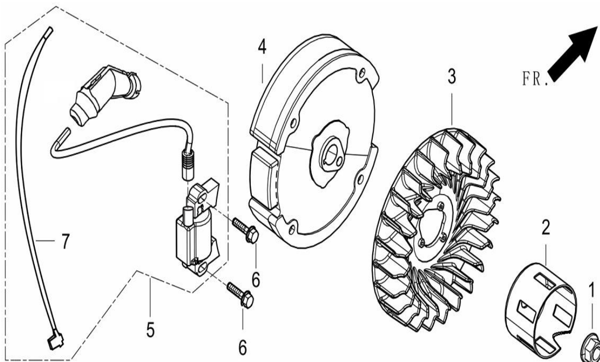
FIG.13 FLYWHEEL / IMPELLER / STARTER PULLEY / IGNITION COIL (E15)
