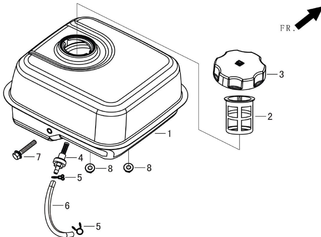
FIG.12 TANK ASSY, FUEL (F01)
