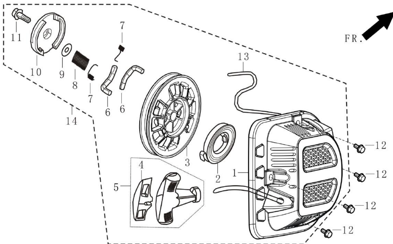
FIG.7 STARTER,RECOIL (E08)
