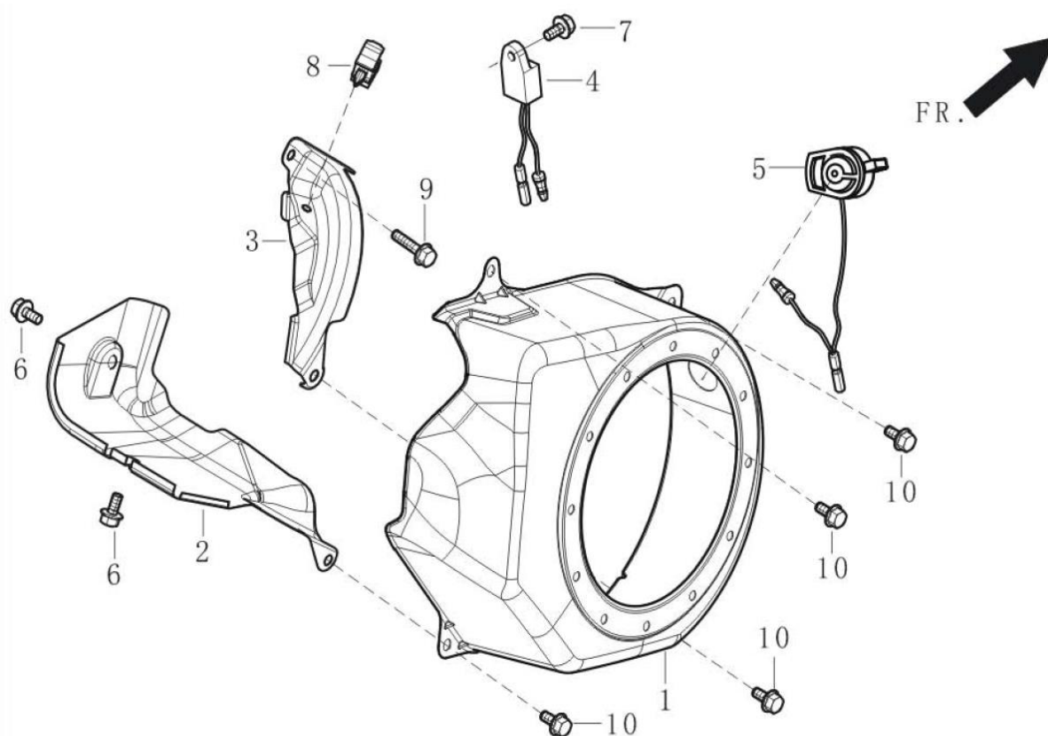
FIG.8 SHROUD / SHIELD,LOWER (E14)
