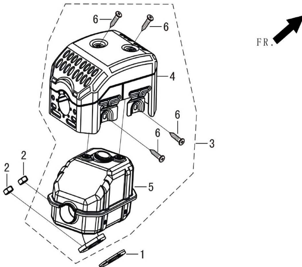
FIG.11 MUFFLER ASSY. (F04)
