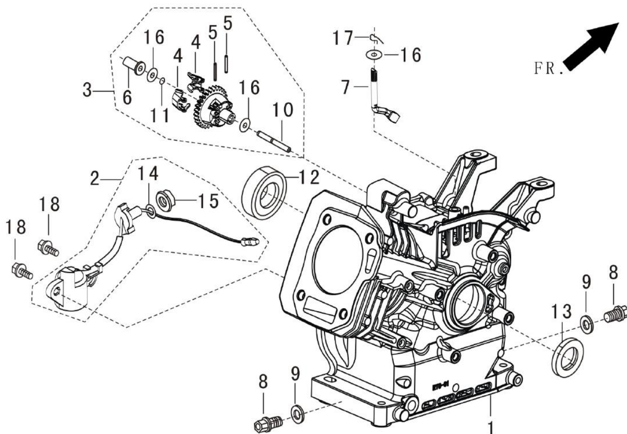
FIG.2 CRANKCASE. / GEAR ASSY, GOVERNOR (E17)
