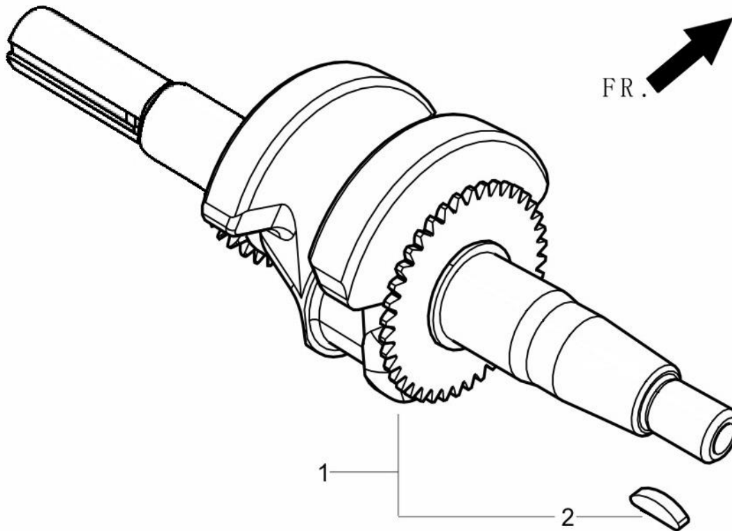
FIG.4 ROD,CRANKSHAFT CONNETING (E03)
