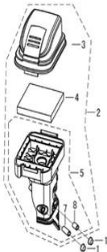
FIG.10 CLEANER, AIR (F02)
