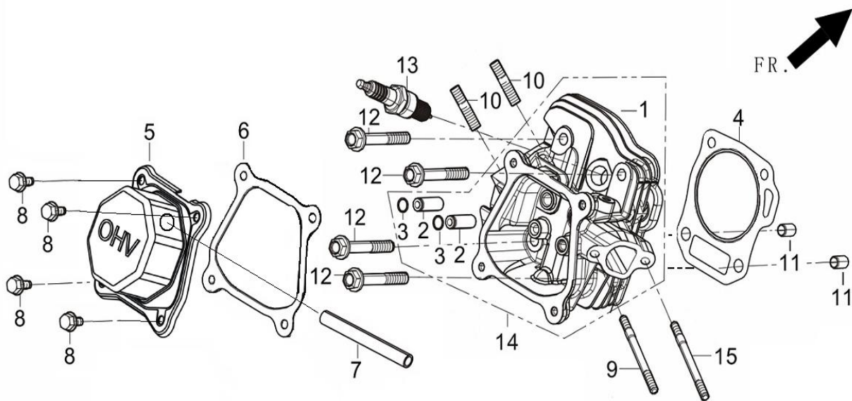
FIG.1 HEAD SUBASSEMBLY, CYLINDER / PLUG,SPARK (E04)
