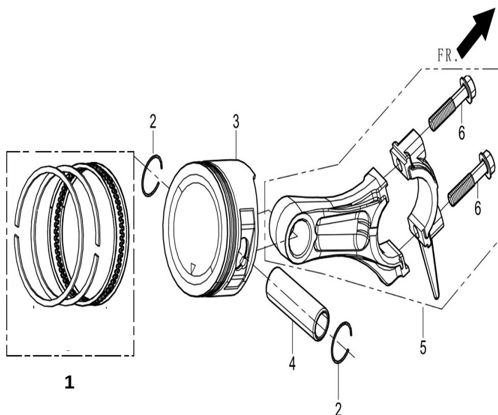
FIG.5 RING SET,OIL / ROD,CRANKSHAFT CONNETING (E04)
