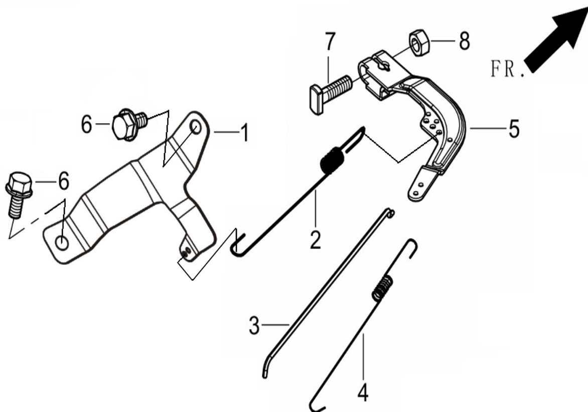
FIG.14 CONTROL ASSY, THROTTLE (E13)
