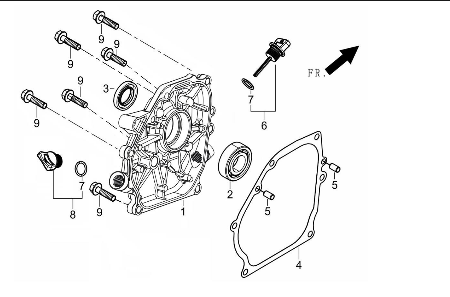
FIG.3 COVER SUBASSEMBLY, CRANKCASE (E01)
