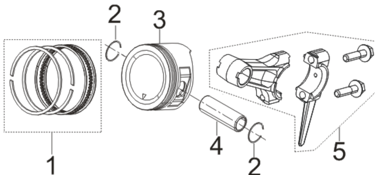
FIG.5 RING SET,OIL / ROD,CRANKSHAFT CONNECTING
