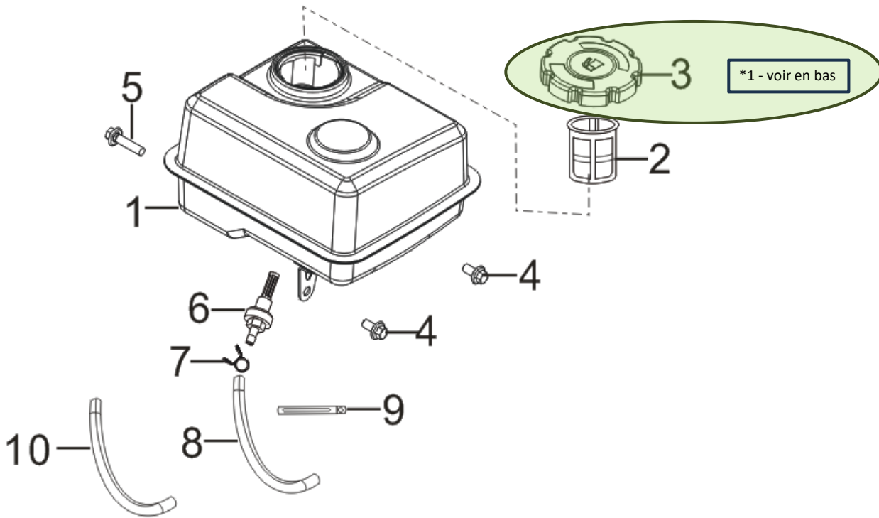
FIG.14 TANK ASSY, FUEL
