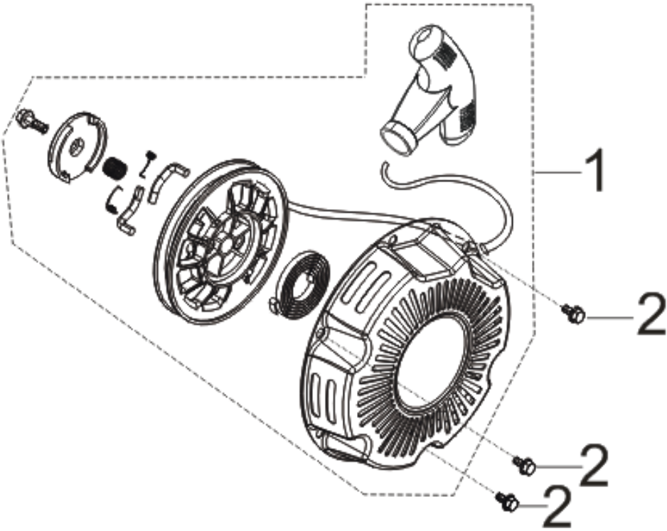
FIG.7 STARTER,RECOIL
