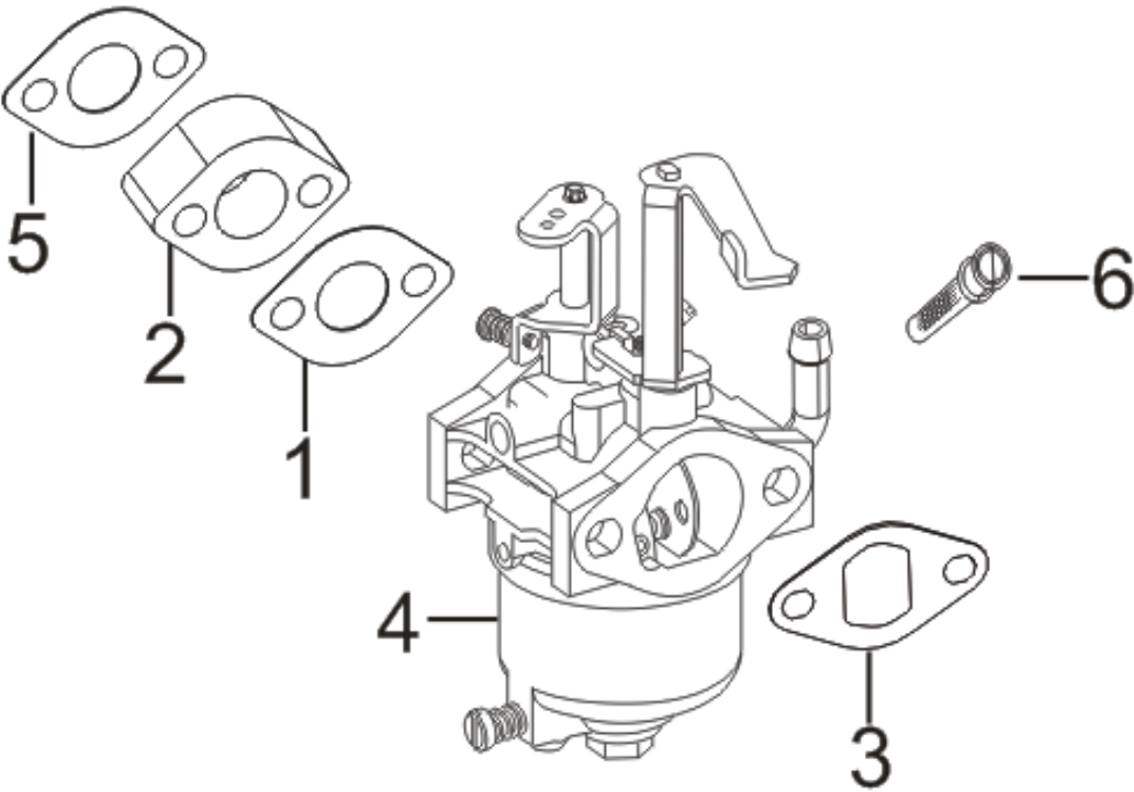
FIG.9 CARBURETOR ASSY.
