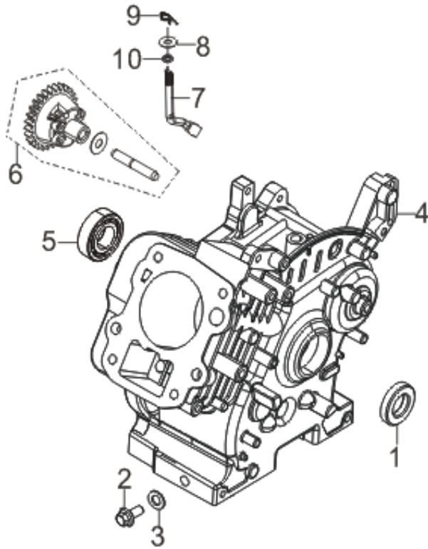
FIG.1 CRANKCASE. / GEAR ASSY, GOVERNOR.
