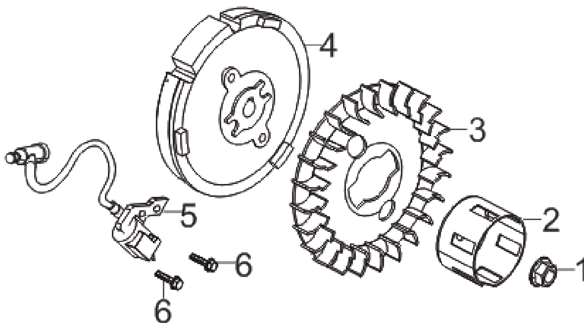
FIG.10 FLYWHEEL / IMPELLER / STARTER PULLEY / IGNITION COIL
