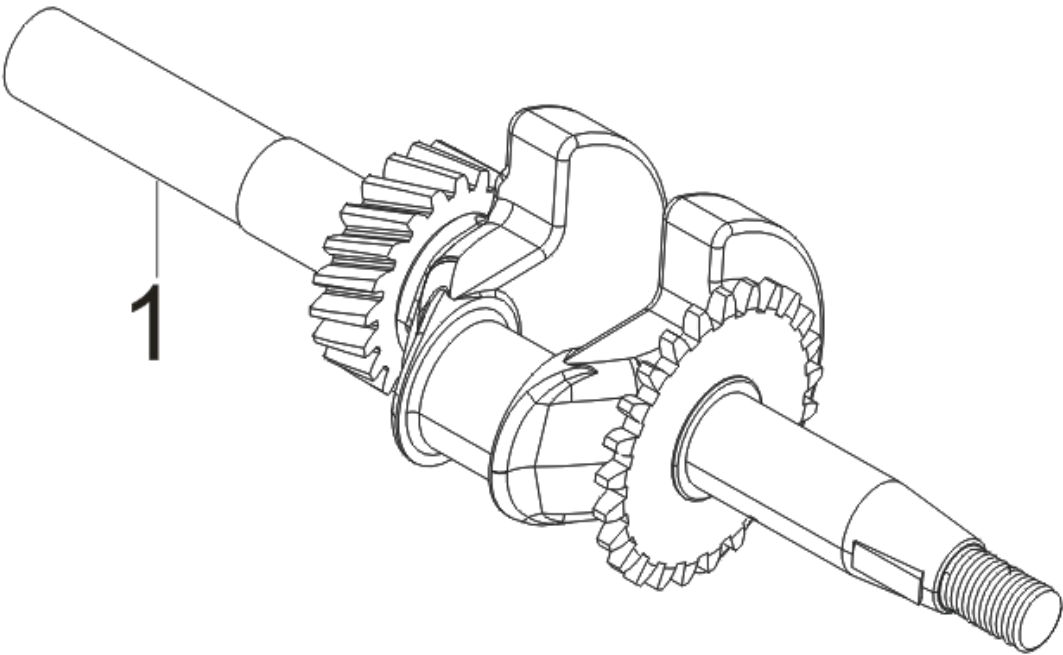
FIG.4 ROD,CRANKSHAFT CONNECTING
