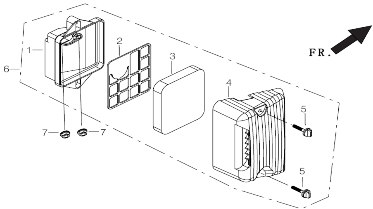
FIG.12 CLEANER, AIR
