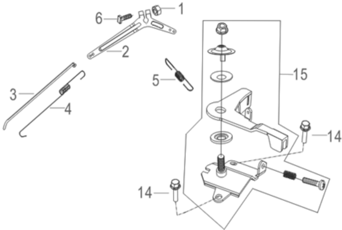
FIG.11 CONTROL ASSY, THROTTLE
