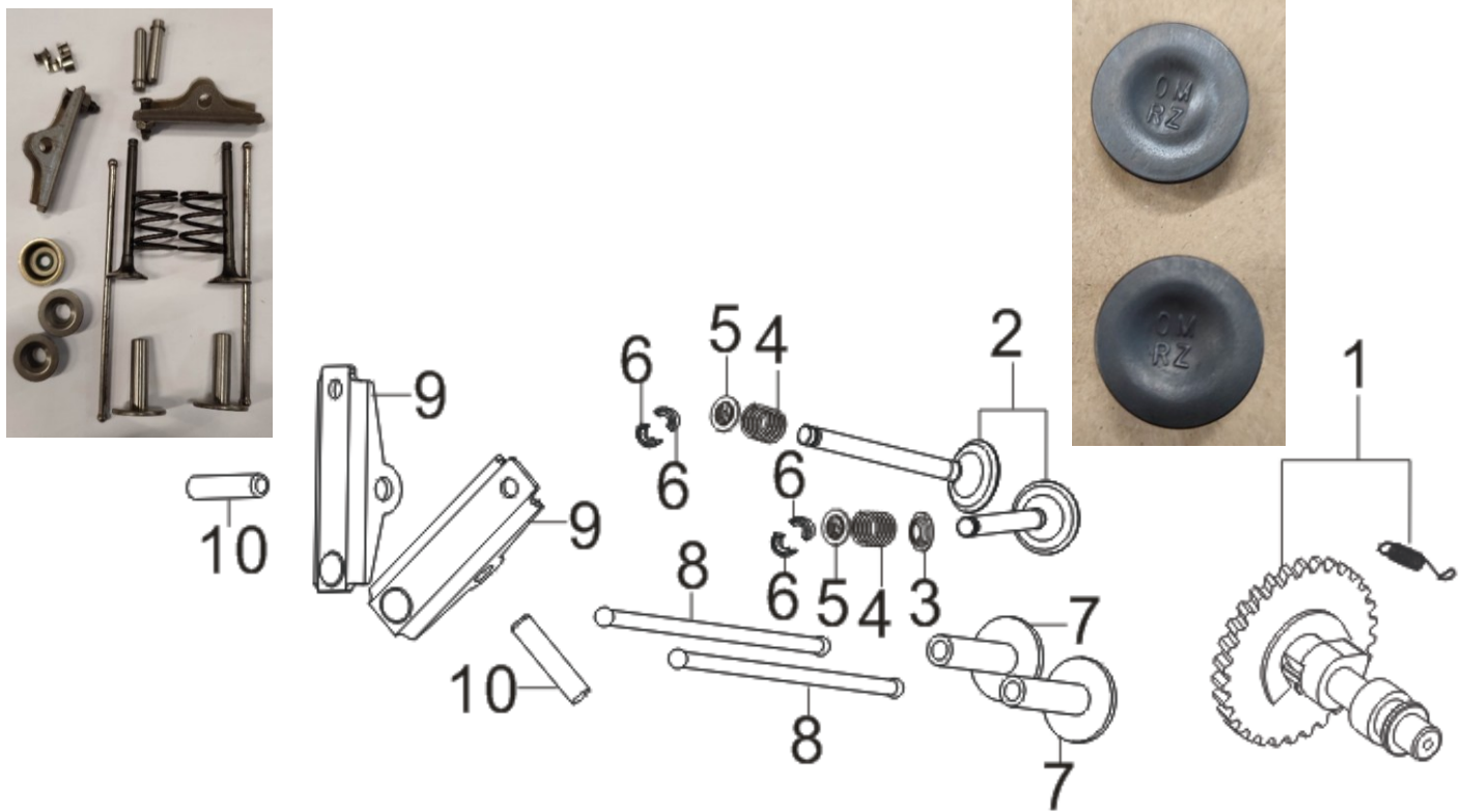
FIG.6 TRAIN, VALVE / CAMSHAFT SUBASSEMBLY
