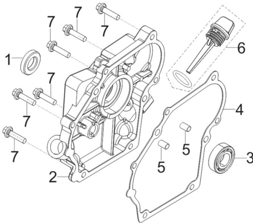
FIG.2 COVER SUBASSEMBLY, CRANKCASE
