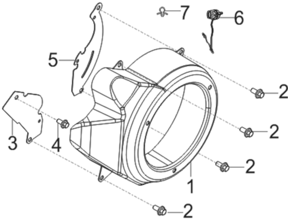
FIG.8 SHROUD / SHIELD,LOWER
