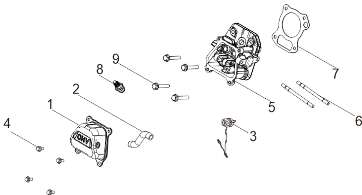
FIG.3 HEAD SUBASSEMBLY, CYLINDER / PLUG,SPARK (E03)
