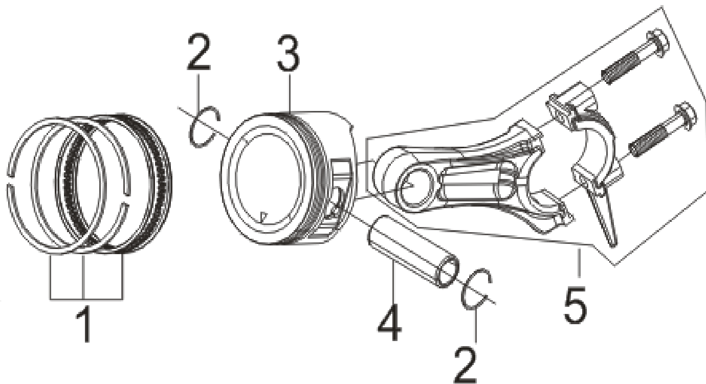
FIG.5 RING SET,OIL / ROD,CRANKSHAFT CONNETING (E05)
